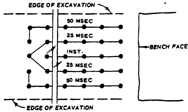
Fig. 5-12. Delays, in milliseconds, as shown (Du Pont ® )
