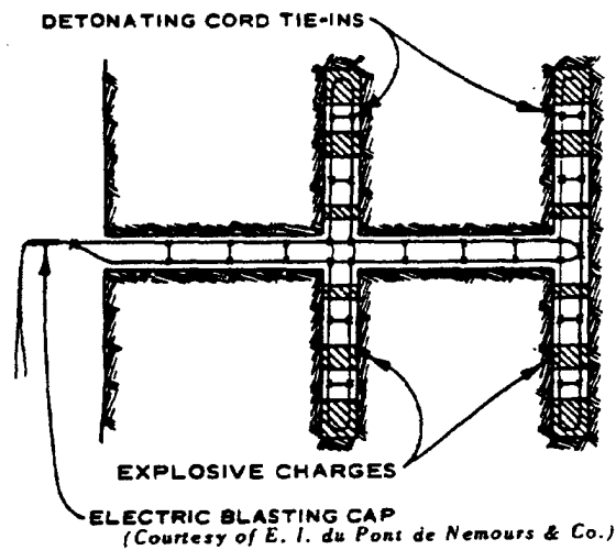
Fig. 5-15. Plan of coyote layout with detonating cord (after Du Pont 8 )
