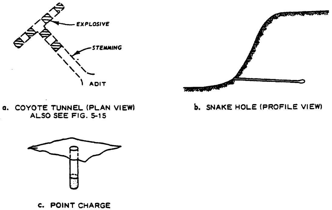
Fig. 5-3. Single-hole arrays
