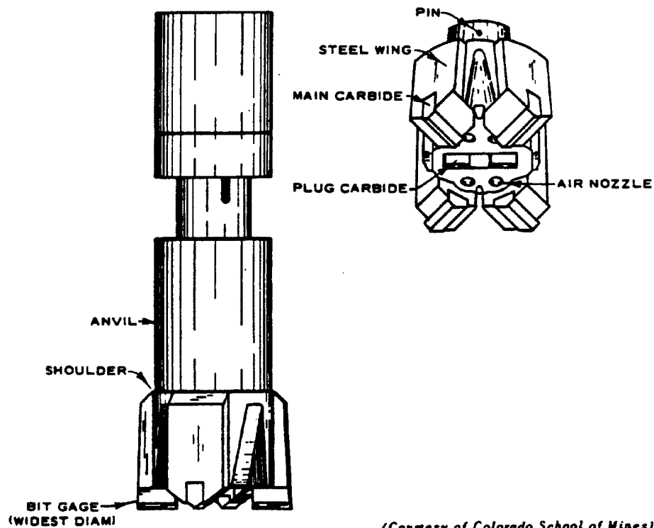
Fig. 4-14. Rotary-percussive drill bit (after Liljestrands 13 )
