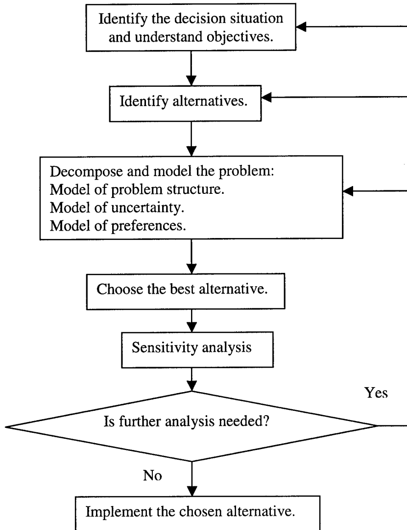
Figure 1. The Decision Analysis Process (after Clemen, 2001: 6).
