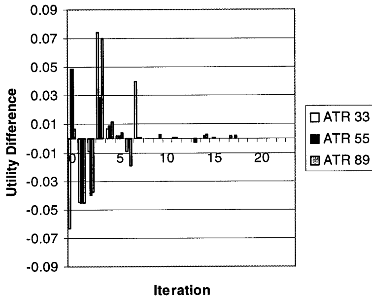
Figure 21. Hybrid Utility Model Difference Between Iteration and True Utility Model, CID Profile.
