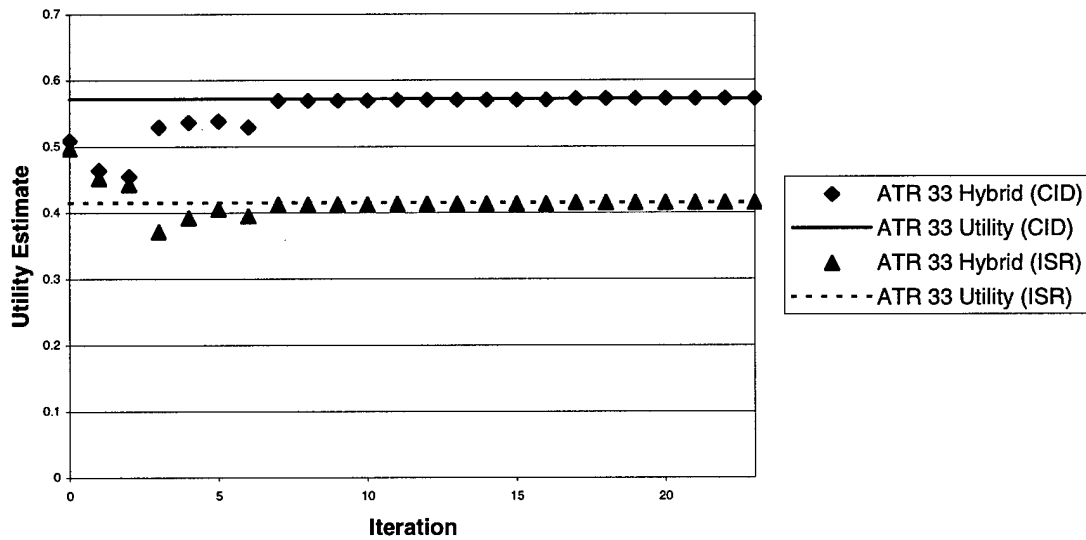
Figure 18. ATR Hybrid Utility Iterations for ATR 33.
