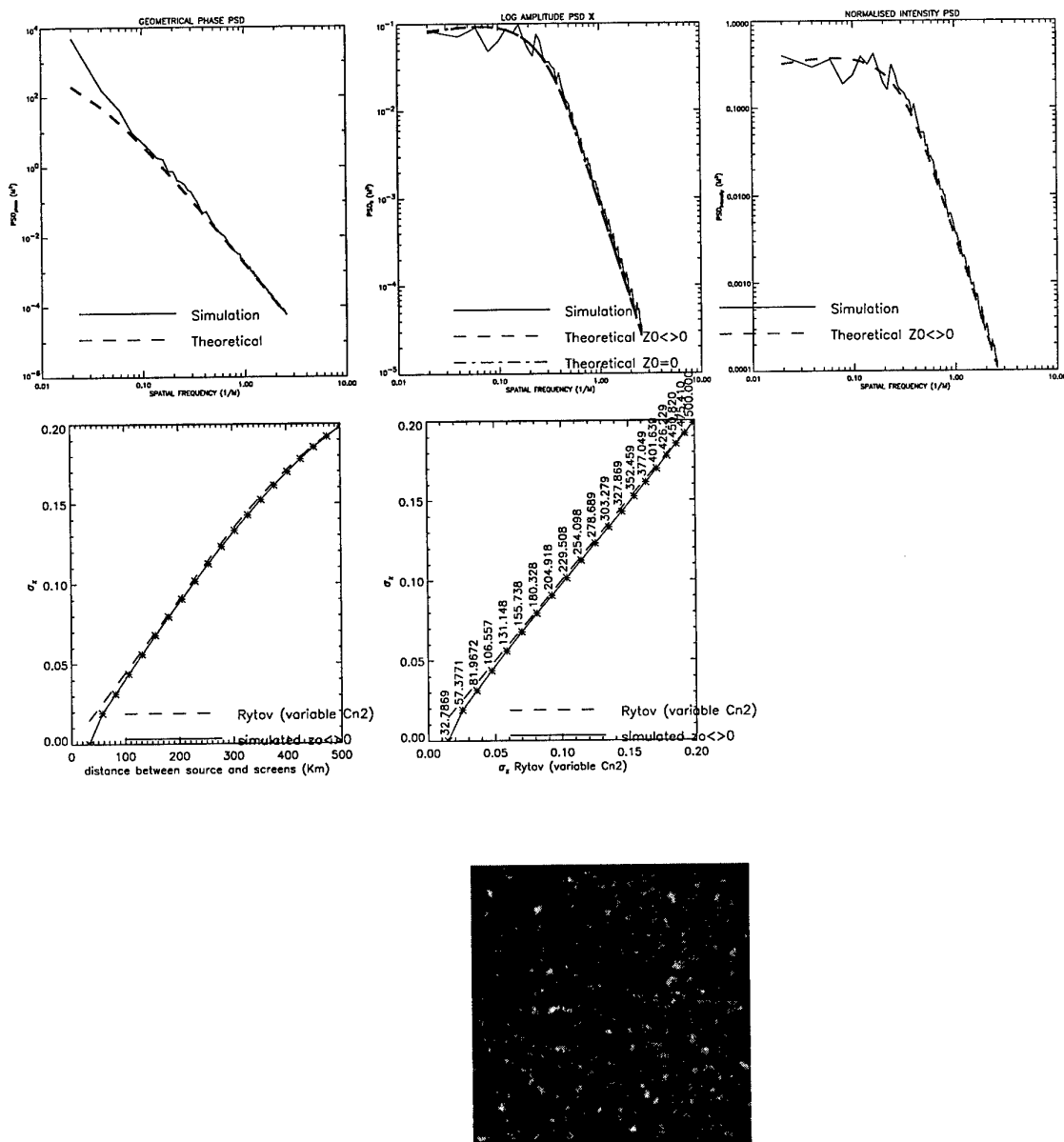
Figure 22: Result of the numerical experiment ( h_{\text{source}} = 15 \text{ km} , \lambda = 5.0 \mu\text{m} ).
