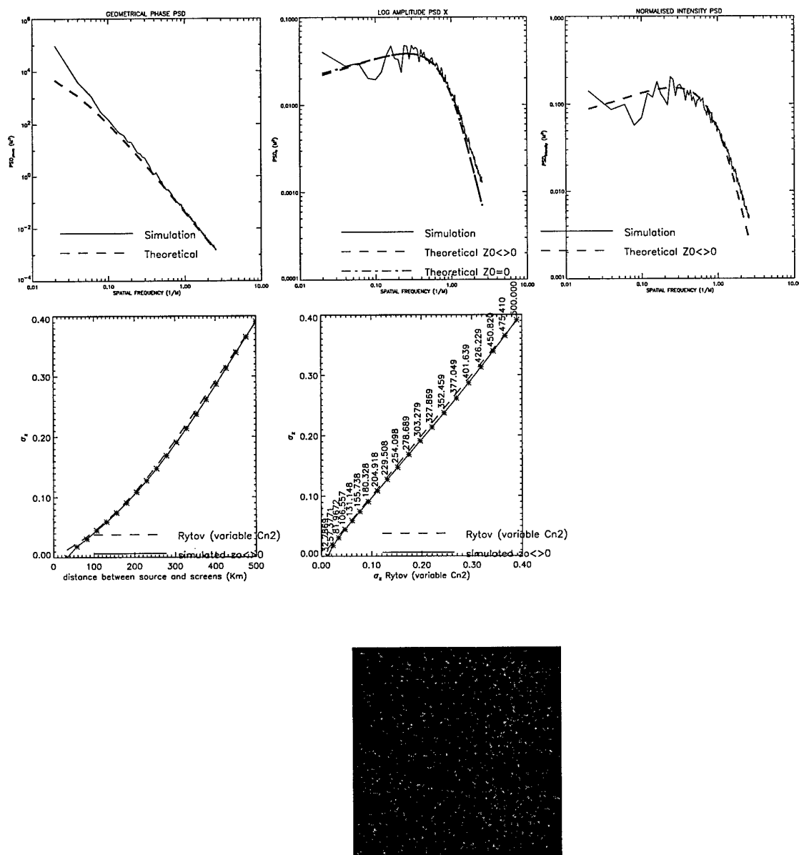
Figure 24 - Result of the numerical experiment ( h_{source} = 25 km, \lambda = 1.06 \mu m ).
