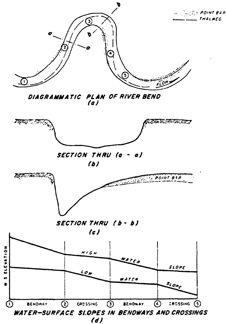
Figure 6-1. Characteristics of a river reach
