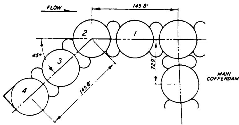
Figure 11-2. Cofferdam deflector
