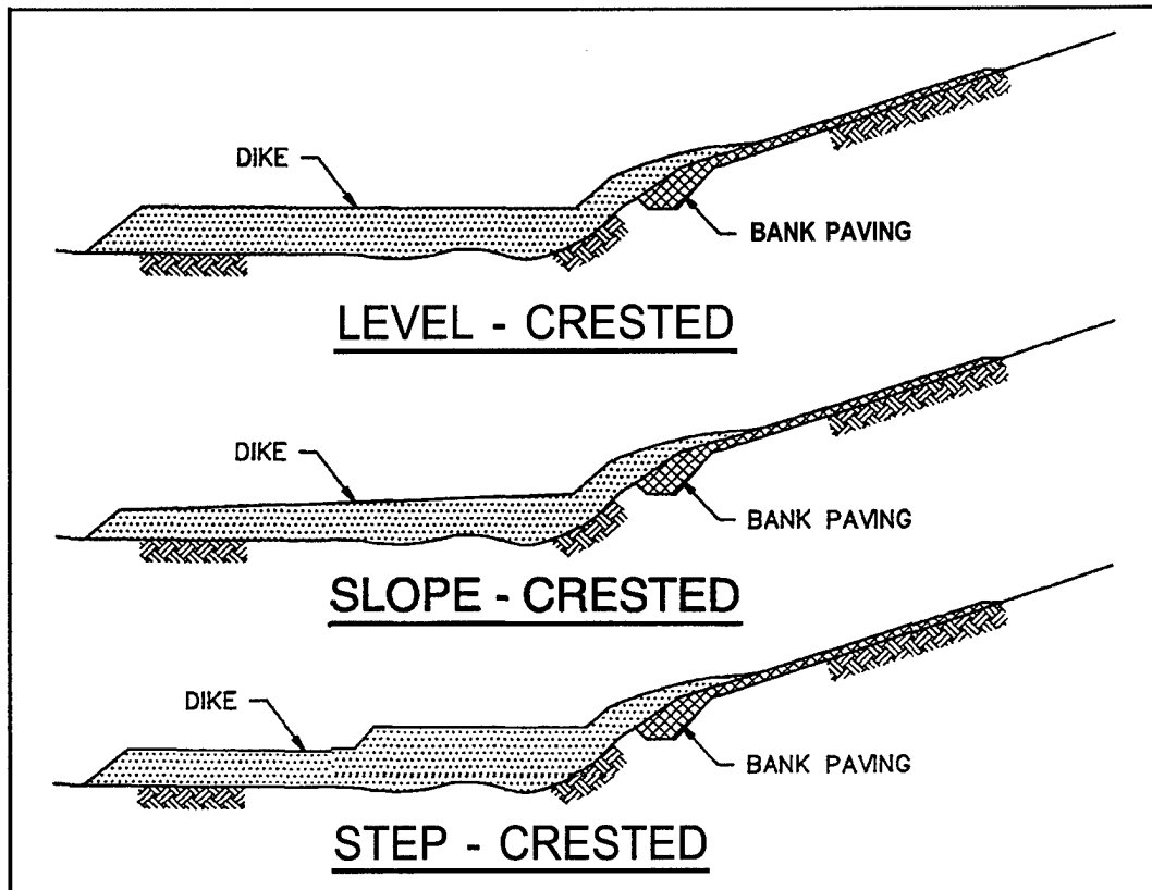
Figure 7-4. Stone spur dike crest profiles
