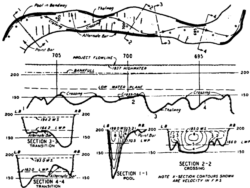
Figure 6-2. Features of a typical improved reach--Mississippi River
