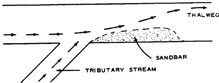
Figure 6-4. Effect of tributary on channel configuration
