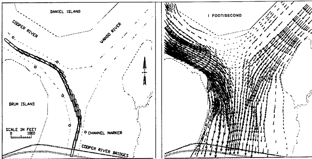
b. RMA2-WES hydrodynamic solution
