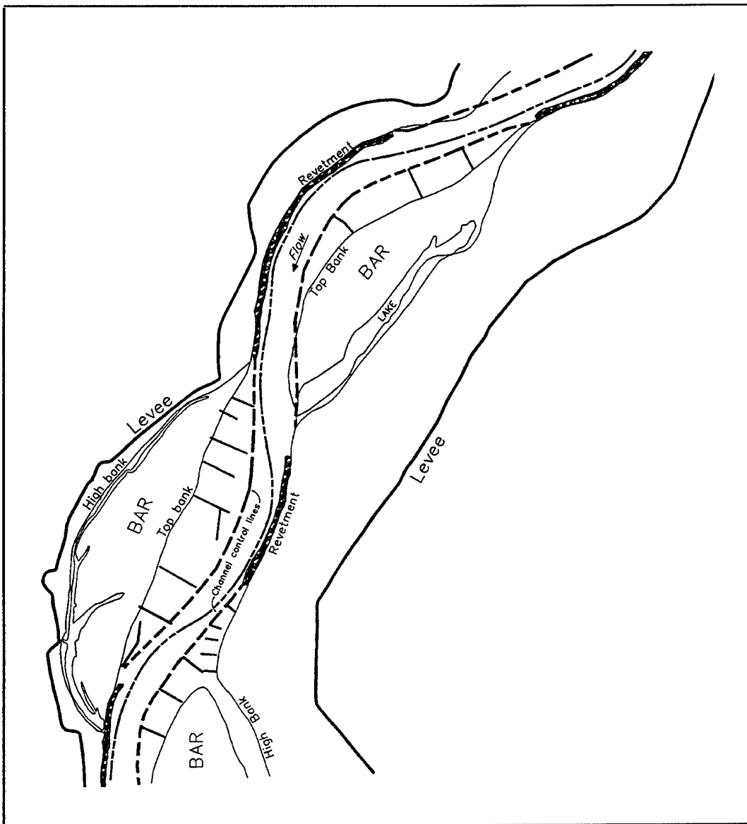
Figure 7-4. Example of layout for channel control lines
