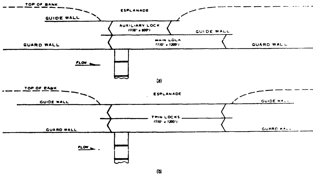
Figure 8-2. Arrangement with adjacent locks
