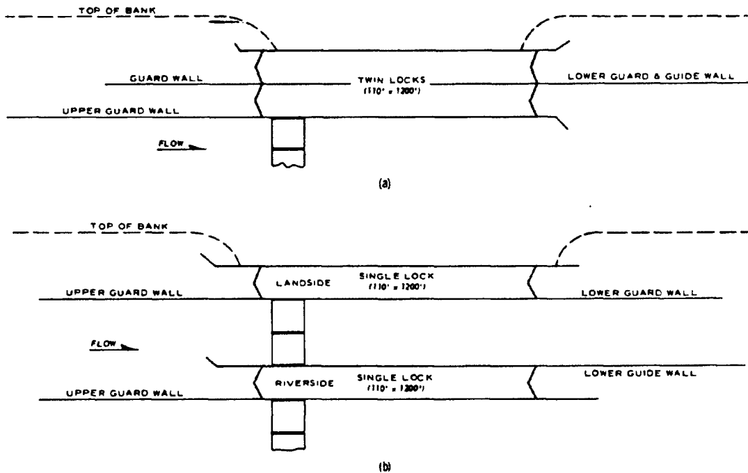
Figure 8-3. New concepts in lock arrangement
