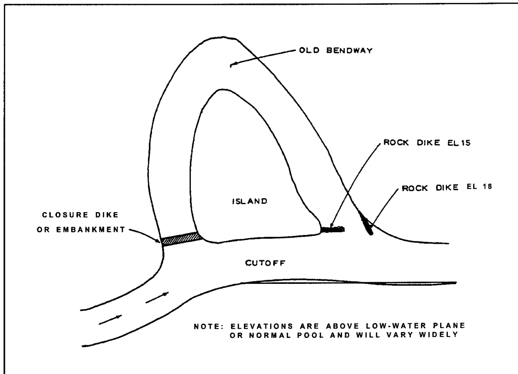
Figure 7-1. Cutoff-old bendway used for harbor or recreation
