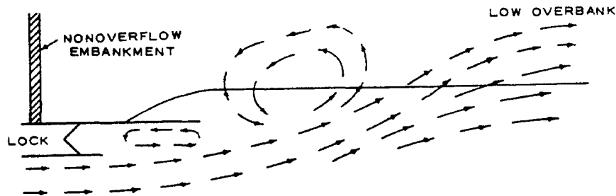
Figure 10-3. Low overbank adjacent to lock approach
