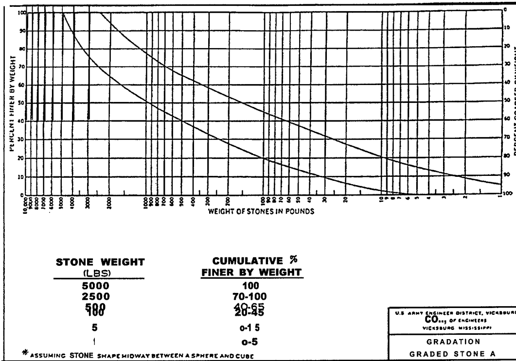
Figure 7-7. Quarry-run stone gradation curve
