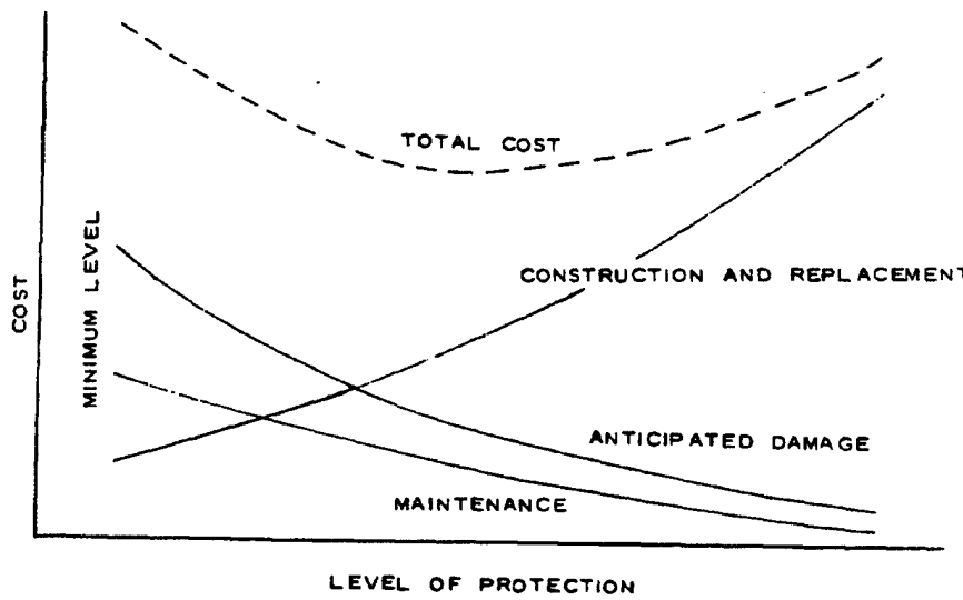
Figure 14-2. Project cost curves
