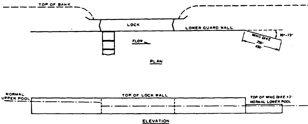
Figure 10-4. Wing dike used to minimize shoaling in lower lock approach
