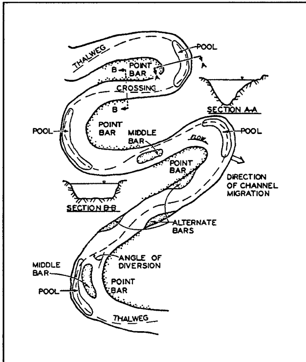
Figure 7-5. Channel planform
