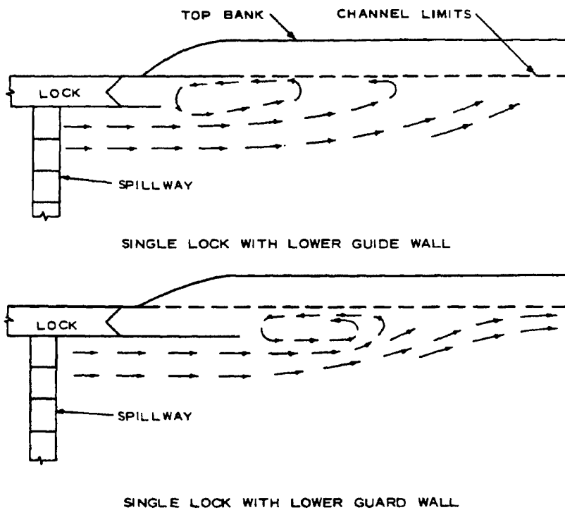
Figure 10-2. Currents in upper lock approach
