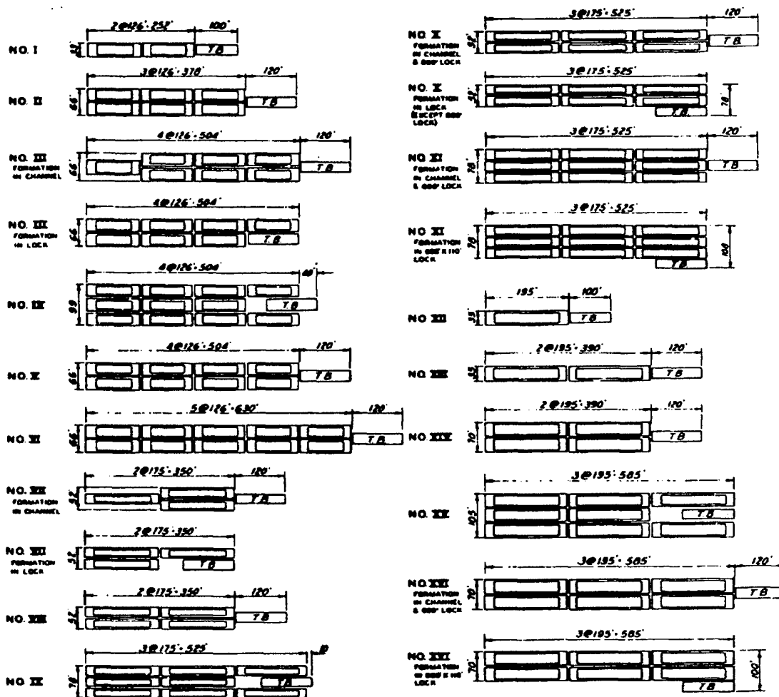
Figure 3-2. Typical arrangements for barge tows
