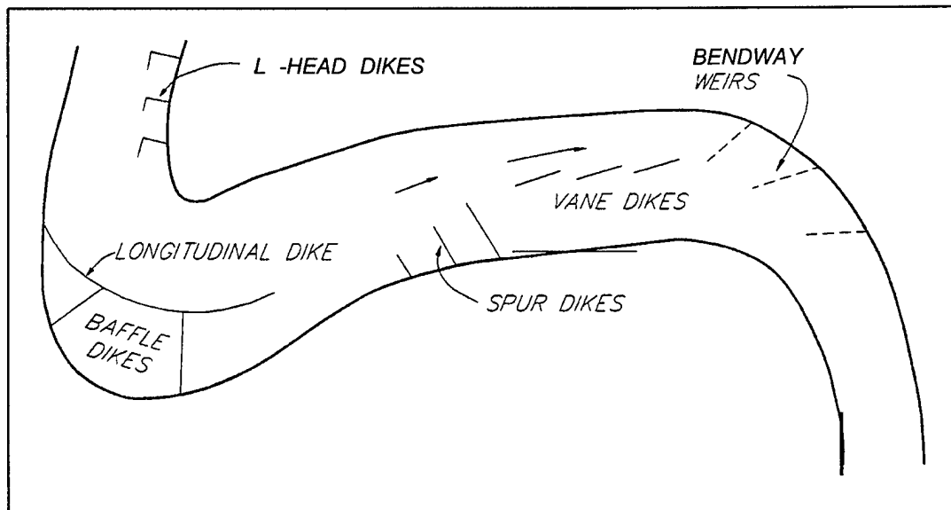
Figure 7-2. Types of training structures in use
