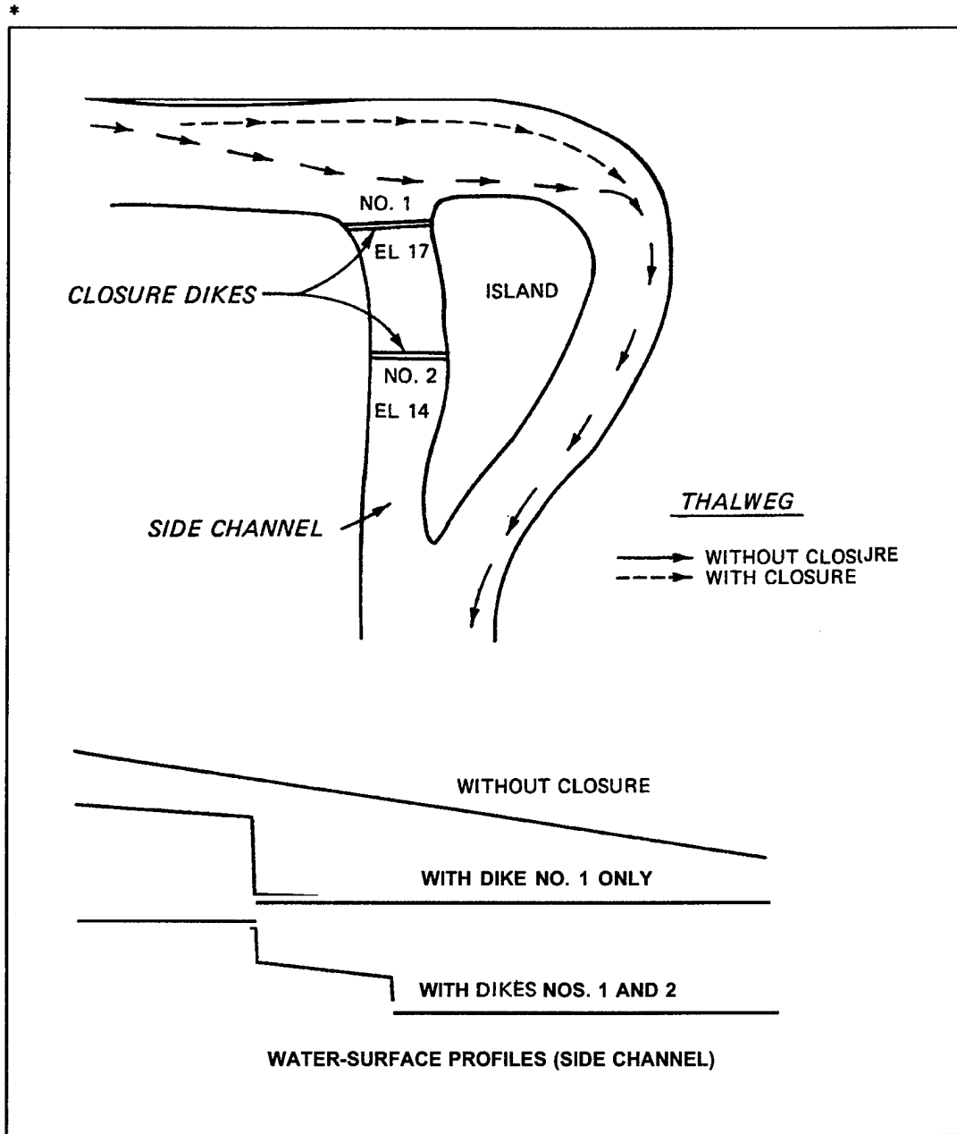
Figure 7-12. Side channel closure
