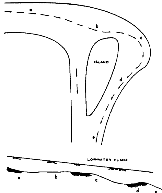
Figure 6-3. Typical divided channel
