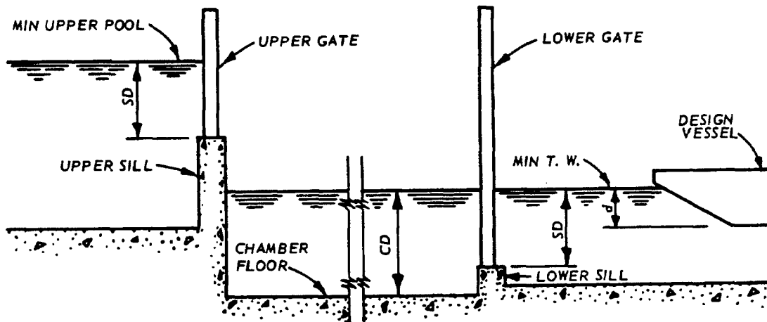
Figure 8-8. Lock longitudinal profile
