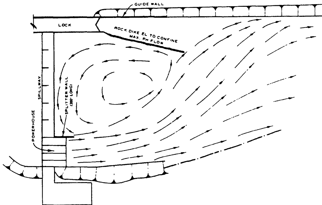
Figure 10-6. Dike used to minimize effect of powerhouse releases on navigation in lower lock approach
