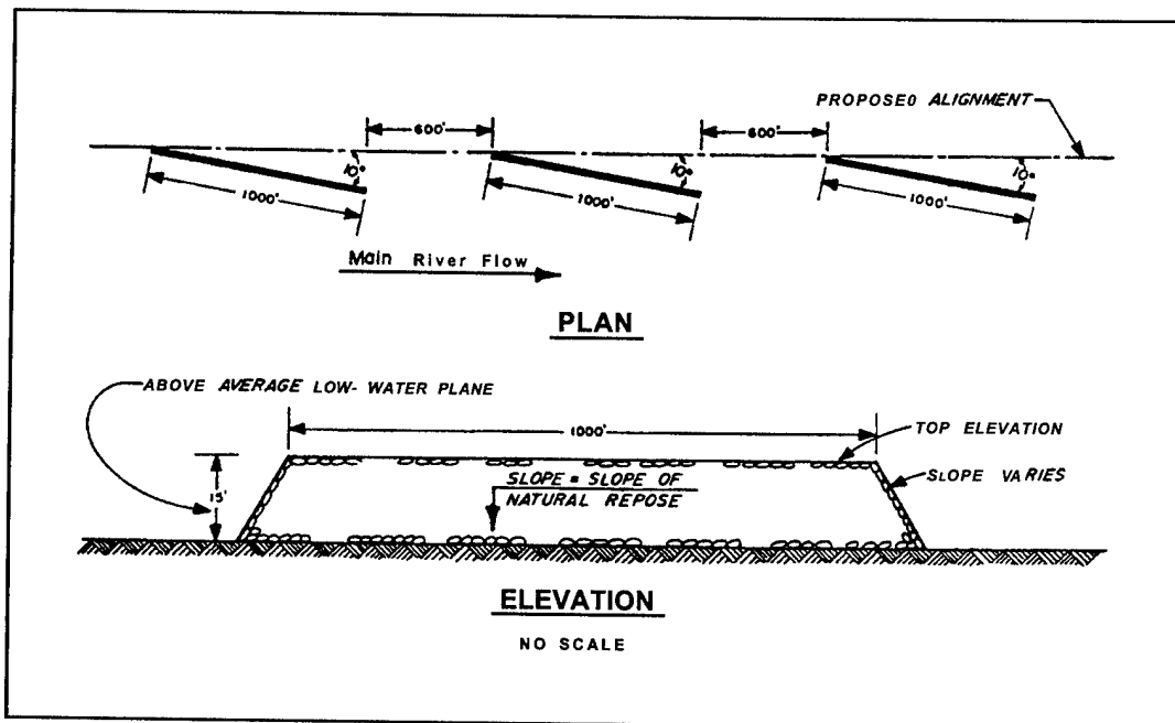
Figure 7-9. Vane dike layout
