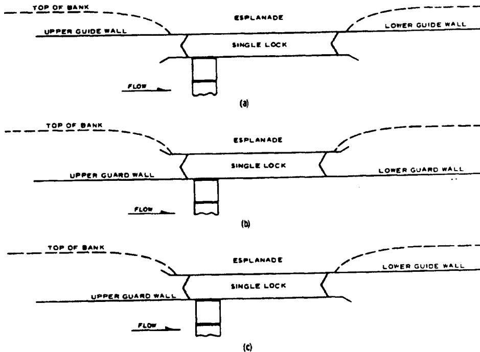
Figure 8-1. Arrangement for single lock
