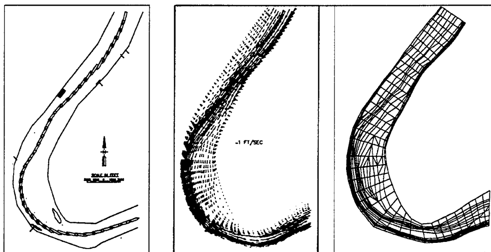
a. WES tow simulator track plots b. RMA2-WES hydrodynamic solution c. Numerical model computational mesh
