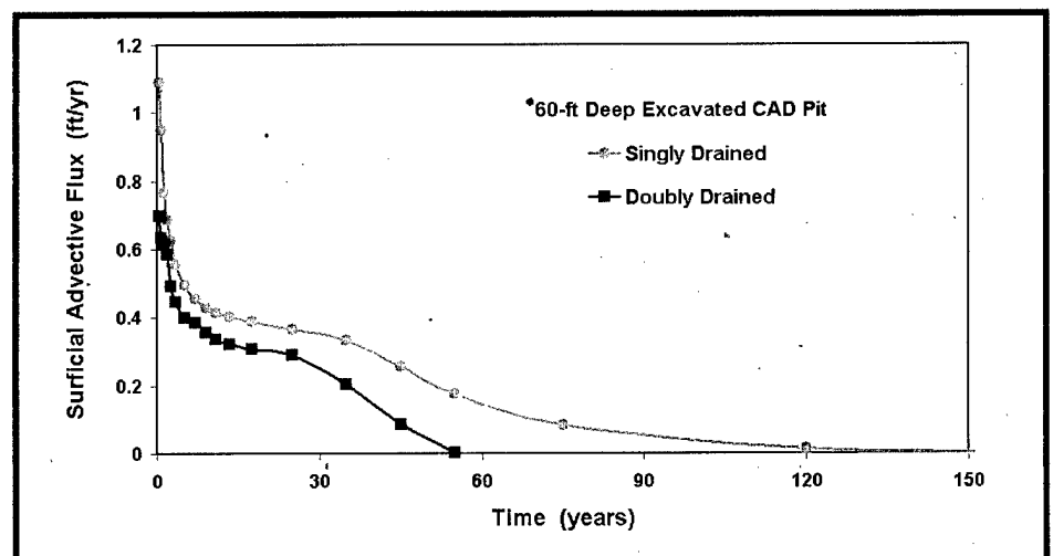
Figure 3. Water flux predictions for 60-ft deep CAD pit
