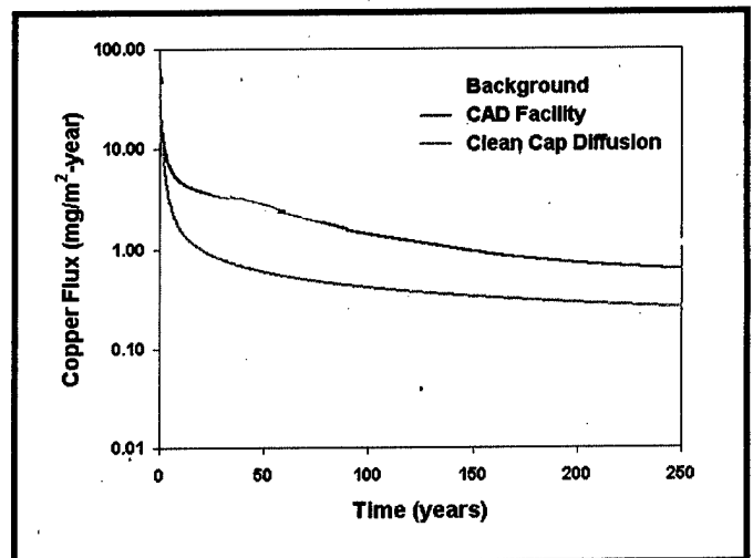
Figure 5. Total copper flux to the water column from surficial sediments
