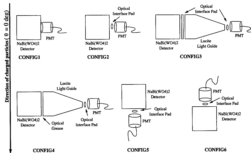
Figure 11: Various setup configurations used when taking data with NaBi(WO_4)_2 . The optical interface pads are transparent and made from a GE Silicone/RTV-615.
