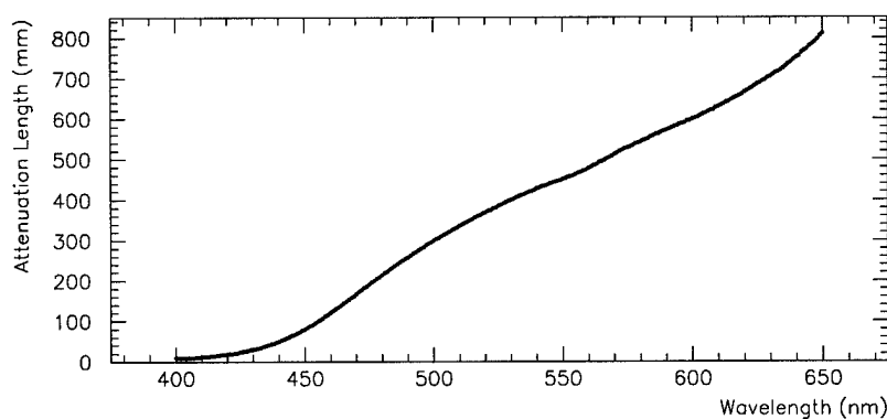
Figure 8: The attenuation length for photons in NaBi(WO_4)_2 as a function of wavelength measured using the Cary 5E Spectrophotometer.
