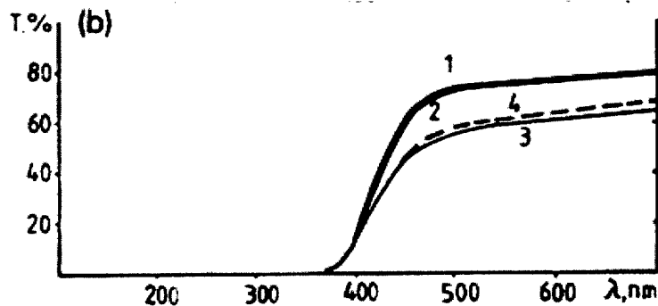
Figure 9: Per cent transmission ( 100 \cdot T_A ) for NaBi(WO_4)_2 with thickness of 10 mm. Each curve corresponds to the following conditions, 1: before irradiation, 2: after dose of 10^7 rad, 3: after dose of 10^8 rad, and 4: 50 days of recovery [2].
