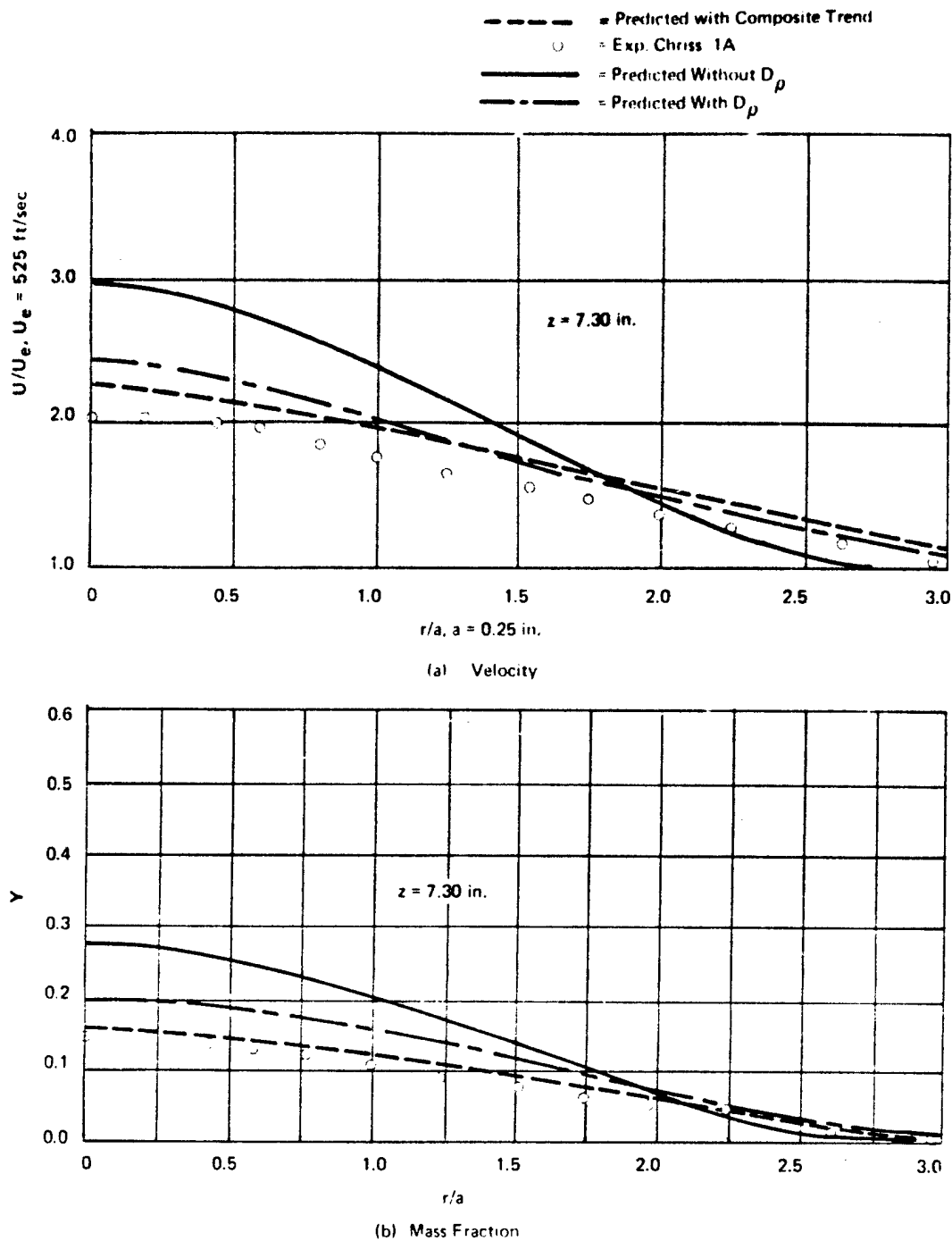
Figure 19. Effect of D_p on Predicted Mean Velocity and Hydrogen Mass Fraction Profile at z = 7.30 Inches. Se_T = 0.9 , Le_T = 1.0 . Data of Case 1A, Chriss, Ref. 6. Calculations started at z = 3.48 in.
