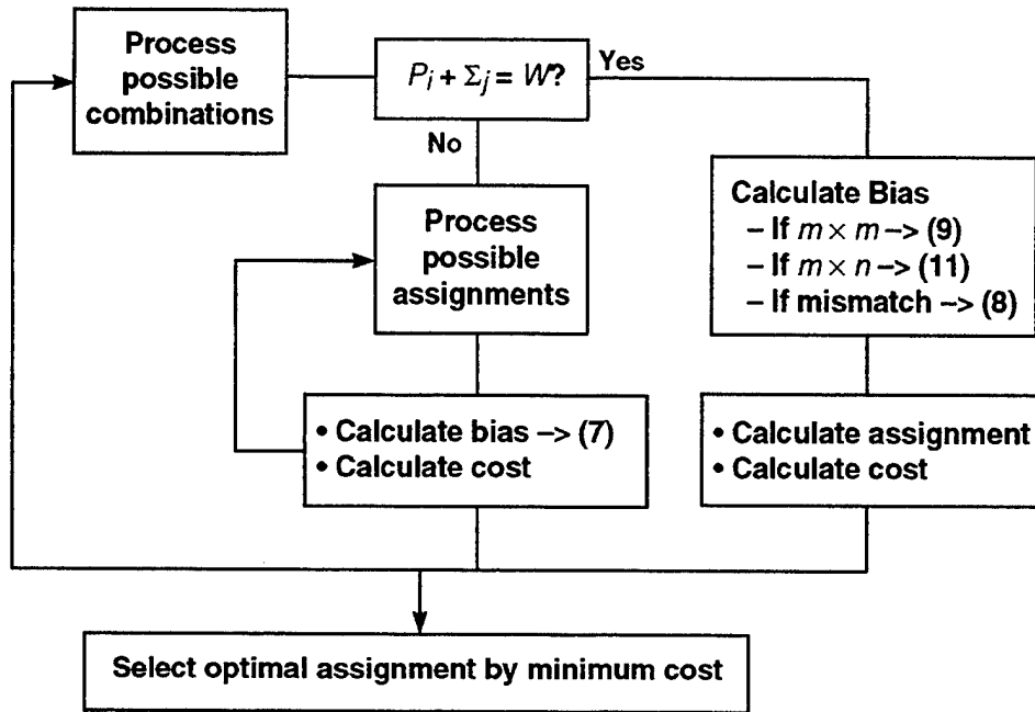
Figure 11. Flowchart of algorithms for cases.
