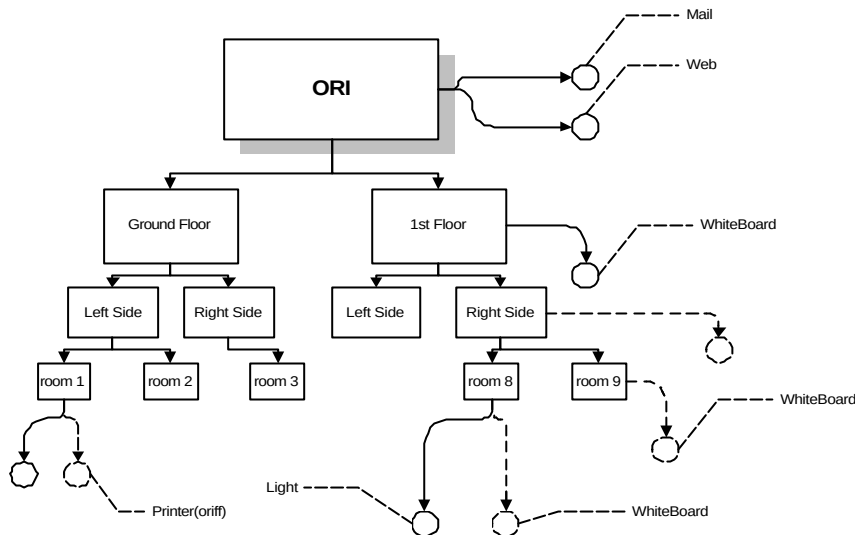
Fig. 7. Zone tree
