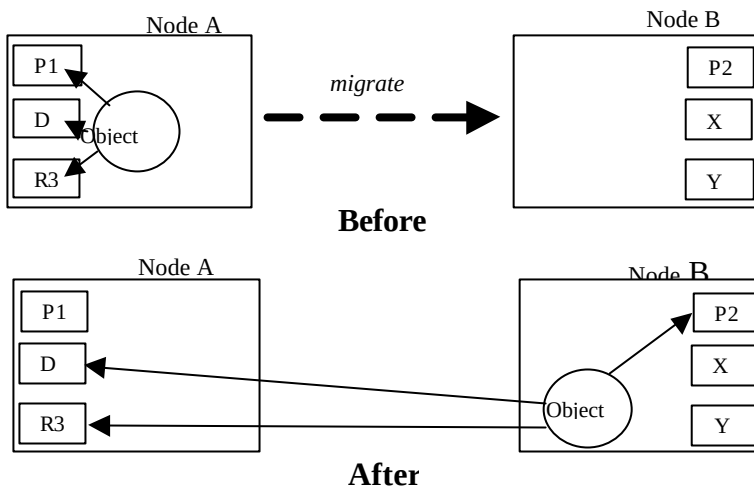
Fig. 3. Architectural Pointers
