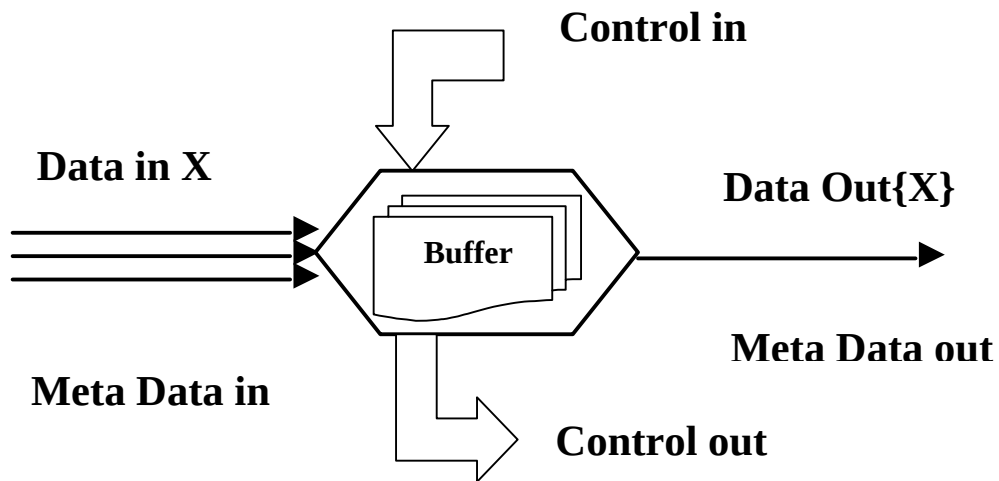
Figure 3. History contextor
