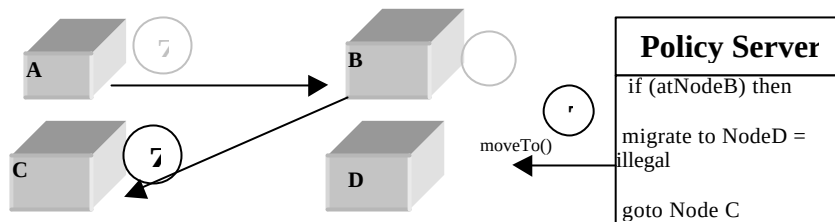
Fig. 2. Migration Technique
