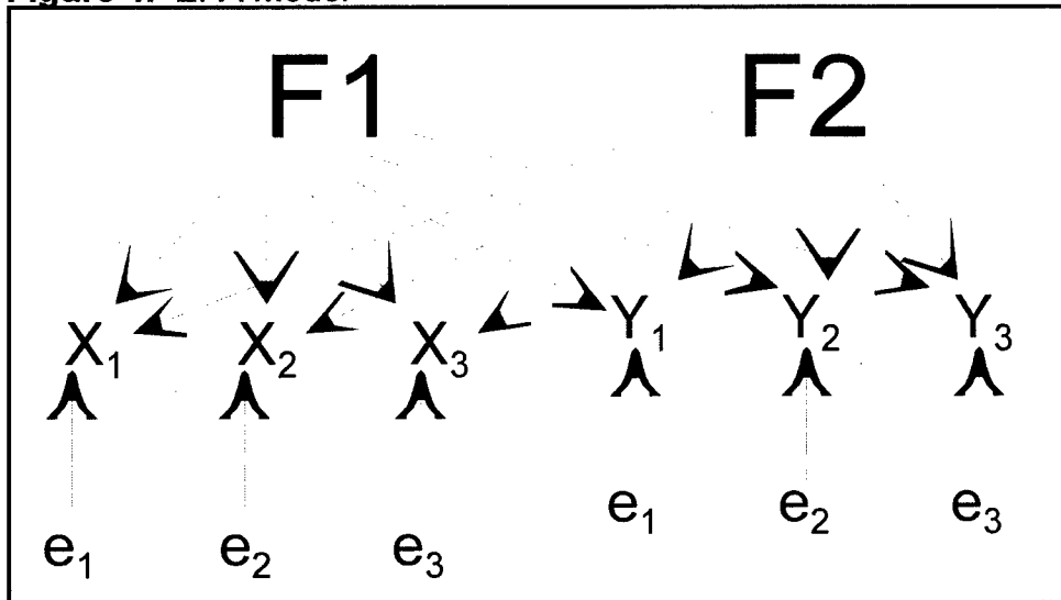
Figure 4. EFA Model
