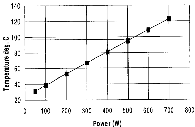
Fig. 2. Thermal simulation results for a forced convection three-phase inverter module. The data are based on junction temperatures as a function of the thermal loss in the module.
