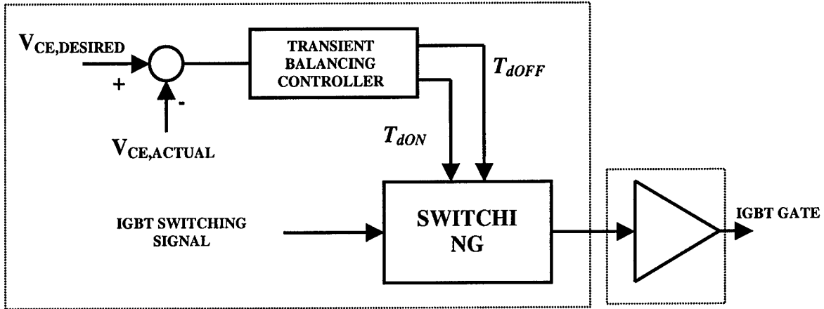
Fig. 7 Transient voltage balancing controller for one IGBT of “ n ” series-connected IGBT.
