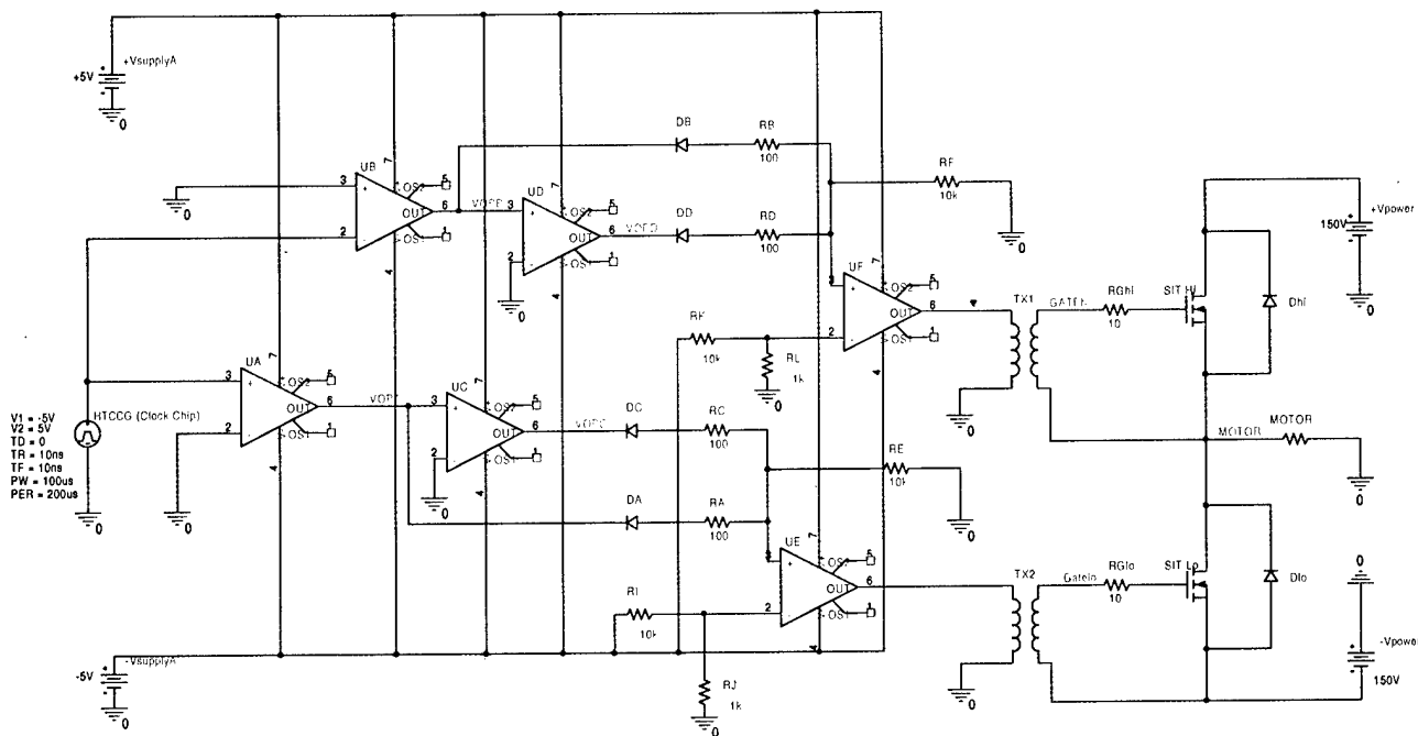
Fig. 14. Novel high-temperature half-bridge design.
