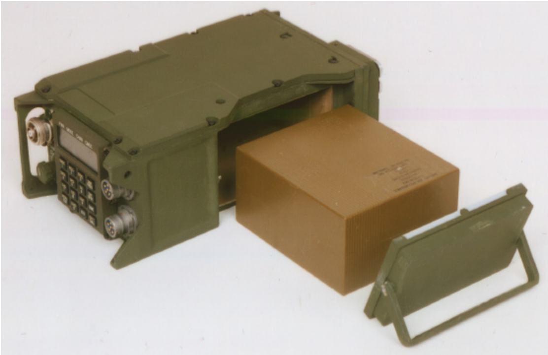
ASIP Radio with Battery Cover Open and Battery Exposed
