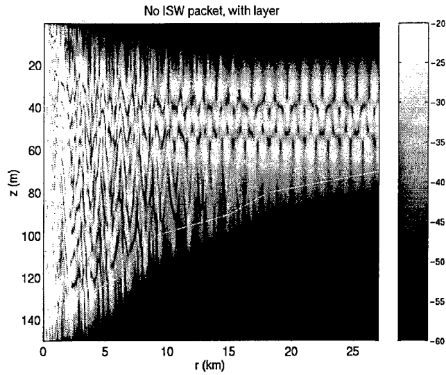
Figure 5. Despread level is shown for the Case 3 PE simulation. The water column has no ISW packet. The warm near-bottom layer is included. Levels are increased over Cases 1 and 2.
