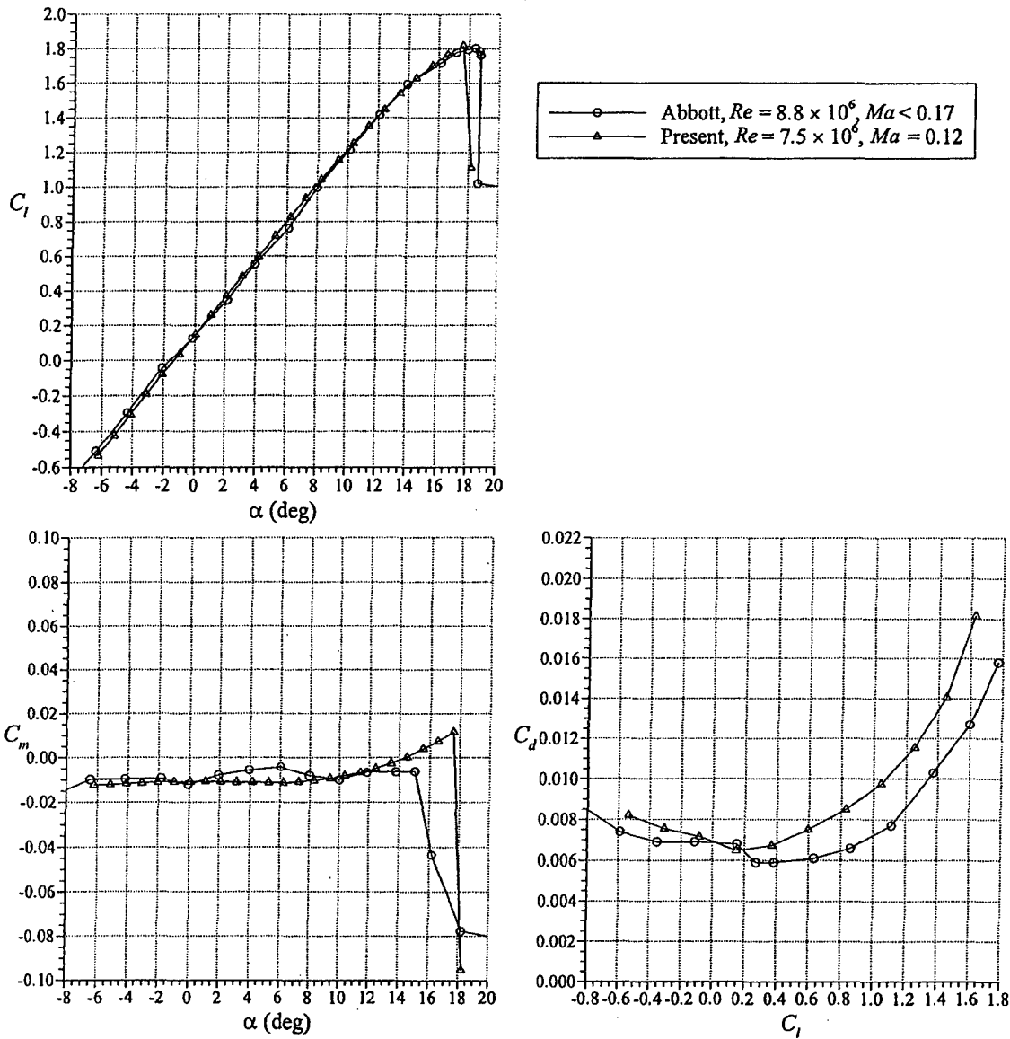
FIGURE 16. COMPARISON OF THE CLEAN NACA 23012 AIRFOIL PERFORMANCE AT Re = 7.5 \times 10^6 WITH HISTORICAL DATA FROM ABBOTT AND VON DOENHOFF AT Re = 8.8 \times 10^6
