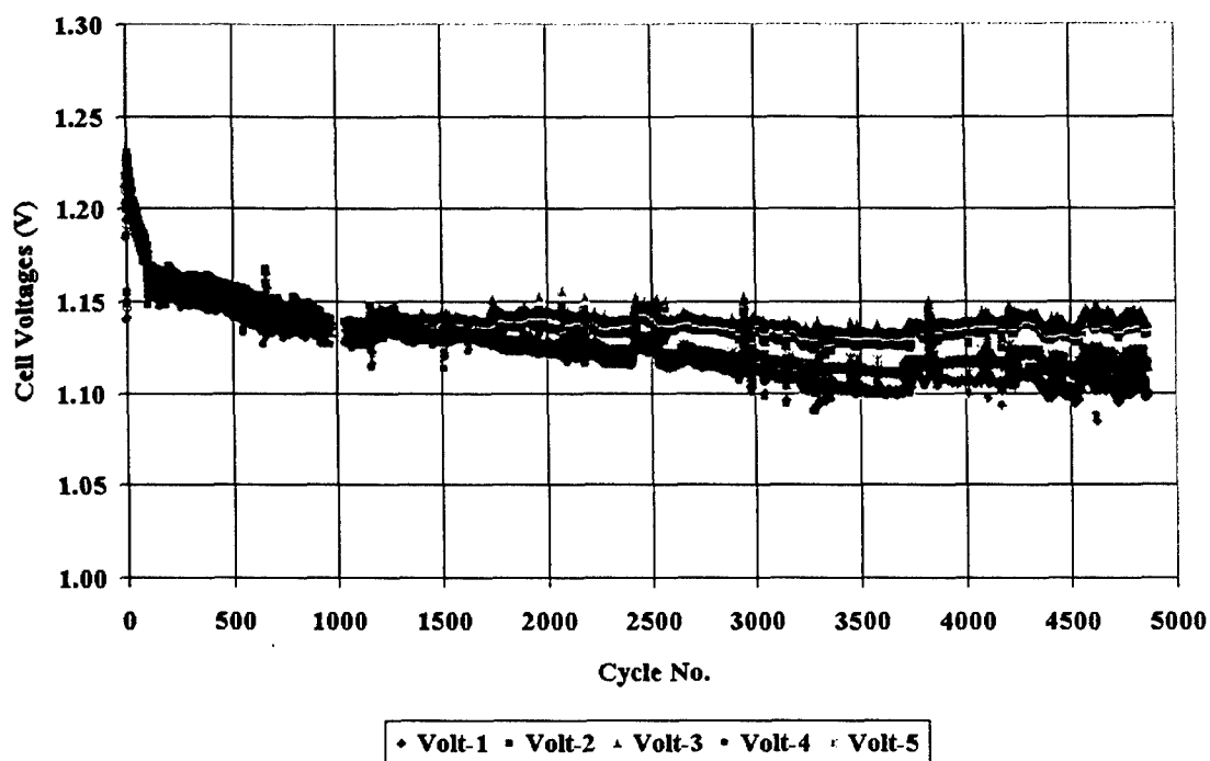
Figure 2. Cell EOD voltages vs. cycle for E007D.
