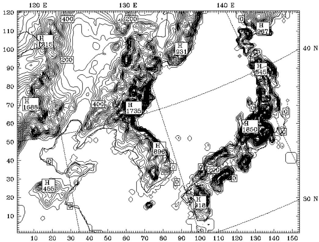
Figure 5. Terrain map of the MM5 inner nest used in this study. Elevations are contoured every 50 meters.
