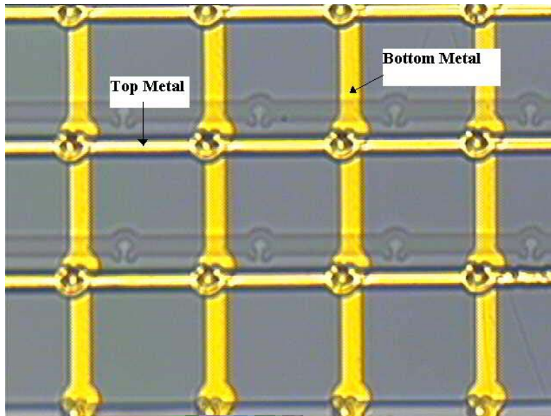
Figure 65 Microscope image (30x) illustrating the matrix array. The shadow shows the misalignment and subsequent recess of the PMGI. The top layer metallization is 1.4\text{ }\mu\text{m} higher than the bottom layer metallization.
