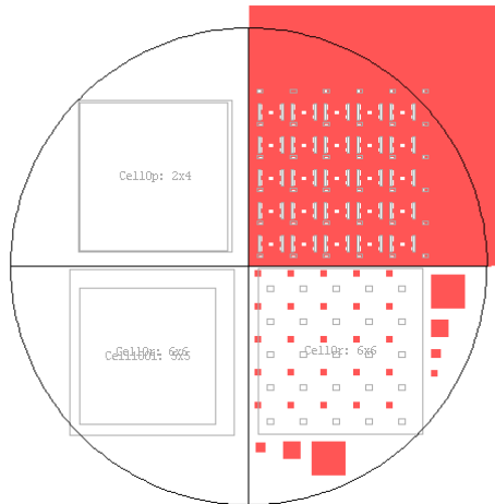
Figure 20 L-Edit layout of photomask 2.
