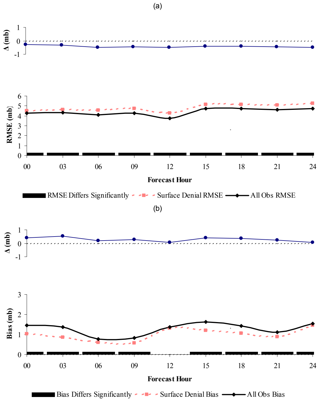
Figure 33. 12Z initialization mean sea level pressure verification results (SFC). The graphs of \Delta represent the average differences (C1-SFC). Chart (a) depicts the average RMSE and chart (b) is the average bias.
