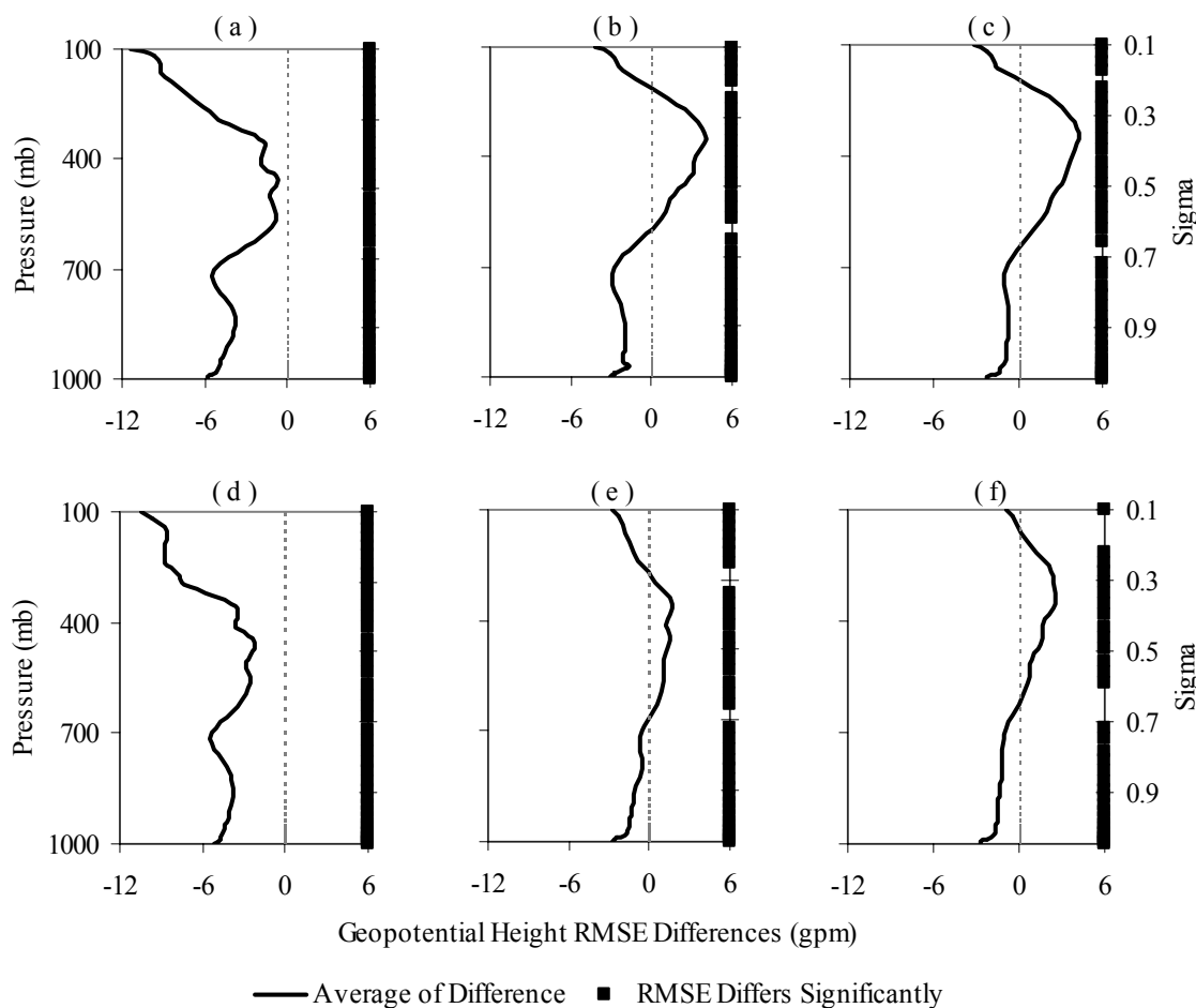
Figure 17. Average differences (C1-TOT) in geopotential height RMSE. Charts (a), (b), and (c) represent the 0-hr, 12-hr, and 24-hr forecasts respectively for the 00Z initialization time. Charts (d), (e), and (f) represent the 0-hr, 12-hr, and 24-hr forecasts respectively for the 12Z initialization time. The black bar denotes sigma levels with a statistically significant difference at the 95% significance level.
