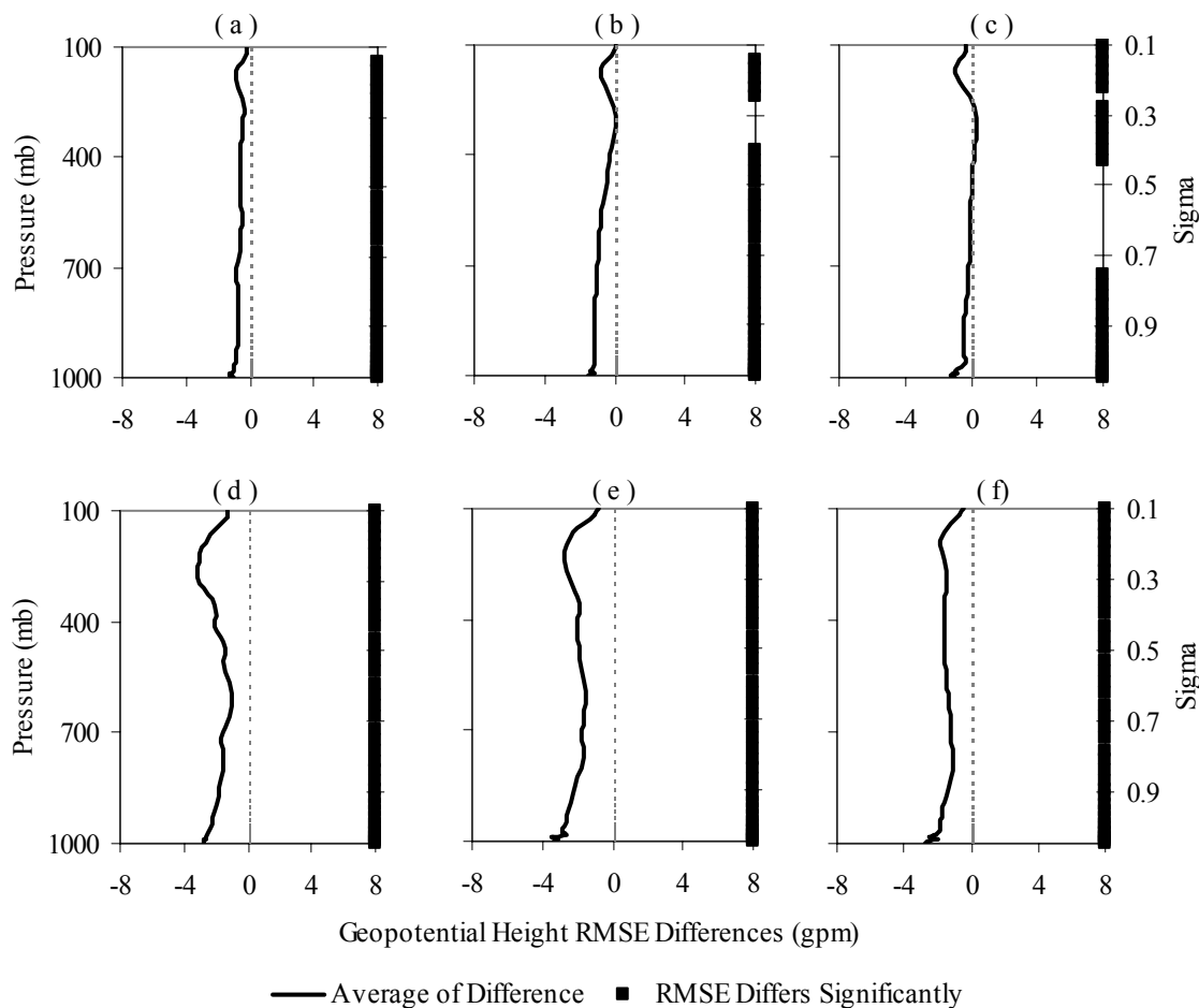
Figure 19. Average differences (C1-SFC) in geopotential height RMSE. Same as Figure 17.
