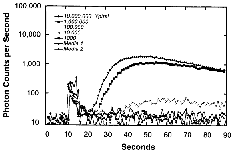
Figure 4-3. Response of Yp-specific cells charged with coelenterazine prior to freezing, with four days post-thaw. The same cells as those used in Figure 4-2 were assayed after incubation for four days at room temperature using 50 µl of killed Yp diluted to the indicated concentrations in CO 2 -I media.
