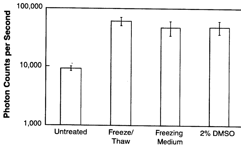
Figure 4-1. Effects of cell treatments on the response of Yersinia pestis ( Yp ) specific B cells to killed Yp . Cells were challenged with 50 \mu l of 10,000,000 Yp /ml diluted in CO 2 -I after various cell treatments. Untreated: Cells were grown in RPMI, loaded with coelenterazine, washed, recovered for 24 h, and challenged with Yp . Freeze/thaw: Cells were grown in RPMI, transferred to freezing medium, and frozen. Thawed cells (1 ml) were placed into 4 ml of RPMI and incubated at 37°C for 24 h, loaded with coelenterazine, washed, recovered for 24 h, and challenged. Freezing medium: Cells were grown in RPMI, transferred to freezing medium and incubated at room temperature for 10 min. Cells (1 ml) were placed into 4 ml of RPMI and incubated at 37°C for 24 h, loaded with coelenterazine, washed, recovered for 24 h, and challenged. 2% DMSO: Cells were grown in RPMI, transferred to RPMI containing 2% DMSO and incubated at 37°C for 24 h, loaded with coelenterazine, washed, recovered for 24 h, and challenged.
