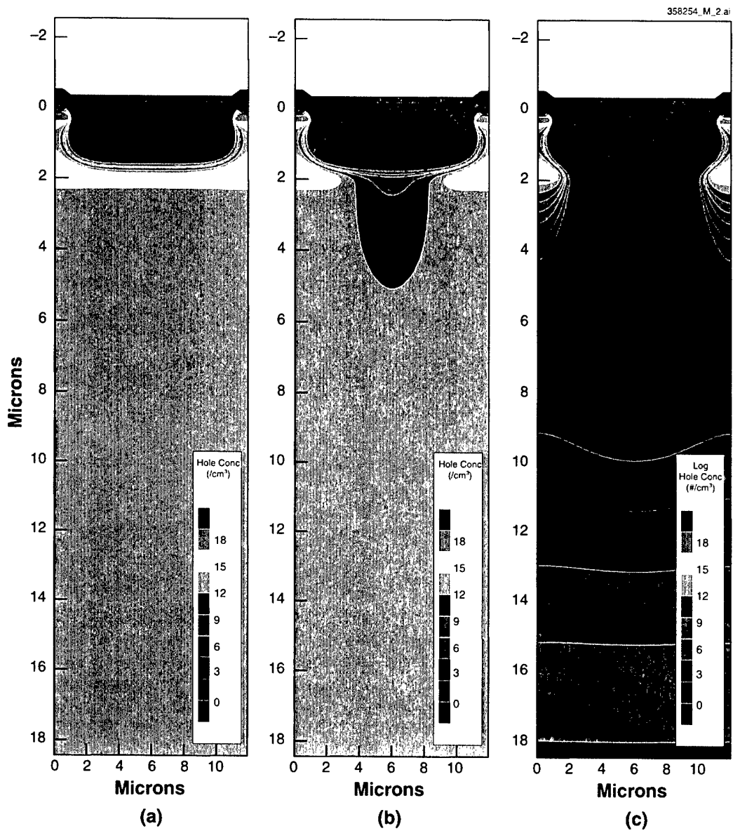
Figure 5-1. Simulated hole concentration contours obtained for electronically shuttered device with gate electrode applied bias of (a) 4, (b) 7, and (c) 12 V.
