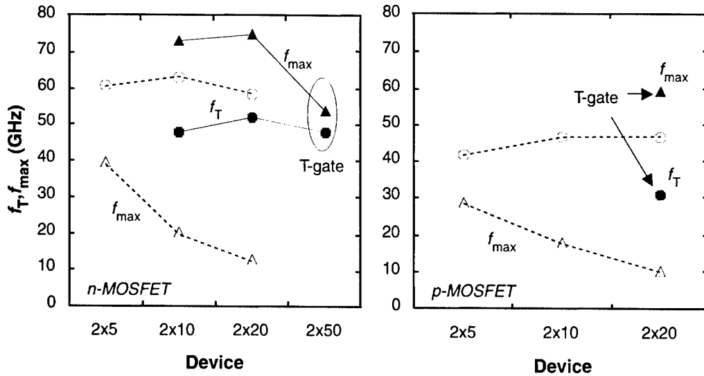
Figure 7-3. Measured f_T and f_{max} of n- and p-MOSFETs with various gate finger widths. The first digit refers to two gate fingers, and the second digit refers to finger width in micrometers. The drain and gate bias are 1.5 and 1.0 V, respectively. The dashed lines are devices without the Al overlay.
