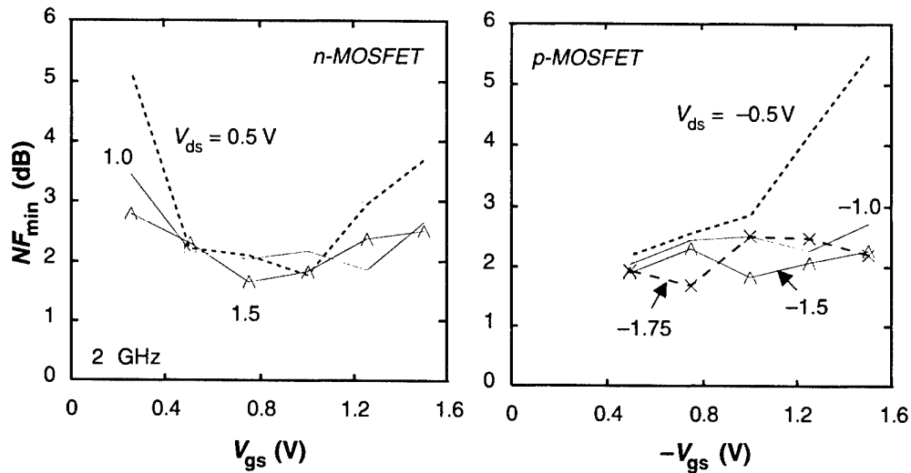
Figure 7-4. Measured NF_{min} of T-gate n- and p-MOSFETs with two 20- \mu m-wide gate fingers as a function of biases.
