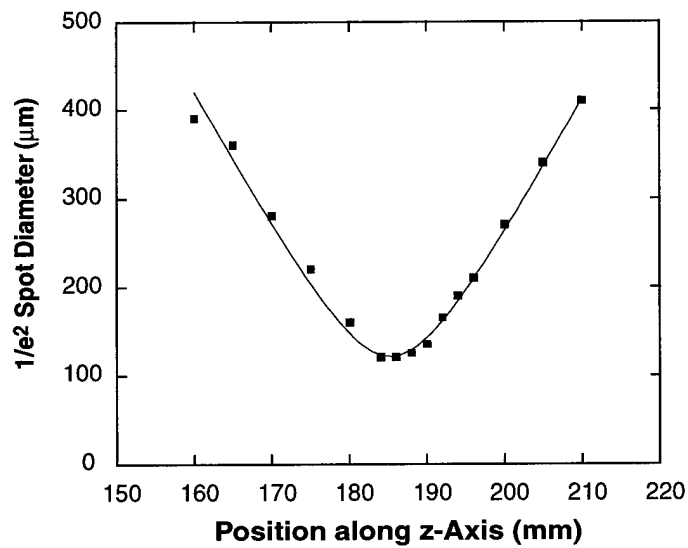
Figure 1-4. Dispersion-plane beam profile of four combined laser elements using a gold-coated grating on a Zerodur substrate. Combined power on the grating is 5.5 W with a curve-fit M² value of 1.40.
