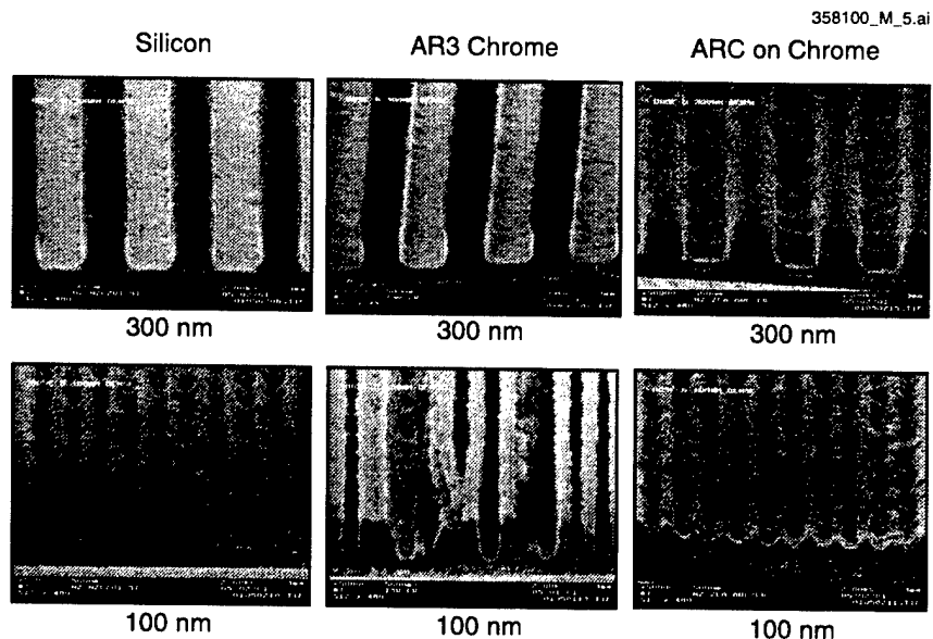
Figure 3-5. Imaging of 100- and 300-nm dense lines at 6.6 \mu\text{C}/\text{cm}^2 on ZCA-201 on silicon, AR3 chrome, and organic ARC on AR3. Substrate sensitivity, manifest as incomplete development, on AR3 chrome and ARC, is not present on silicon.
