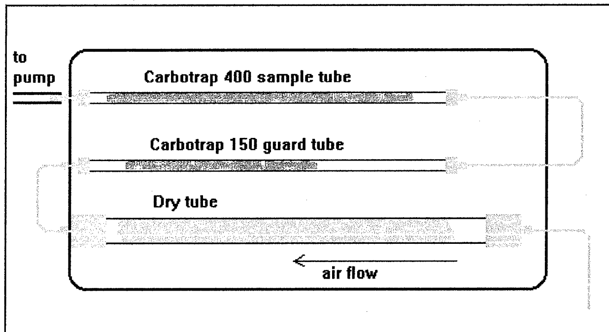
Figure 4.2.0 Schematic diagram of the 1999, multi-bed JAG box sampling train. Inlet is at lower right via copper tubes from the hive. The sample air is drawn through an anhydrous sodium sulfate drying tube, a Carbotrap 150 guard tube and a Carbotrap 400 sampling tube. The air sampling pump is attached via Tygon tubing to the JAG box outlet at the upper left.
