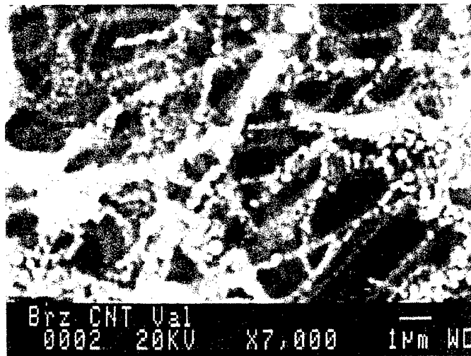
Figure 1. Scanning electron micrograph of braided single-walled carbon nanotubes on an iron substrate.
