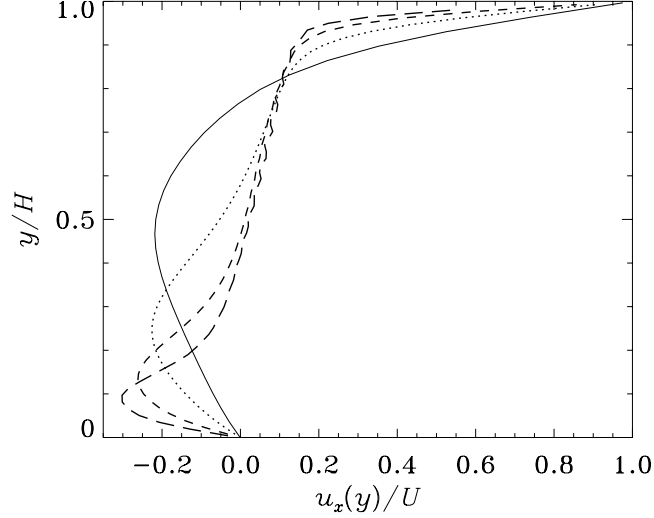
FIG. 7. 3-D lid-driven cavity flow. Effect of Reynolds number \text{Re} on the normalized horizontal velocity profiles u_x(x, y, z)/U at x/H = z/H = 0.5 . The results are obtained by using D3Q19 LBE model with U = 0.1 , \text{Re} = 100 , N_x \times N_y \times N_z = 33^3 , \Delta = 0.5 (solid line); U = 0.1 , \text{Re} = 400 , N_x \times N_y \times N_z = 67^3 , \Delta = 0.5 (dotted line); U = 0.1 , \text{Re} = 1000 , N_x \times N_y \times N_z = 67^3 , \Delta = 0.5 (dashed line); and U = 0.1 , \text{Re} = 2000 , N_x \times N_y \times N_z = 67^3 , \Delta = 0.25 (long dashed line).
