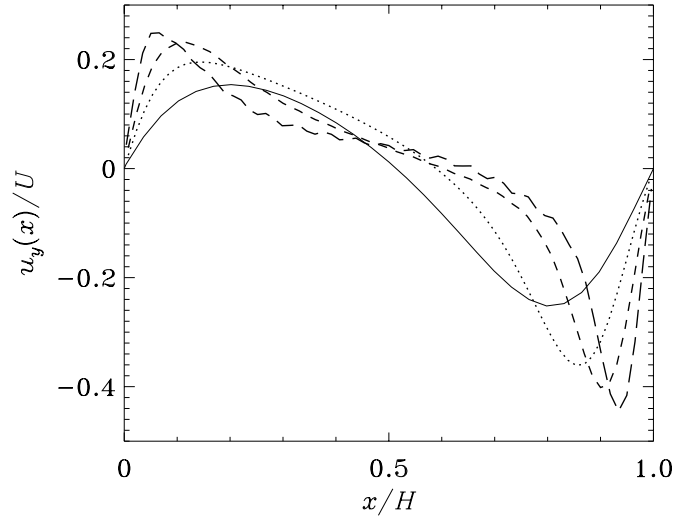
FIG. 8. 3-D lid-driven cavity flow. Effect of Reynolds number \text{Re} on the normalized transversal velocity profiles u_y(x, y, z)/U at y/H = z/H = 0.5 . The results are obtained by using D3Q19 LBE model with U = 0.1 , \text{Re} = 100 , N_x \times N_y \times N_z = 33^3 , \Delta = 0.5 (solid line); U = 0.1 , \text{Re} = 400 , N_x \times N_y \times N_z = 67^3 , \Delta = 0.5 (dotted line); U = 0.1 , \text{Re} = 1000 , N_x \times N_y \times N_z = 67^3 , \Delta = 0.5 (dashed line); and U = 0.1 , \text{Re} = 2000 , N_x \times N_y \times N_z = 67^3 , \Delta = 0.5 (long dashed line).
