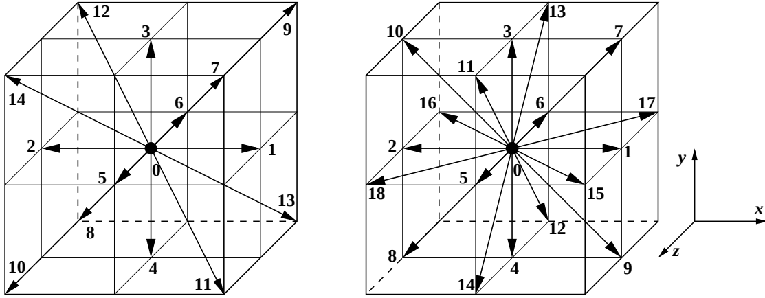
FIG. 15. Discrete velocity sets \{\mathbf{e}_\alpha\} for the D3Q15 (left) and D3Q19 (right) models.
