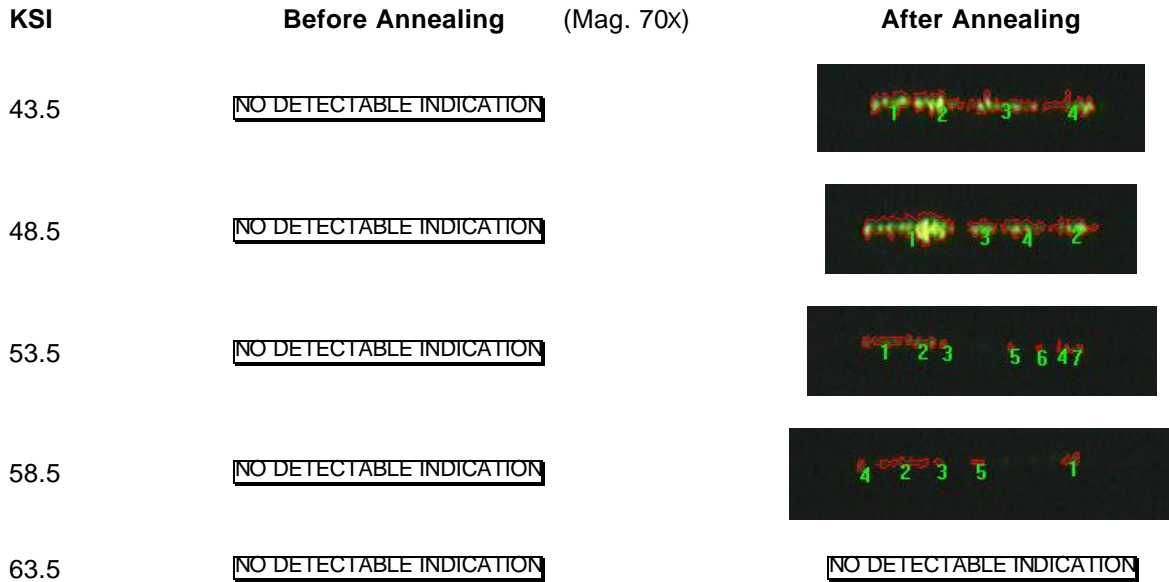
Figure 9. Fluorescent penetrant indications from the crack in specimen #63. (Part 2 of 2)
