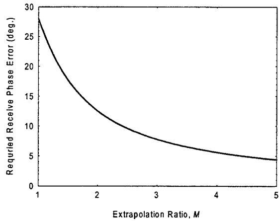
Figure 6. The RMS receive phase error that is required in order to achieve 1 dB of transmit beamforming loss is plotted as a function of the extrapolation ratio, M .
