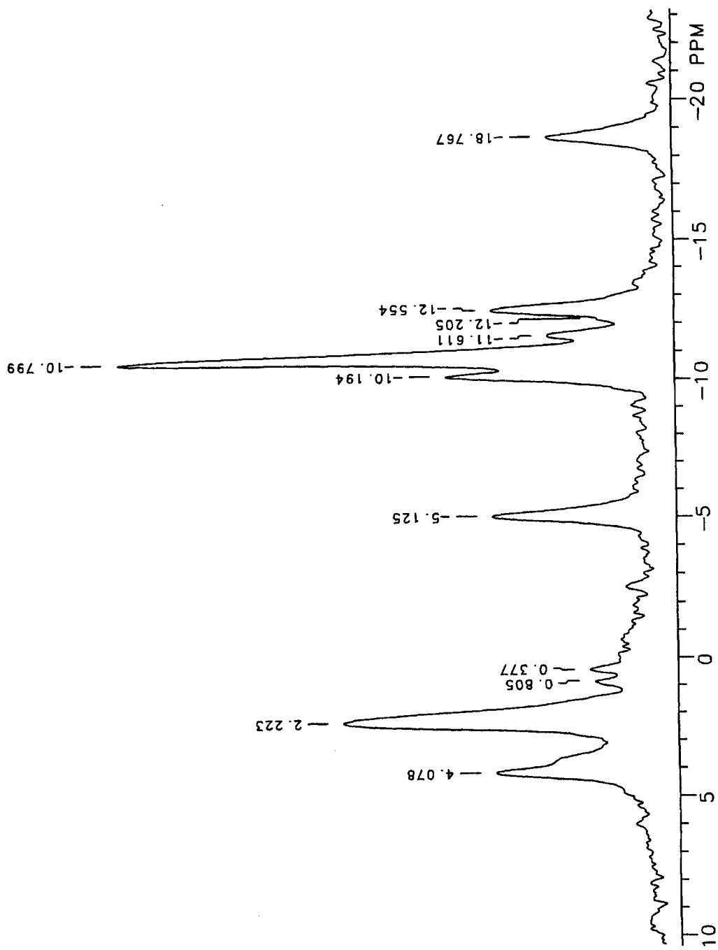
Figure 6. A ^{31}\text{P} spectrum of drug sensitive MC7 wild type cells treated with Tamoxifen ( 8 \mu\text{g/ml} ). The repetition time is 1 second. The number of transient is 2000. The RF pulse width is 36.1 \mu\text{s} . There is no difference compared with a spectrum taken from a Tamoxifen free medium.
