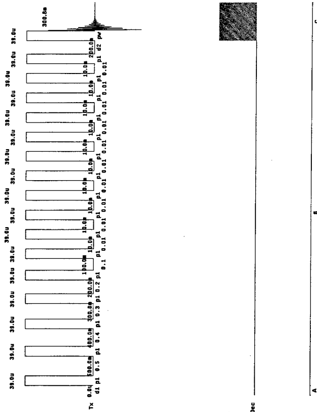
Figure 19. T1 relaxation time measurement. The NMR T1 relaxation times of all the phosphorus metabolites of MCF7 breast cancer cells were measured with the improved NMR perfusion system. (A) A saturation recovery technique is used. A series of 16 RF pulses flips the magnetization to a horizontal plane first. It follows by a 90° RF pulse and data acquisition period. (B) A list of measured T1 relaxation times for each phosphorus metabolites. The T1 values vary from 0.38 seconds for \beta -ATP and longer than 12 seconds for GPE.
