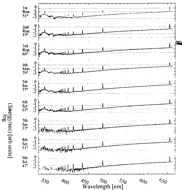
Figure 5. Series of emission spectra from ESEX arcjet showing continuum radiation from the nozzle and line structure from the plume.
