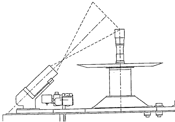
Figure 1. ESEX thruster (right) and video still camera field of view. Ram direction is up in this figure.
