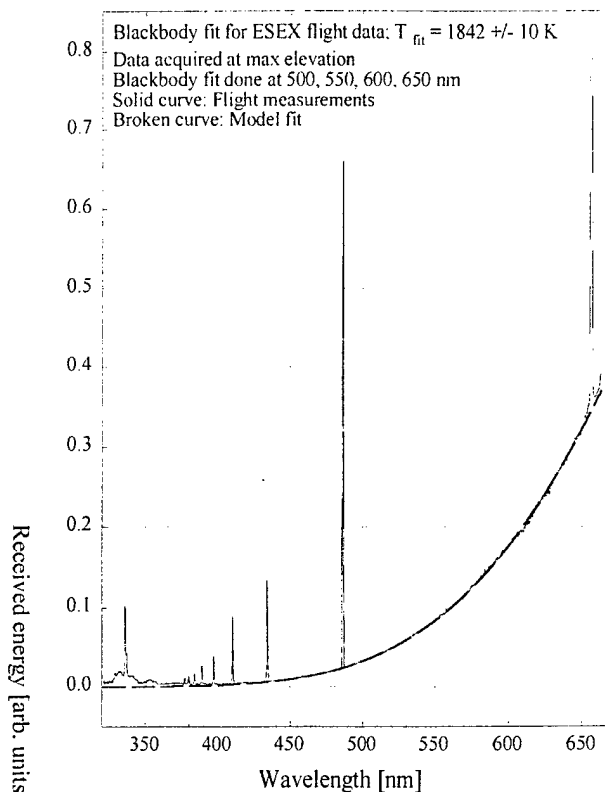
Figure 9. Blackbody fit to arcjet nozzle emission.
