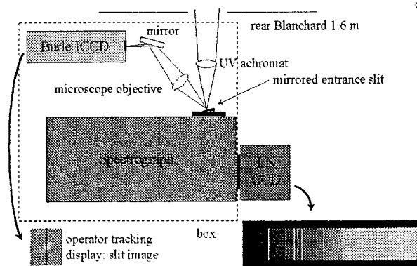
Figure 4. Schematic diagram of ESEX spectrograph, detector, and slit camera.
