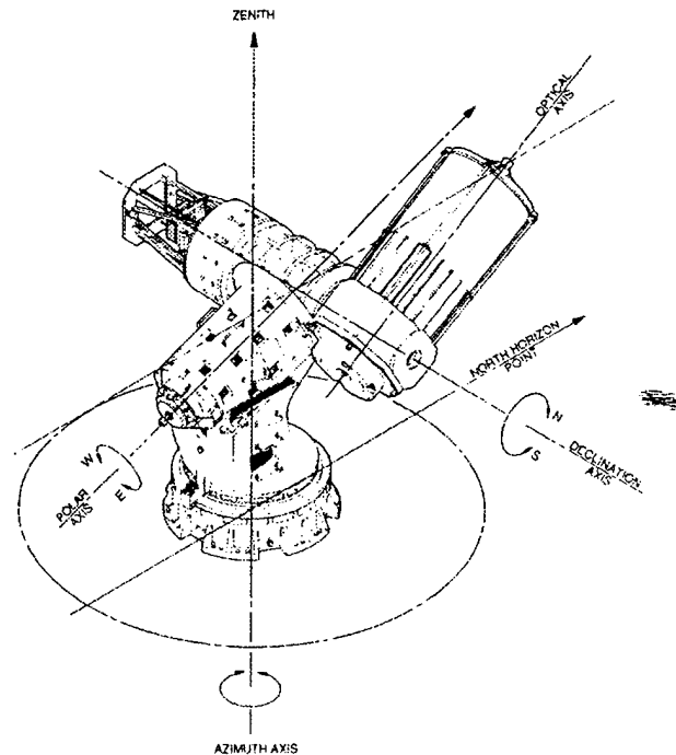
Figure 2. MSSS 1.6 telescope and 3-axis mount.
