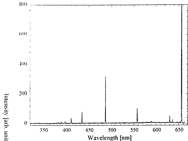
Figure 6. Spectrum obtained during arcjet firing well after nozzle is obscured by spacecraft body (The above is 10 th in the series, for comparison to Fig 5). Blackbody emission is gone but emission lines from the plume persist.
