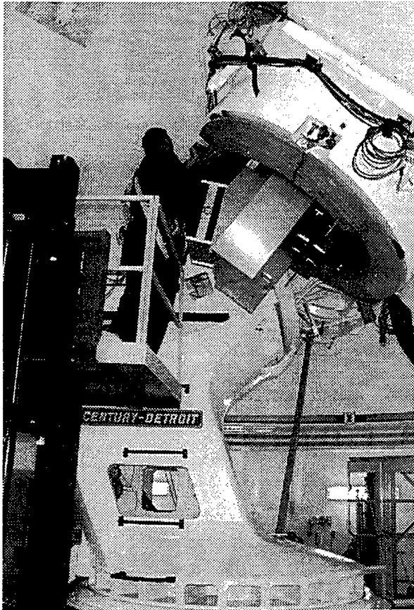
Figure 3. ESEX Spectrograph package mounted to the 1.6 m MSSS telescope.
