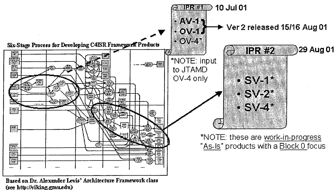
Figure 18. Structured Analysis for developing C4ISR architectures
