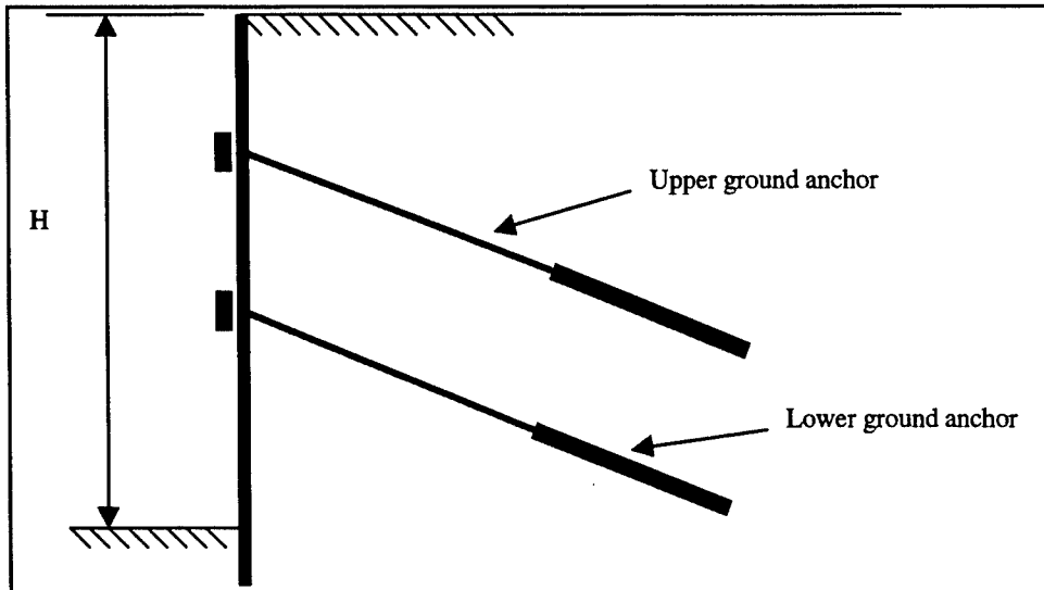
Figure 3.1. Tieback wall system
