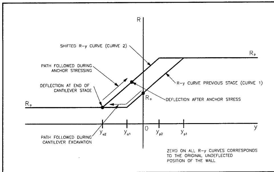
Figure 6.17. Shifted R - y curve to model construction stages (after Figure 86; Weatherby, Chung, Kim, and Briaud 1998)
