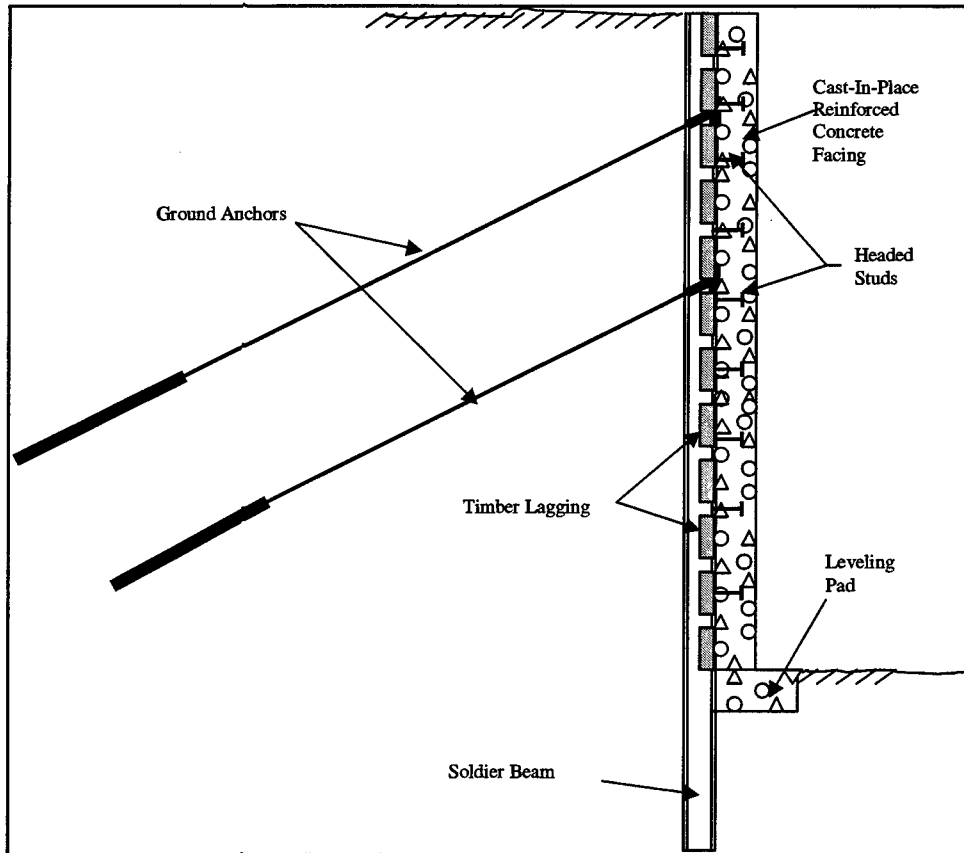
Figure 2.7. Soldier beam system with wood lagging and post-tensioned tieback anchors (general)
