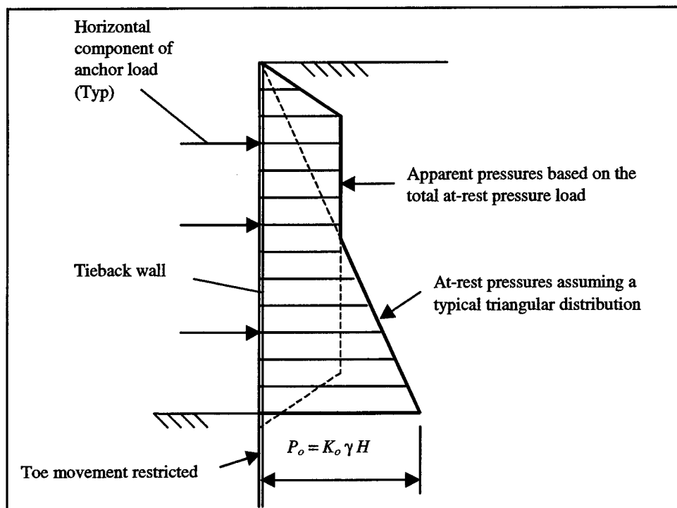
Figure 5.9. Pressure distribution when toe movements are restricted
