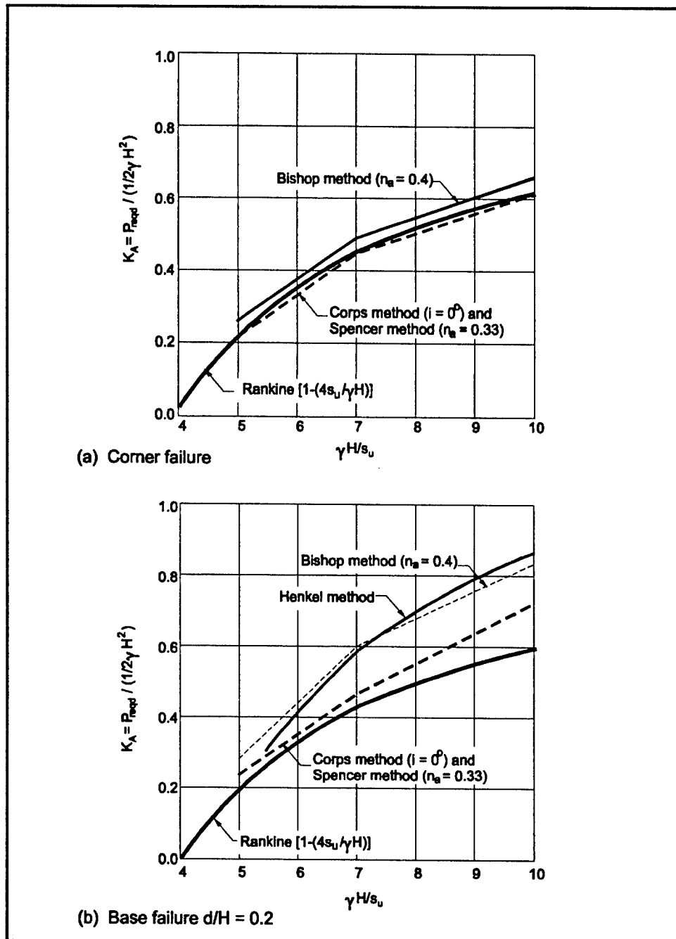
Figure 9.5. Comparison of limit equilibrium methods for cohesive soils (after Figure 50 of Sabatini, Pass, and Bachus 1999)
