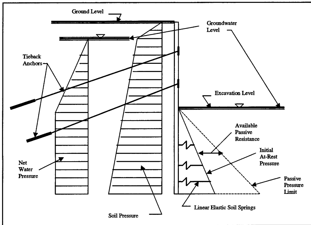
Figure 1.5. Linear elastic finite element model (LEFEM) of diaphragm wall in combination with linear Winkler soil springs
