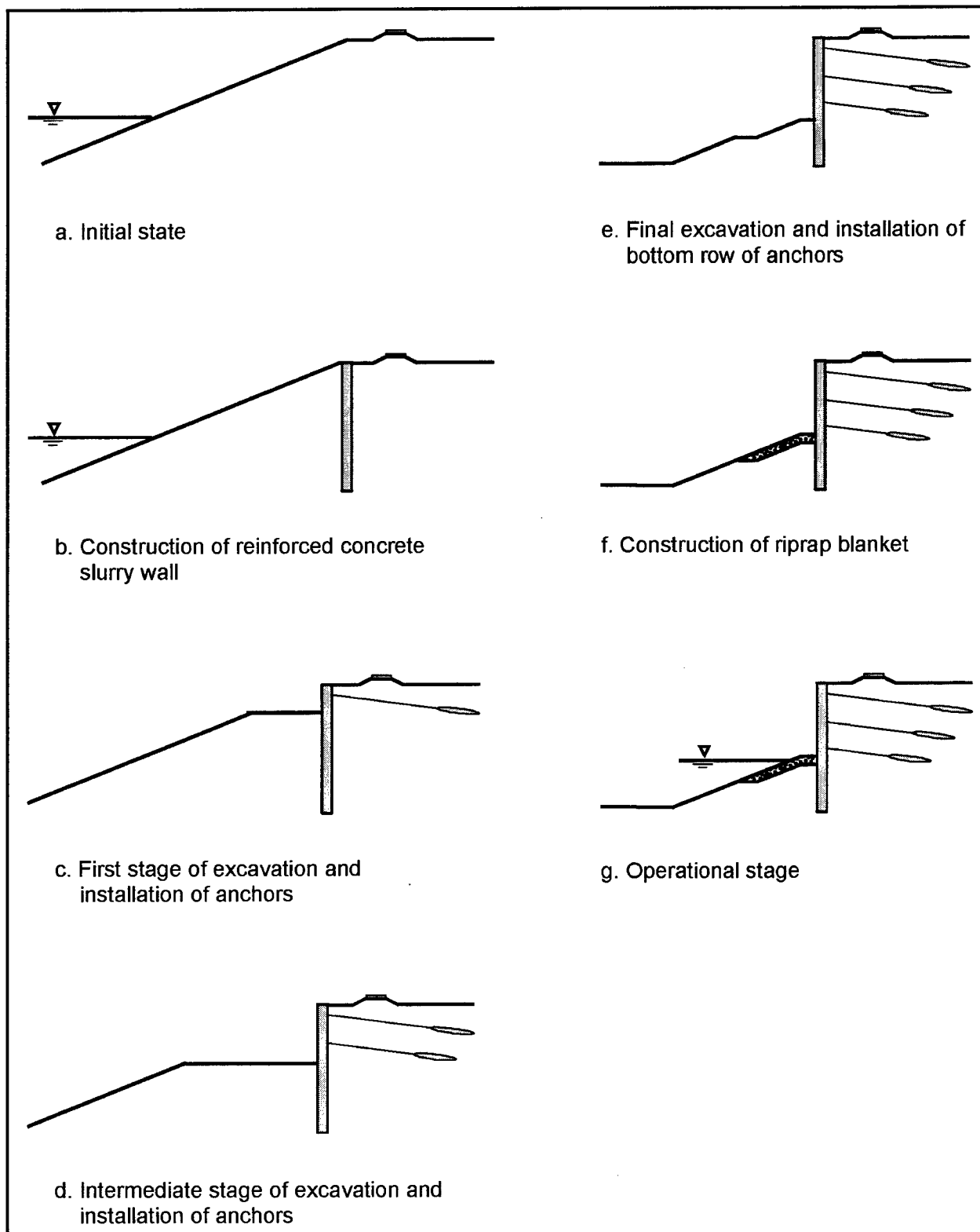
Figure 7.3. Typical construction and operation stages
