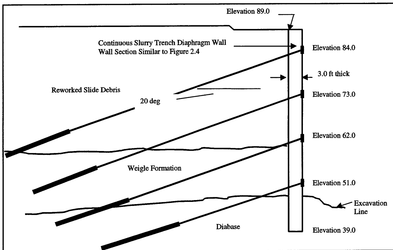
Figure 7.6. Bonneville Navigation Lock, temporary tieback wall—vertical section
