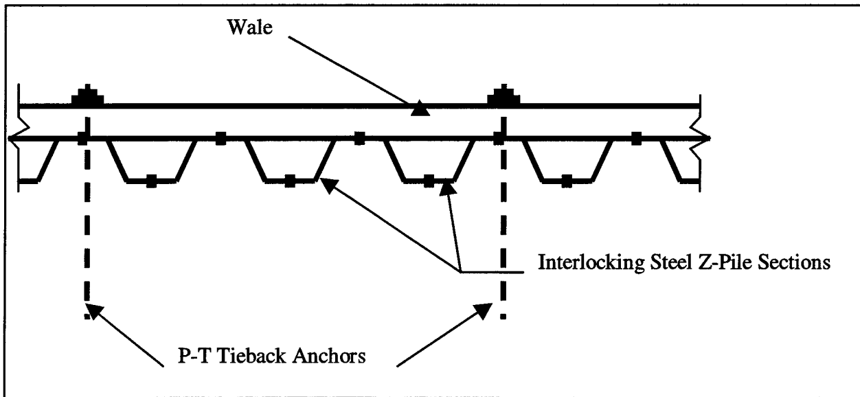
Figure 2.1. Vertical sheet-pile system with wales and post-tensioned tieback anchors
