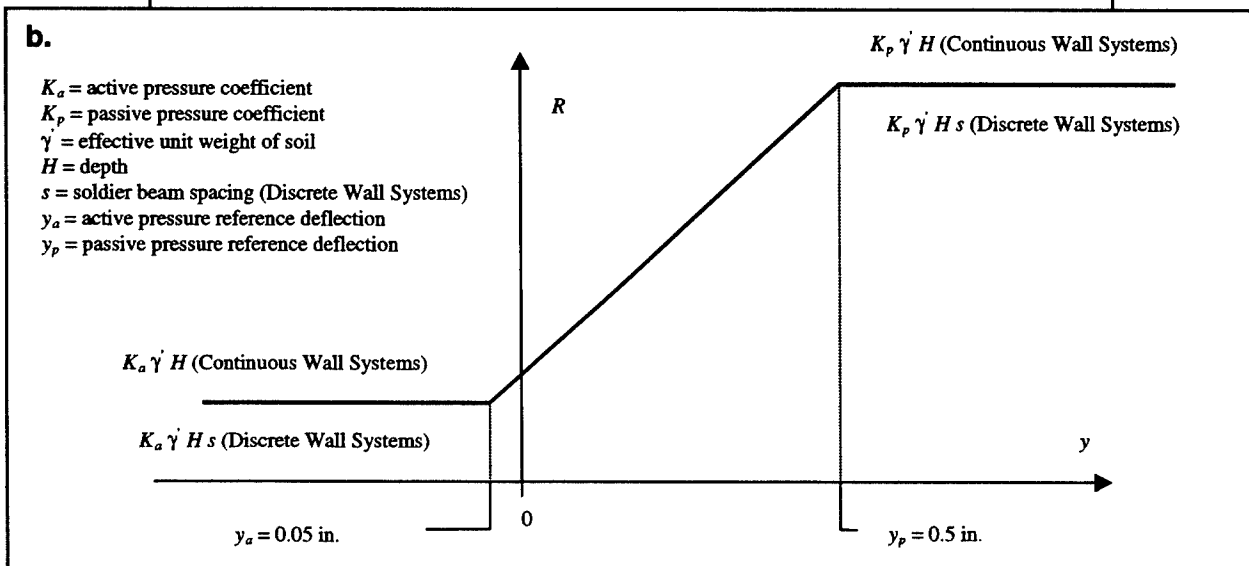
Figure 6.7. Diagram illustrating R - y curves for tieback walls in cohesionless soils (general R - y curve system per Weatherby, Chung, Kim, and Briaud 1998)
