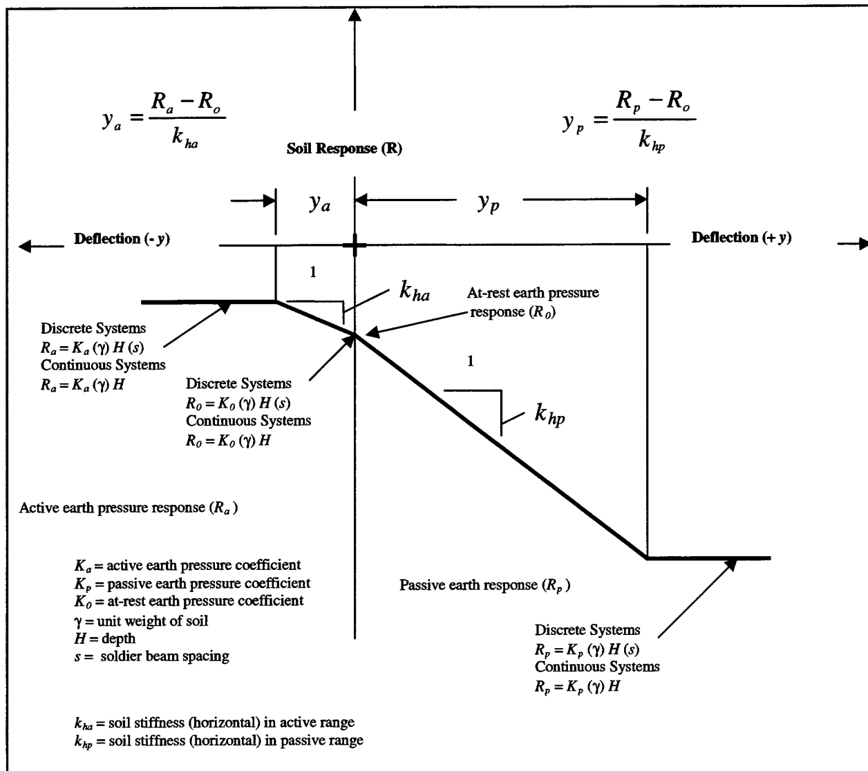
Figure 6.6. Idealized elastoplastic earth response-deflection ( R - y ) curve (right side soil spring per CBEAMC convention) (Dawkins 1994b)
