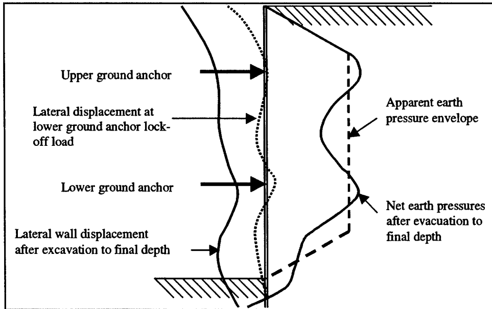
Figure 3.5. Lower tieback installation—final-stage excavation—lateral wall movements and earth pressures (after Sabatini, Pass, and Bachus 1999)
