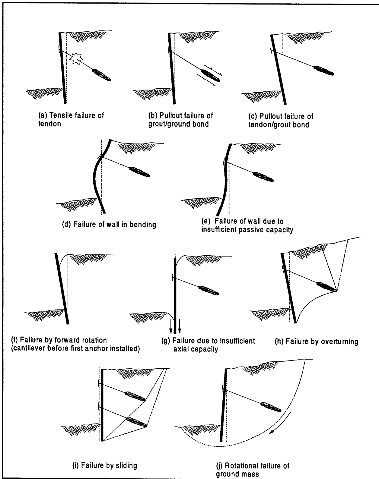
Figure 9.1. Potential failure conditions to be considered in design of anchored walls (after Figure 11 of Sabatini, Pass, and Bachus 1999)
