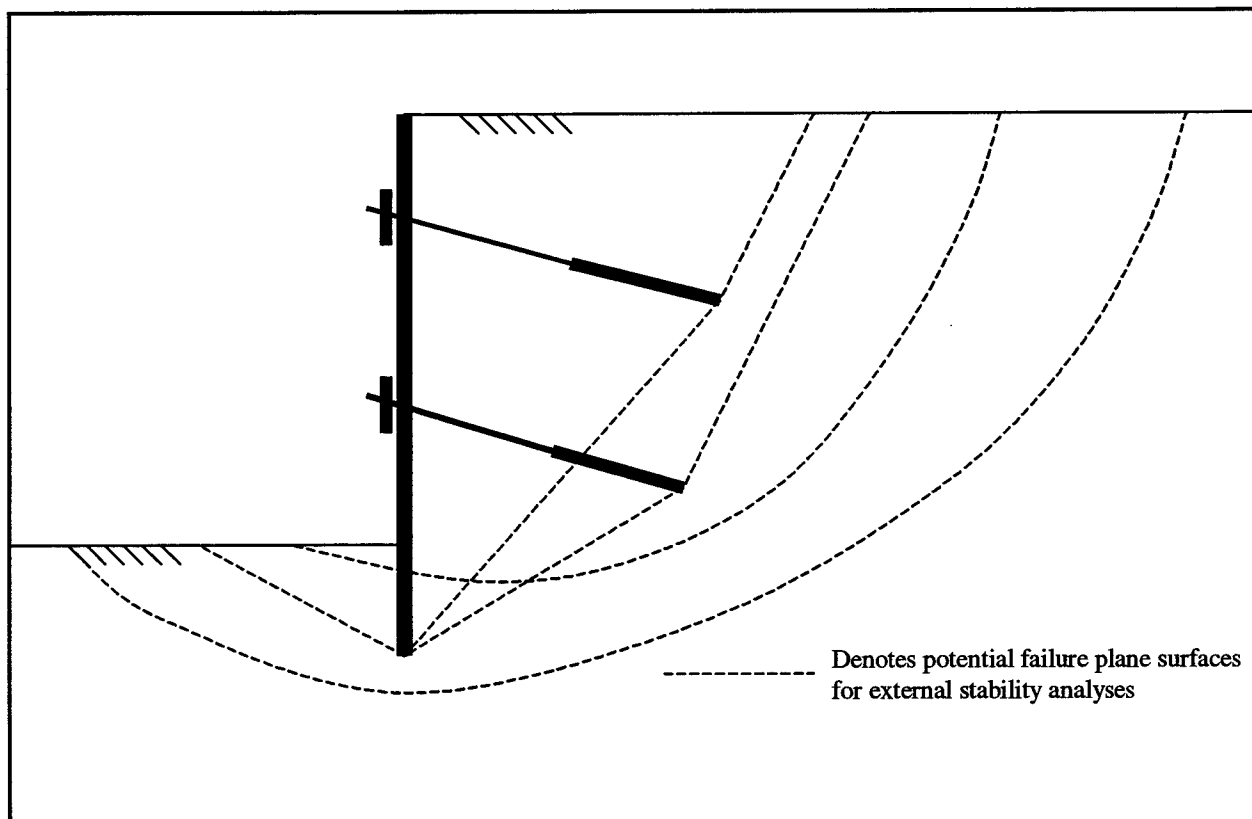
Figure 9.2. Failure surfaces for external stability evaluations (after Figure 52 of Sabatini, Pass, and Bachus 1999)
