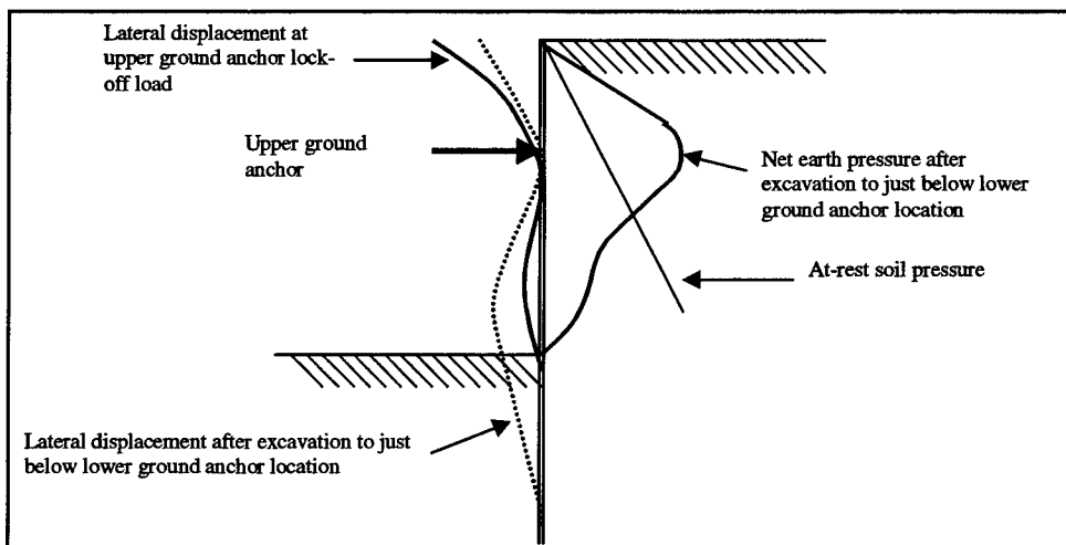
Figure 3.4. Second stage excavation—lateral wall movements and earth pressures (after Sabatini, Pass, and Bachus 1999)
