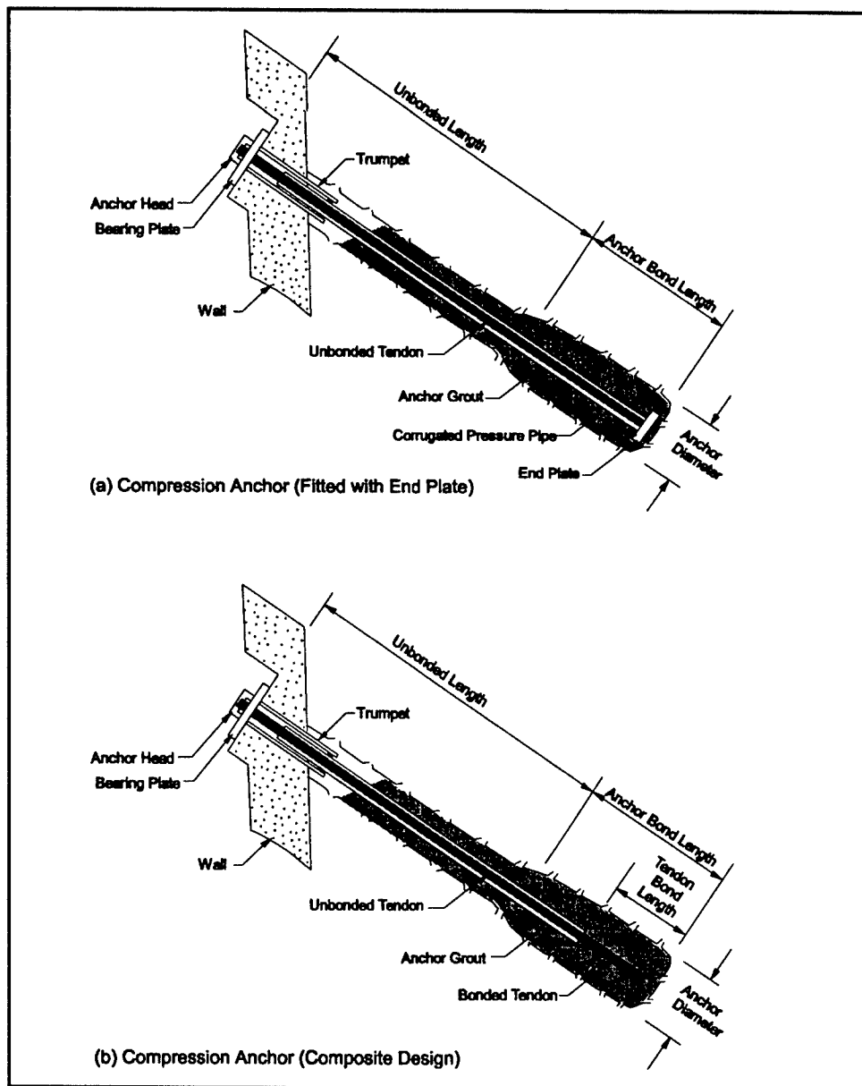
Figure 8.3. Types of compression anchors (after Figure 35 of Sabatini, Pass, and Bachus 1999)
