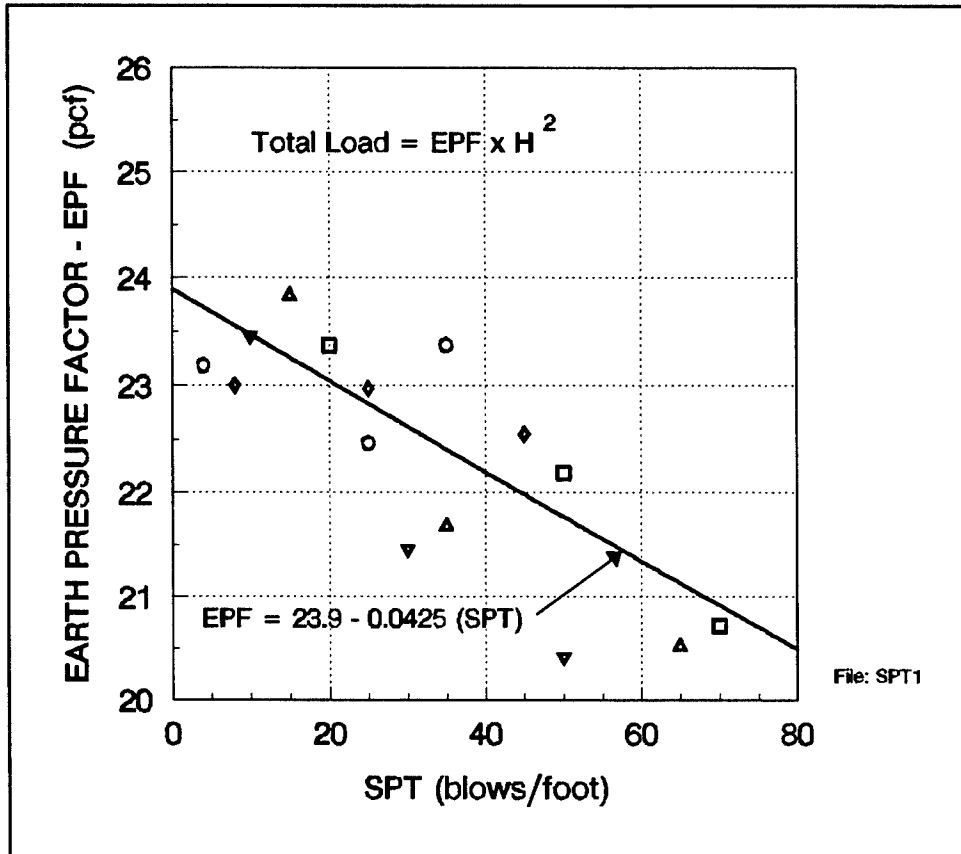
Figure 5.5. Earth pressure factors (EPF) as a function of standard penetration resistance – symbols represent plot of Table 5.1 data (adapted from Figure 30, Weatherby 1998)
