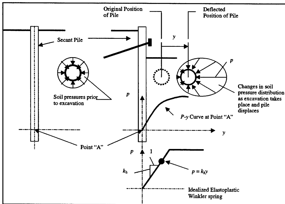
Figure 6.1. Concept of p - y curve
