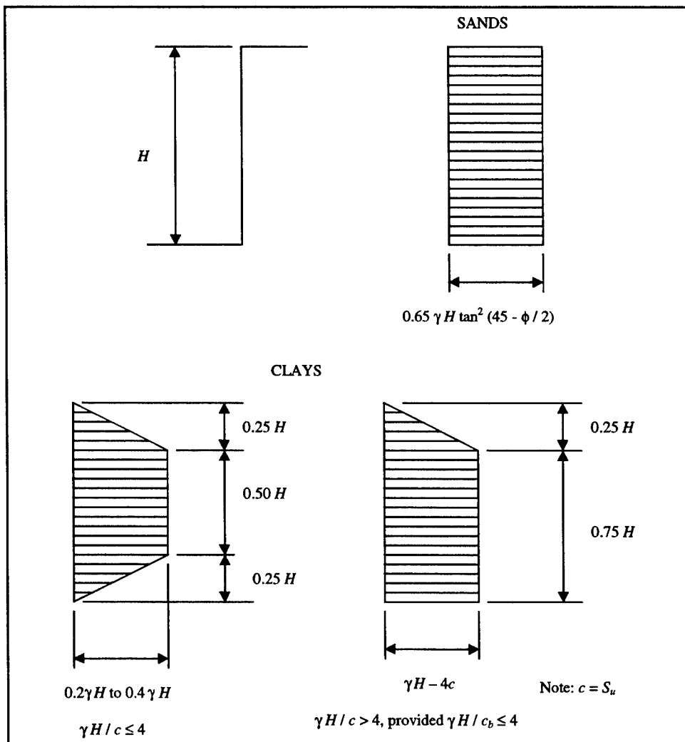
Figure 5.2. Apparent earth pressure diagrams (adapted from Figure 19, Weatherby 1998)
