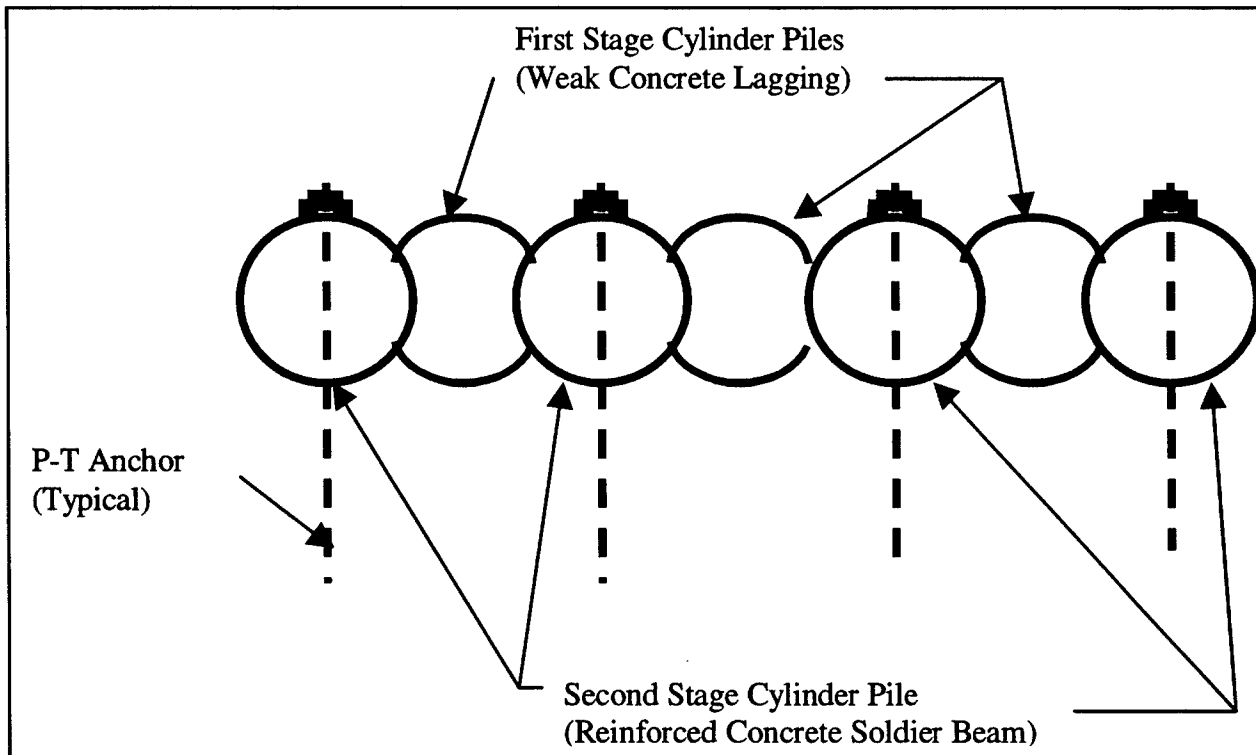
Figure 2.3. Secant cylinder pile system with post-tensioned tieback anchors
