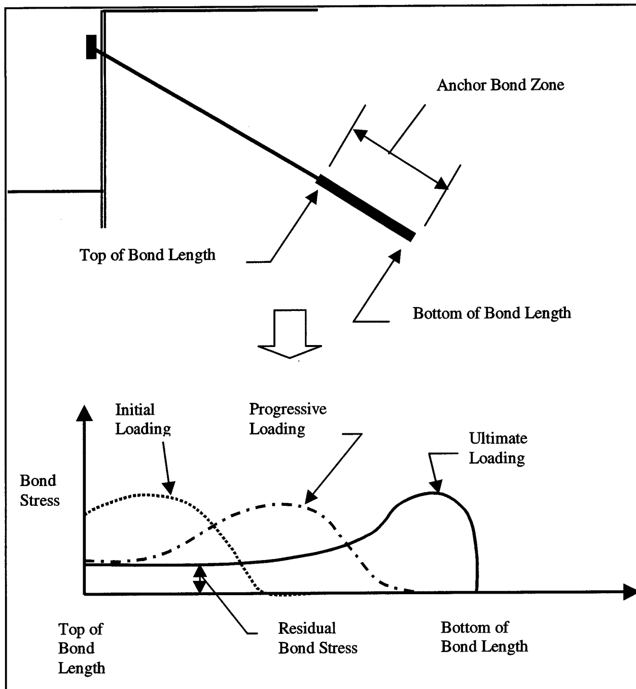
Figure 8.4. Mobilization of bond stress for a tension anchor in anchor bond zone
