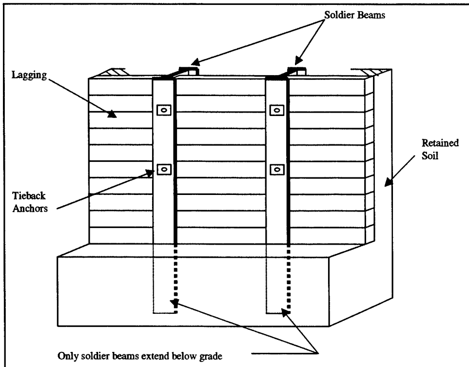
Figure 2.13. Discrete wall system
