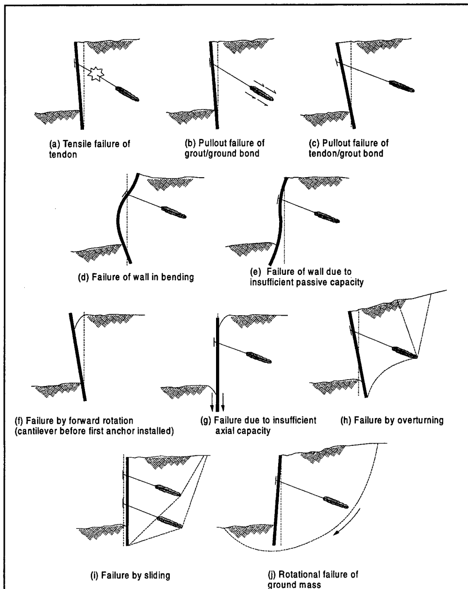
Figure 3.12. Potential failure conditions to be considered in design of anchored walls (after Figure 11; Sabatini, Pass, and Bachus 1999)
