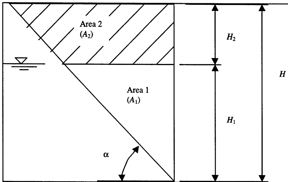
Figure 5.16. Method 2, effective unit weight for partially submerged soils (from Ebeling and Morrison 1992)
