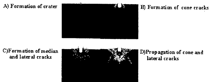
Figure 3. Numerical simulation of damage induced by the impact of a 0.55 mm diameter steel spherical particle on a fused silica target at a velocity of 3670 m/s (red area is anisotropically damaged).
