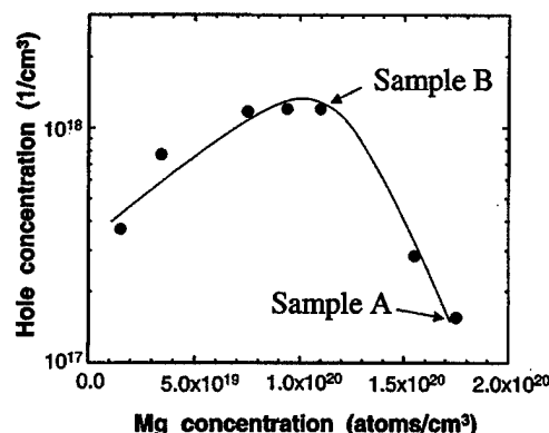
FIG. 1. Room-temperature Hall measurements of the hole concentration as a function of the Mg concentration (determined by SIMS) for a series of Mg-doped GaN films.
