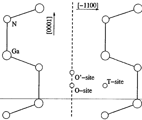
FIG. 5. Schematic representation of atomic positions in the (11\bar{2}0) plane of wurtzite GaN. The large circles represent Ga atoms, medium circles N atoms. The high-symmetry interstitial sites are indicated: O is the octahedral interstitial site and T the tetrahedral interstitial site. O' indicates the position of the global minimum for \text{Be}_{int}^{2+} .
