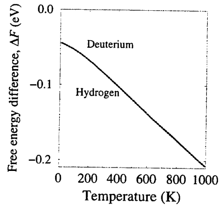
Figure 3: Free energy differences between \text{AB}_{N,\perp} and \text{OA}_{\parallel} configurations of Mg-H and Mg-D complexes as a function of temperature.
