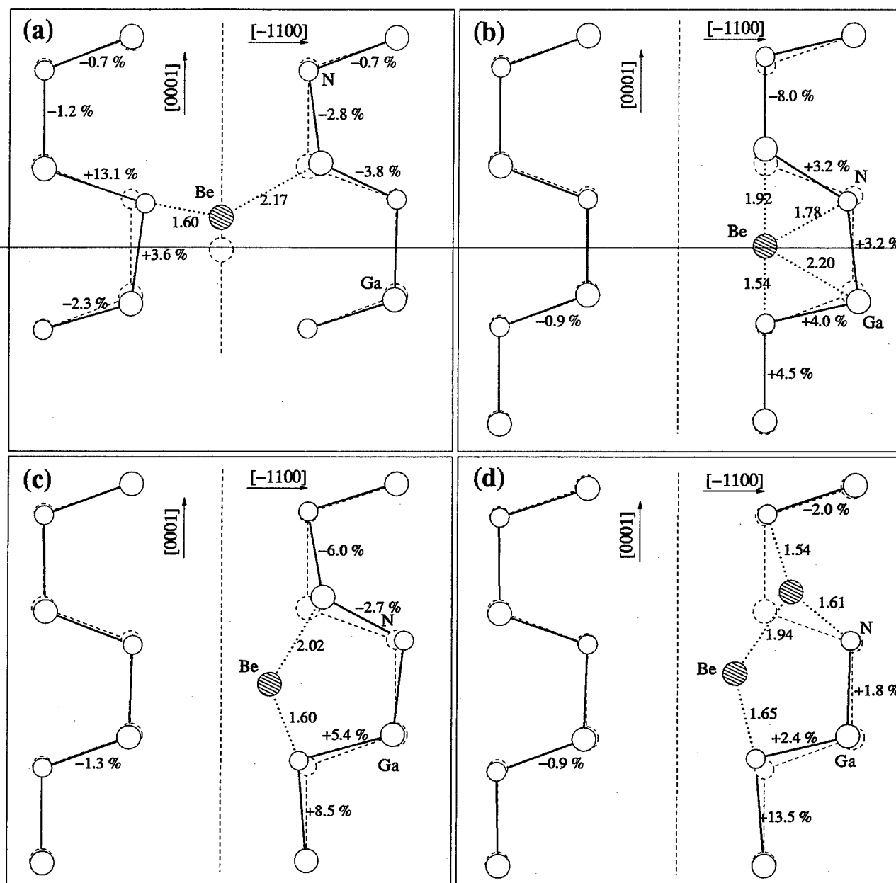
FIG. 6. Schematic representation of atomic positions in the (11\bar{2}0) plane for \text{Be}_{\text{int}}^{2+} at various interstitial sites in wurtzite GaN. Large circles represent Ga atoms, medium circles N atoms, and the hatched circle represents Be. Dashed circles indicate ideal atomic positions, dashed lines bonds in the ideal lattice. Distances between Be and its neighbors are given in Å and changes in Ga-N bond lengths are given as the percentage change from the bulk Ga-N bond lengths. The panels correspond to a Be interstitial in the following configurations: (a) O' site; (b) T site; (c) A site; and (d) the \text{Be}_{\text{Ga}}\text{-Be}_{\text{int}}^+ complex.
