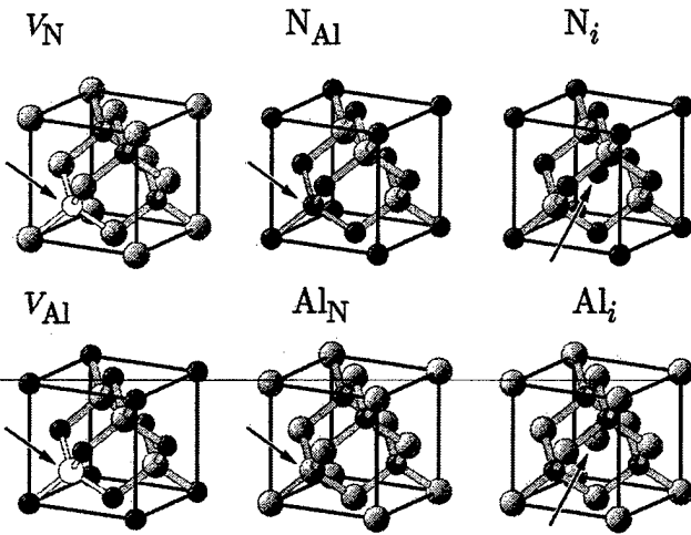
FIG. 1. Atomic geometry of native point defects in zinc-blende AlN in the ideal (unrelaxed) structure. Large gray and small dark spheres represent Al and N atoms, respectively. Vacancies are indicated by the white circles.
