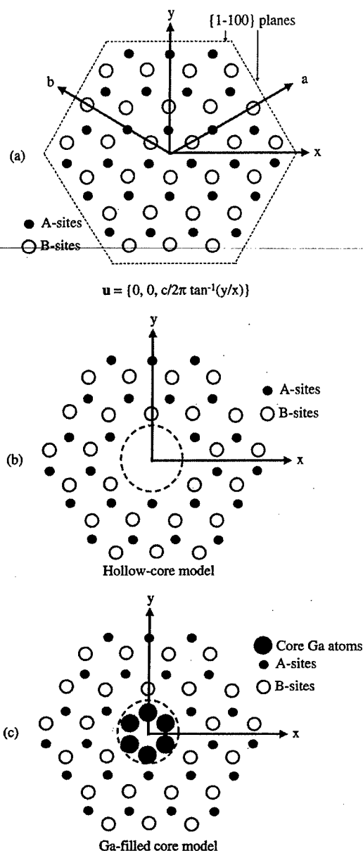
FIG. 1. (a) (0001) projection of the supercell employed to model a screw dislocation. The closed circles represent Ga and N atoms in the A sites of the wurtzite lattice. The open circles represent Ga and N atoms in B sites. Not shown are the H atoms which saturate the 18 Ga and 18 N dangling bonds in each cell on the six {10-10} surfaces. Each supercell contains one prismatic crystal of GaN. The supercell vectors \mathbf{a} and \mathbf{b} give rise to a periodic hexagonal arrangement of prisms in the x - y plane. The structure is periodic in the z direction with periodicity c = 5.1 Å. The screw dislocation is generated by applying the displacement (0,0,\Delta z) . (b) A stoichiometric hollow core dislocation is created by removing the Ga and N atoms from within the central core of the filled core dislocation. (c) The Ga-filled core is obtained by removing the nitrogen atoms from the central core. The Ga atoms in the core form a pair of helices, each with pitch 2c .
