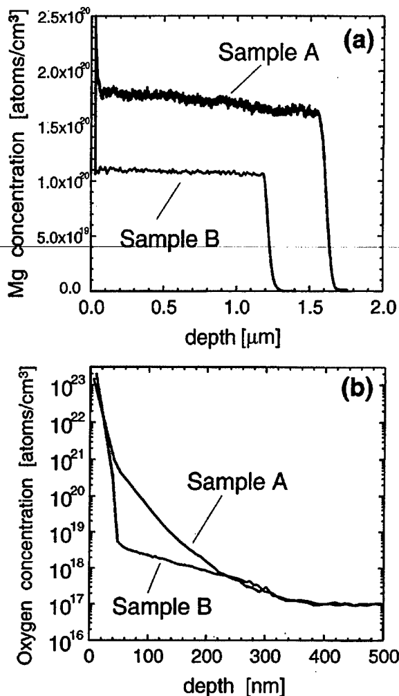
FIG. 2. SIMS depth profiles of the (a) Mg concentration and (b) O concentration for the high-doped (sample A) and medium-doped (sample B) GaN:Mg samples.
