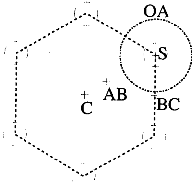
Figure 2: Lattice locations considered for the analysis of ion-channeling measurements by Wampler et al. [8]. Projected positions of hydrogen in the \text{OA}_{\parallel} configuration are shown as the dash-dotted circle.
