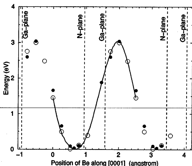
FIG. 8. Total energy of \text{Be}_{\text{int}}^{2+} at positions along the center of the open channel in WZ GaN, measured from the O site, and referenced to the energy at the global minimum ( O' ). Solid circles: the results from 1 \times 1 \times 1 k -mesh calculations; open circles: 2 \times 2 \times 2 k -mesh calculations; solid line: interpolation curve.
