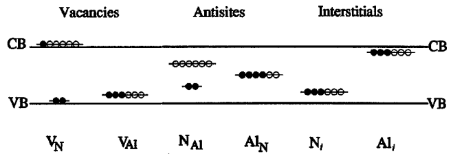
FIG. 2. Schematic representation of the defect-induced electronic states in zinc-blende AlN for the neutral charge state. Filled and open circles denote electrons and holes, respectively.
