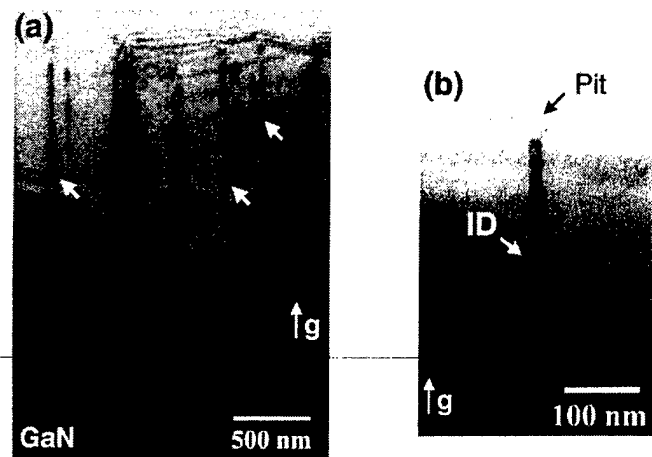
FIG. 3. TEM images of sample A taken with g=0002 near the [1120] zone axis. (a) Low magnification image showing the interface (dotted line) between the doped and the undoped layer. Inversion domains (ID) are indicated by arrows. Modulated strain contrast fringes are observed only in the doped layer. (b) High magnification image of an isolated ID associated with a pit at the film surface.
