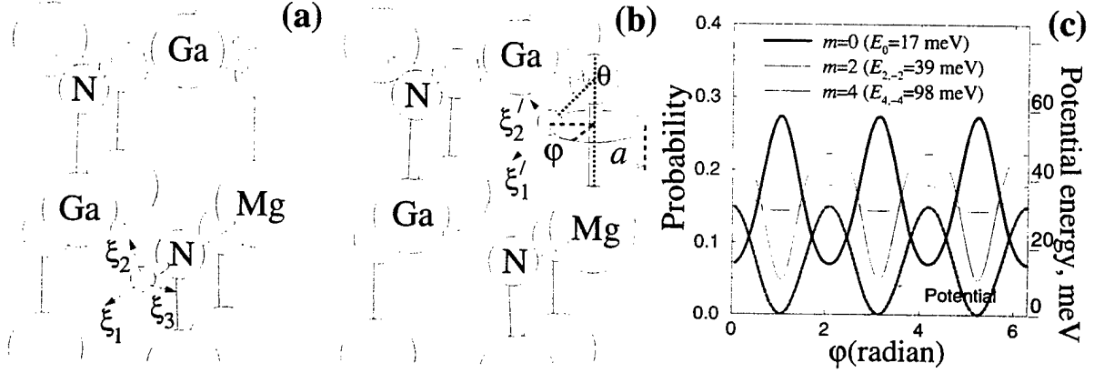
Figure 1: Perspective view of Mg-H complexes in (a) the \text{AB}_{\text{N},\perp} and (b) the \text{OA}_{\parallel} configurations. The path of H rotating around the bond axis is also shown in (b). (c) Quantum-mechanical probabilities to find H at an angle \phi in the \text{OA}_{\parallel} configuration, for a few selected states (solid lines). The ground state (with energy 17 meV) is shown as a thick line, the 3rd excited state as a medium line (39 meV) and the 8th excited state as a thin line (98 meV). The potential used in the calculation is shown as a thin dashed line.
