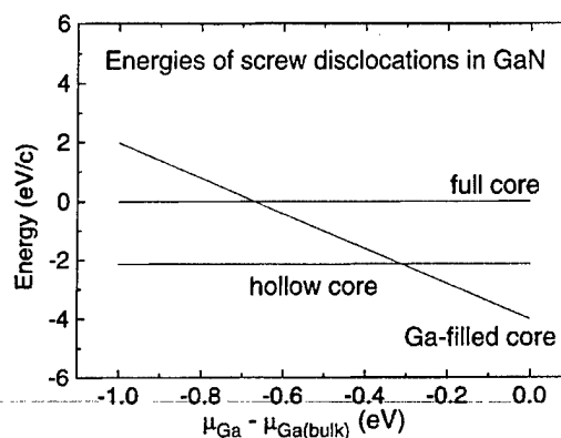
FIG. 2. Relative energies of possible screw dislocations as a function of the Ga chemical potential. The upper limit on \mu_{\text{Ga}} is \mu_{\text{Ga(bulk)}} . The Ga-filled core model is energetically favorable with respect to the hollow core model for \mu_{\text{Ga}} - \mu_{\text{Ga(bulk)}} > -0.31 eV.
