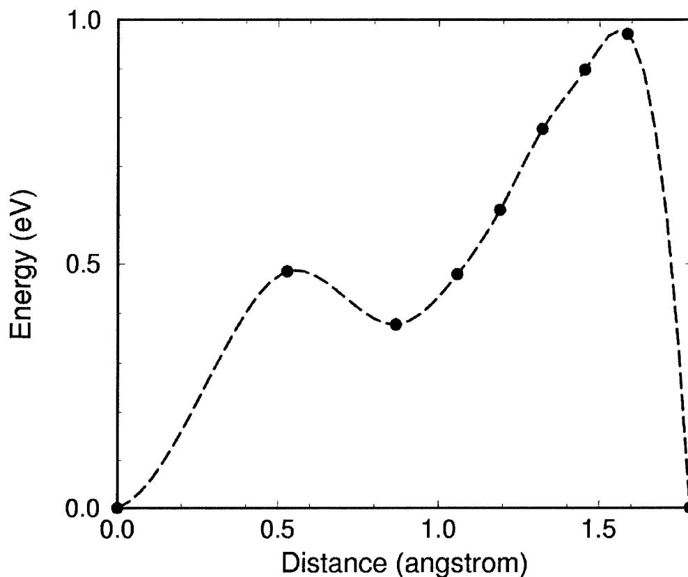
Figure 2: Total energy (referenced to the ground-state configuration) of \text{Ga}_i^{3+} as a function of the horizontal distance of the \text{Ga}_i atom measured from the center of the hexagonal channel towards the T site. By the time the \text{Ga}_i has reached the T site, it has moved through a triangle of N atoms and replaced a Ga host atom, pushing the original Ga host atom off its lattice site to become the new \text{Ga}_i .
