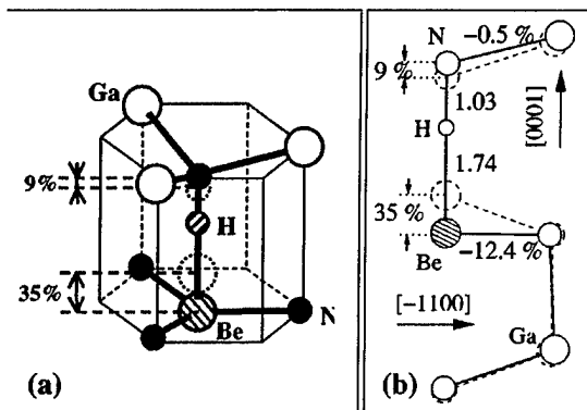
FIG. 9. Schematic illustration of the atomic structure of the Be-H complex. The H atom is located in a bond-center site along the c axis. The \text{Be}_{\text{Ga}}^- is relaxed outward by a very large amount, moving it into the plane of its three N neighbors.
