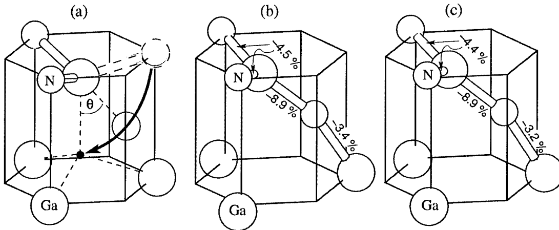
Figure 4: Ball-and-stick model of atomic positions describing the diffusion process of the nitrogen vacancy. (a) Illustration of the migration path. (b) The saddle-point configuration of V_N^{3+} . (c) The saddle-point configuration of V_N^+ . Large spheres represent Ga atoms, medium spheres N atoms, and the black dot shows the ideal lattice site of the vacancy. The percentages denote the changes from the bulk Ga-N bond length.
