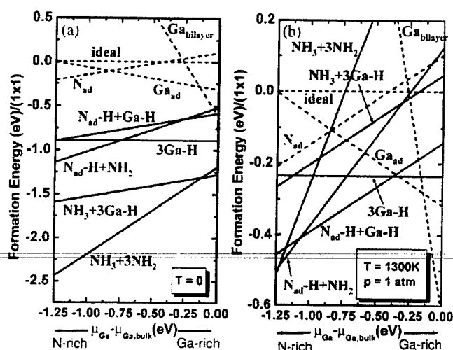
FIG. 1. Calculated formation energies for GaN(0001) surfaces, as defined in Eq. (1), as a function of \mu_{\text{Ga}} . All structures (except Ga bilayer ) have 2 \times 2 periodicity, but energies are expressed in eV per 1 \times 1 cell. Dashed lines indicate hydrogen-free surfaces. (a) T = 0 ; (b) T = 1300 K, p(\text{H}_2) = 1 atm. Note the very different energy scale in the two plots.
