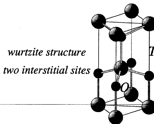
FIG. 5. Schematic representation of the wurtzite structure indicating the two high-symmetry interstitial positions T and O . Large gray and small dark spheres represent cations and anions, respectively.
