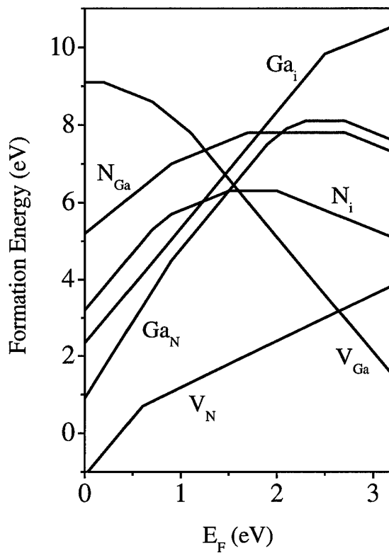
Figure 1: Formation energies as a function of Fermi level for native point defects in GaN. Ga-rich conditions are assumed. The zero of Fermi level corresponds to the top of the valence band. Only segments corresponding to the lowest-energy charge states are shown. The slope of these segments indicates the charge state. Kinks in the curves indicate transitions between different charge states.
