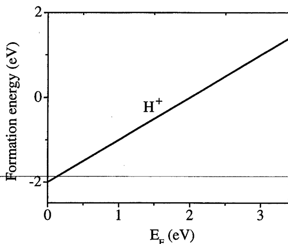
Fig. 4 Formation energy of the positive charge state of hydrogen in ZnO as a function of Fermi level. E_F = 0 corresponds to the top of the valence band. The chemical potential of hydrogen was chosen to correspond to H_2 molecules at T=0 . Charge states other than the positive are not stable.
