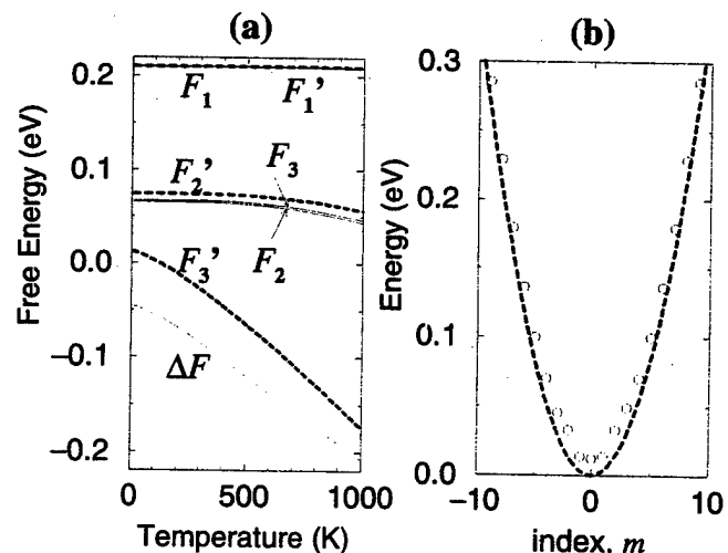
FIG. 3. (a) Free energies as a function of temperature. The thin solid lines indicate the free energy associated with the vibrational stretching ( F_1 ) and bending ( F_{2,3} ) modes of Mg-H complexes in the AB_{N,\perp} configuration; the dashed lines apply to the OA_{\parallel} configuration, where F_3 corresponds to the rotational mode. The free-energy difference \Delta F is shown as the thick solid line; it is almost entirely due to the difference between F_3 and F_3' . (b) Energy levels for the nearly free rotor in the OA_{\parallel} configuration of the Mg-H complex, calculated using an energy barrier E_{b\phi} = 32 meV and a radius a = 0.79 Å. The dashed line is a perfect parabola, reflecting the solutions for a free rotor.
