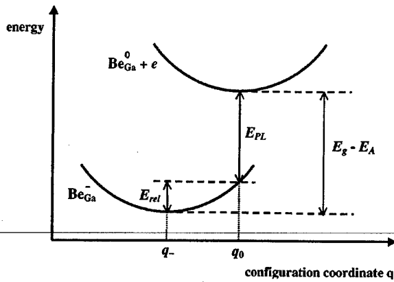
FIG. 2. Schematic configuration coordinate diagram illustrating the difference between thermal and optical ionization energies. The curve for \text{Be}_{\text{Ga}}^0 is vertically displaced from that for \text{Be}_{\text{Ga}}^- assuming the presence of an electron in the conduction band. E_{\text{rel}} is the Franck-Condon shift, i.e., the relaxation energy that can be gained, in the negative charge state, by relaxing from configuration q_0 (equilibrium configuration for the neutral charge state) to configuration q_- (equilibrium configuration for the negative charge state).
