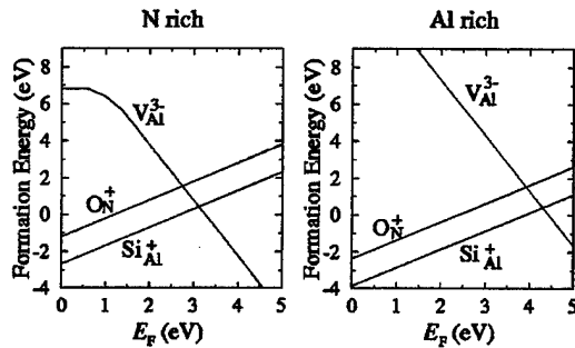
FIG. 7. Formation energies (LDA) of impurities and defects relevant for n -type AlN, as a function of the Fermi level under nitrogen-rich (left panel) and aluminum-rich (right panel) conditions. Oxygen and silicon are donor impurities, and the Al vacancy is the dominant compensating defect. E_F=0 corresponds to the valence-band maximum.
