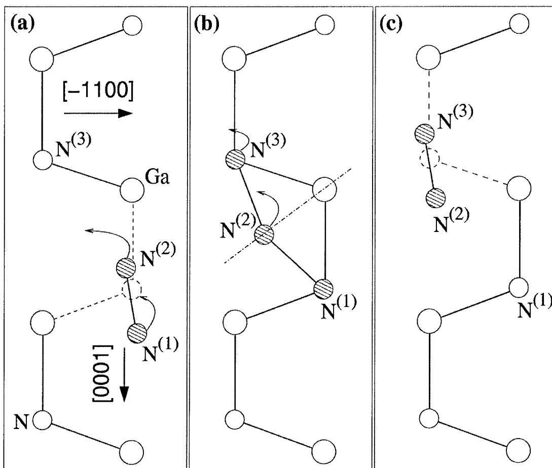
Figure 3: Schematic illustration of the migration of interstitial nitrogen via an interstitialcy mechanism. (a) Ground state. (b) Saddle-point configuration. (c) New ground state, after one migration step. Large circles represent Ga atoms, medium circles N atoms, and shaded medium circles highlight N atoms involved in the migration. Dashed circles indicate ideal atomic position of the lattice N, dashed lines bonds in the ideal lattice. The numbers in square brackets identify the migrating atoms. The center of mass of the two closest nitrogen atoms is also indicated.
