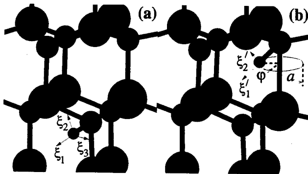
FIG. 2. Perspective view of Mg-H complexes in (a) the AB_{N,\perp} and (b) the OA_{\parallel} configuration. The path of H rotating around the crystal axis is also shown in (b). The directions of vibration for stretching ( \xi_1 ) and bending modes ( \xi_2, \xi_3 ) are indicated by arrows; in (b), \xi_3 is replaced by the azimuthal angle \phi describing the rotational motion of H.
