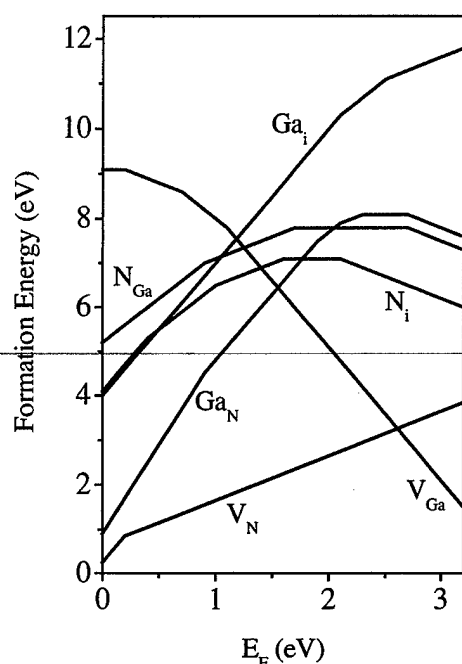
Fig. 1 Formation energies as a function of Fermi level for native point effects in GaN under Ga-rich conditions. E_F = 0 corresponds to the top of the valence band.
