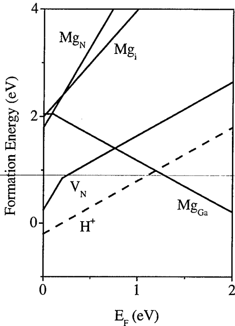
Fig. 3 Formation energies as a function of Fermi level for defects and impurities relevant for p -type GaN, under Ga-rich conditions. E_F = 0 corresponds to the top of the valence band.
