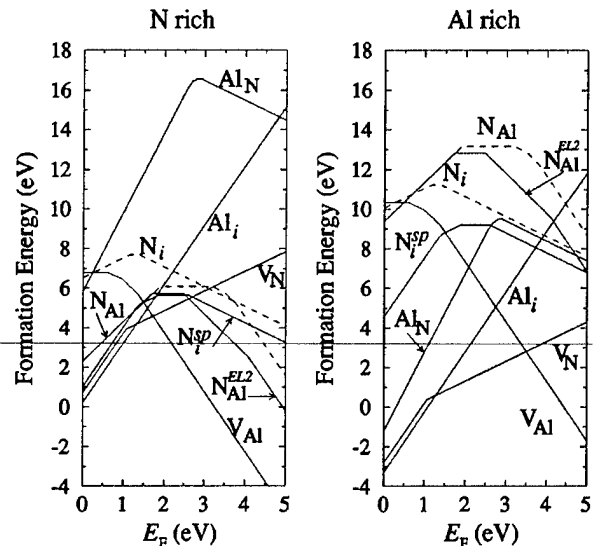
FIG. 4. Defect formation energies (LDA) for native point defects in zinc-blende AlN as a function of the Fermi level under nitrogen-rich (left panel) and aluminum-rich (right panel) conditions. E_F = 0 corresponds to the valence-band maximum.
