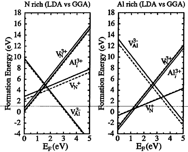
FIG. 6. Comparison of GGA (dashed lines) and LDA (solid lines) results for defect formation energies of various low-energy point defects in zinc-blende AlN. Formation energies are shown as a function of the Fermi level under nitrogen-rich (left panel) and aluminum-rich (right panel) conditions. E_F=0 corresponds to the valence-band maximum.
