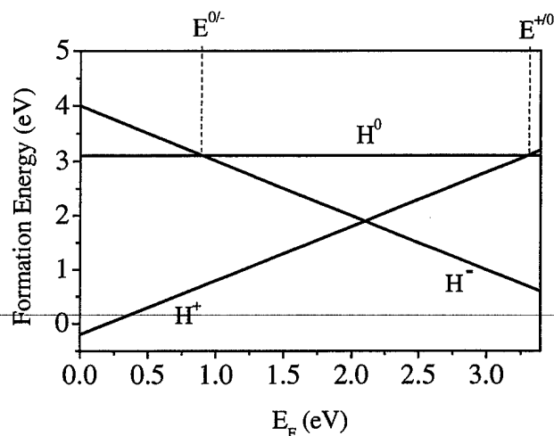
Fig. 2 Formation energies of various charge states of hydrogen in GaN as a function of Fermi level. E_F = 0 corresponds to the top of the valence band. The chemical potential of hydrogen was chosen to correspond to \text{H}_2 molecules at T=0 .
