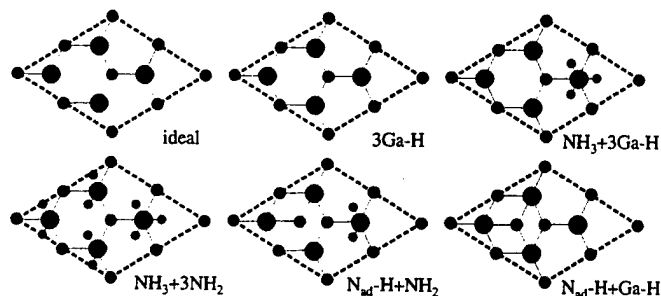
FIG. 2. Schematic top view of prevalent 2 \times 2 reconstructions for GaN(0001) surfaces. Large open circles represent Ga atoms, solid circles N, and small open circles H.
