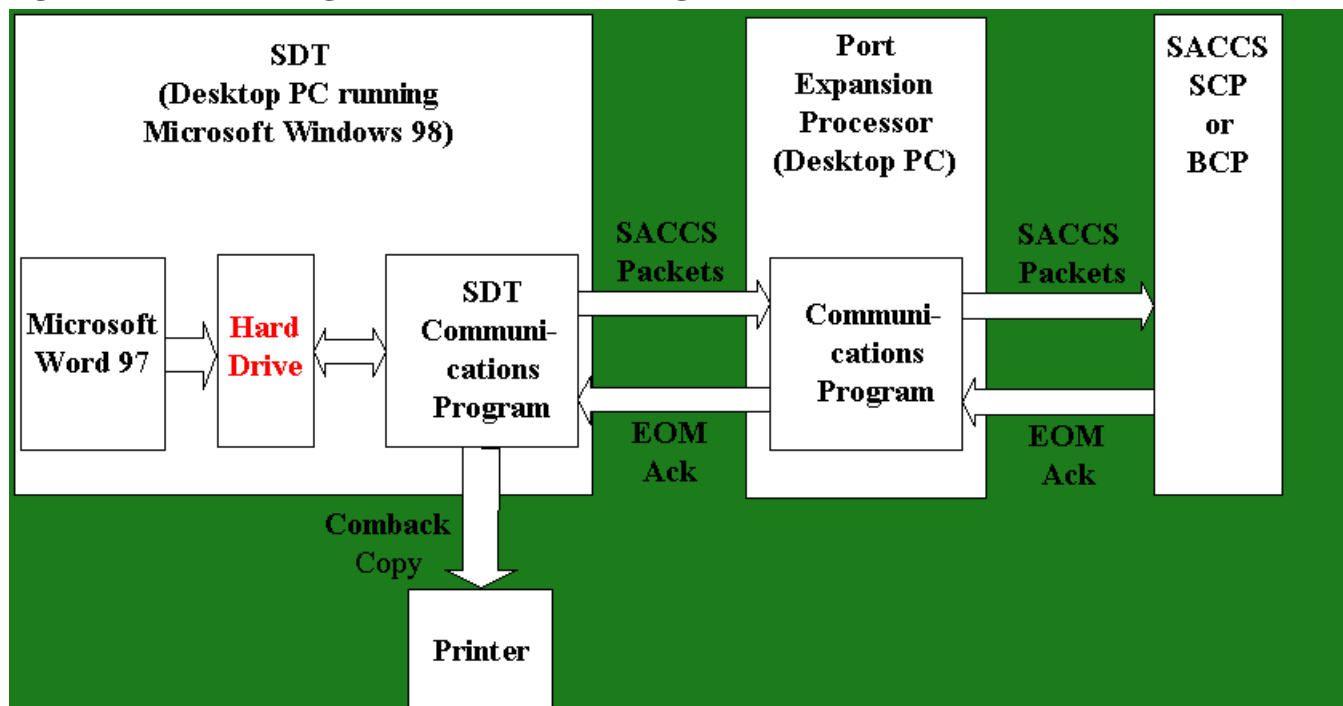
Figure 5.1. SDT Message Transmission Flow Diagram.
