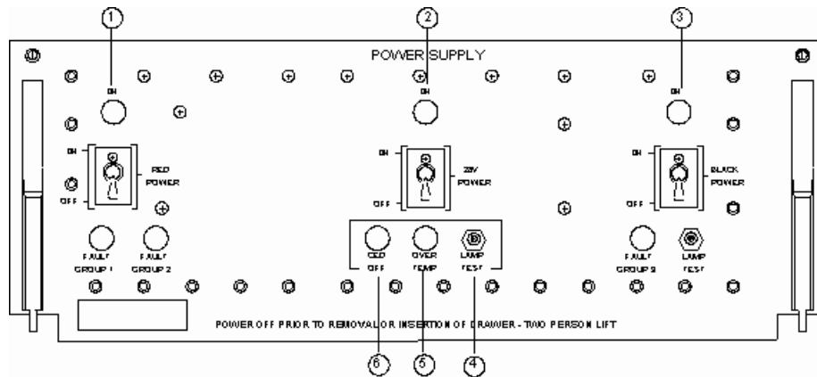
Figure 2.9. Power Supply.
