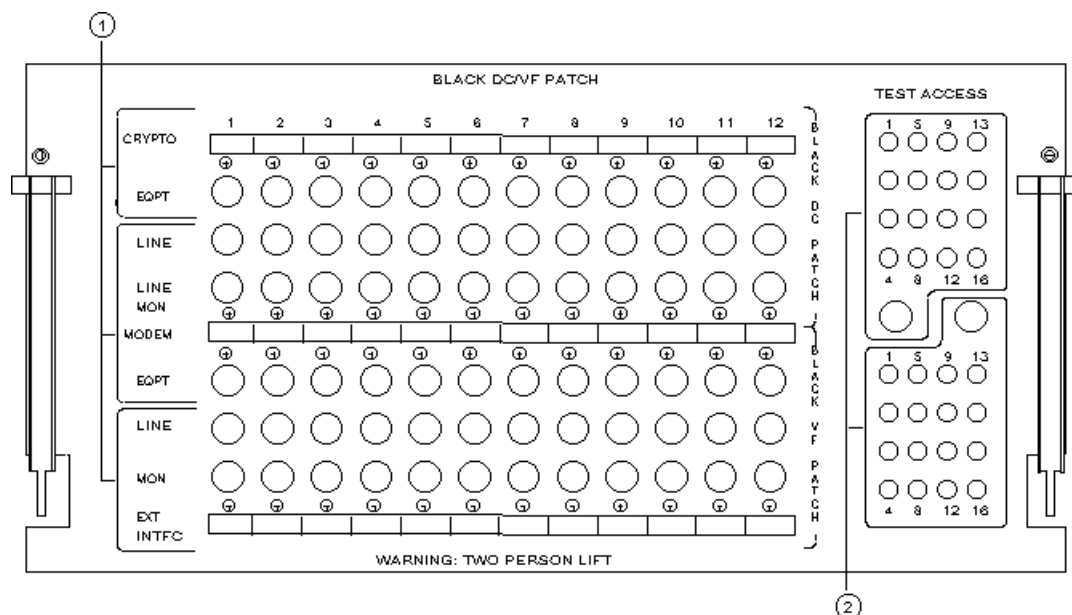
Figure 2.12. Black Patch Panel.
