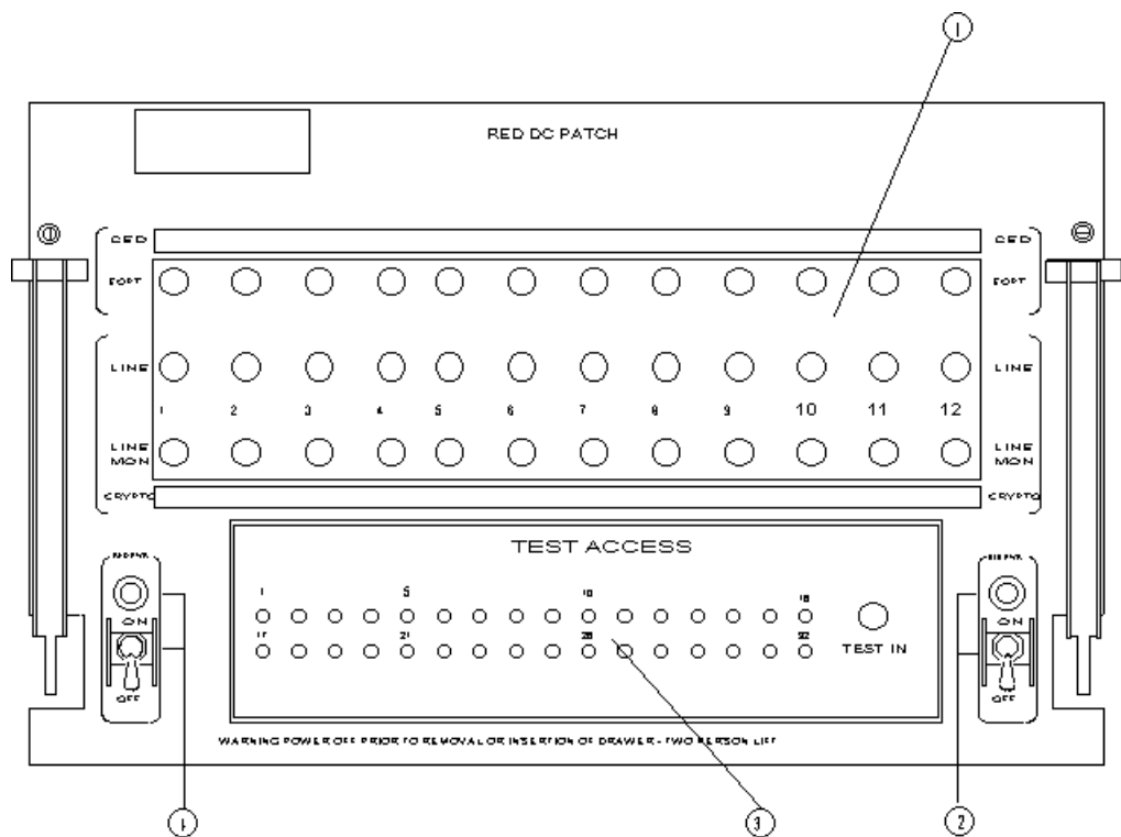
Figure 2.11. Red Patch Panel.
