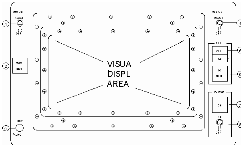
Figure 2.1. 24-Line VDU Display Area.
