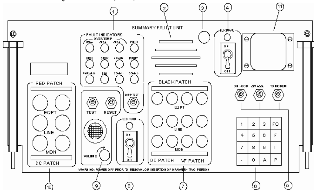
Figure 2.4. Summary Fault Unit (SFU).
