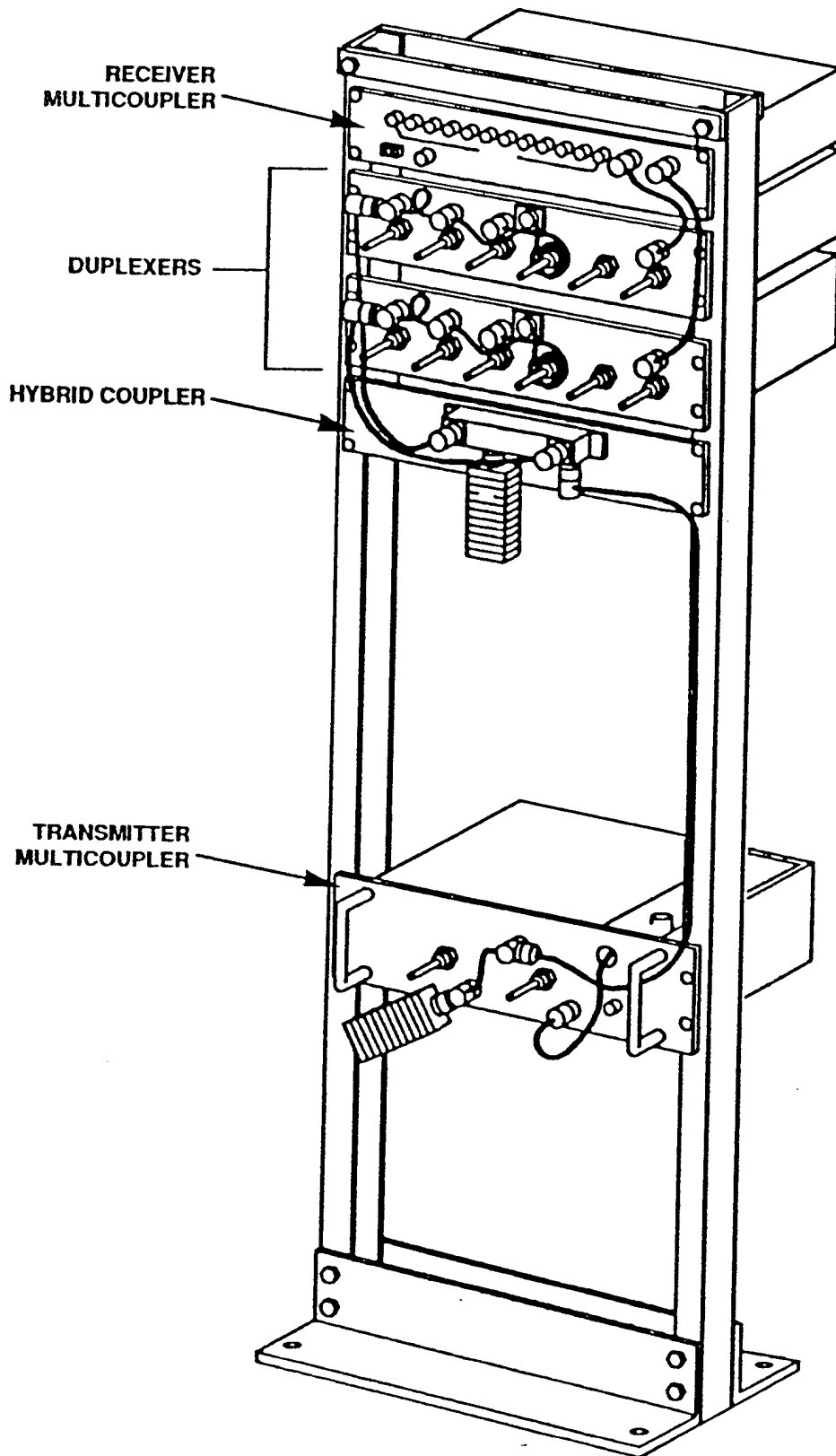
Figure 3. PVPCS Combined
