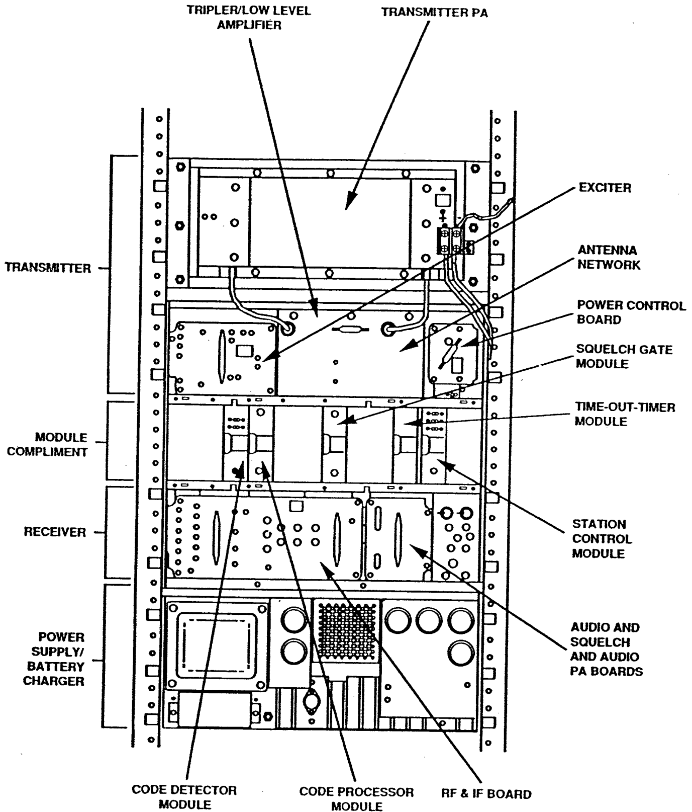
Figure 2. PVPCS Repeater
