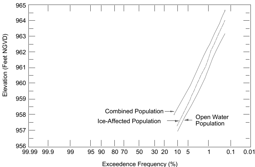
Figure 4. Stage-frequency curves for the Red River of the North at Wahpeton.
