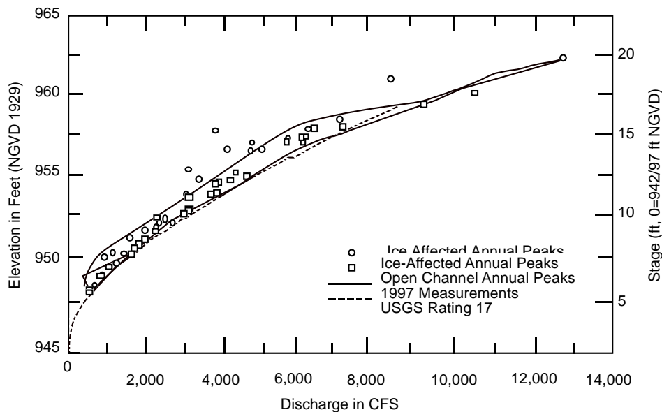
Figure 3. Elevation-discharge data for USGS Gage 05051500, Red River of the North at Wahpeton, North Dakota, showing ice-affected and annual peaks along with data for the 1997 event and the current rating curve (#17).
