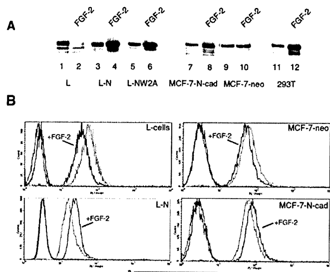
Figure 5. N-cadherin prevents FGF-2 induced FGFR downregulation resulting in chronic FGFR cell surface expression (A) Mouse L-cell fibroblasts (L, lanes 1-2) or L-cells stably transfected with N-cadherin (LN, lanes 3-4) or a non-adhesive N-cadherin mutant (LNW2A, lanes 5-6) were transiently transfected with FGFR-Flag and then treated for 18 hr with or without 100 ng/ml FGF-2 in the presence of 5 \mu g/ml Heparin. MCF-7-N-cad cells (lanes 7-8), MCF-7-neo (lanes 9-10), or 293T cells (lanes 11-12) were treated similarly. Cells were harvested and FGFR levels were determined by immunoblotting of cell extracts using anti-Flag antibodies. (B) Endogenous expression of cell surface-associated FGFR was analyzed by flow cytometry for the binding of an anti-FGFR-1 antibody. In each panel, the resulting histograms for anti-FGFR-1 staining from the FGF-2 treated cells were compared to those from untreated cells
