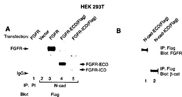
Figure 6 . N-cadherin and the FGFR interact exclusively via th extracellular domain. (A) Transfected Flag-tagged FGFR (lane 3) or FGFR-ECD (lane 4) but not FGFR-ICD (lane 5) co-precipitate with endogenous N-cadherin in HEK 293T.
