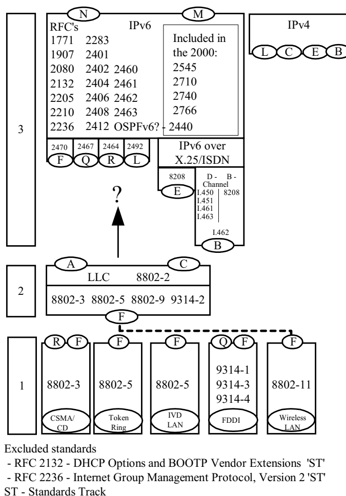
Figure 1. Functional IPv6 network profile
