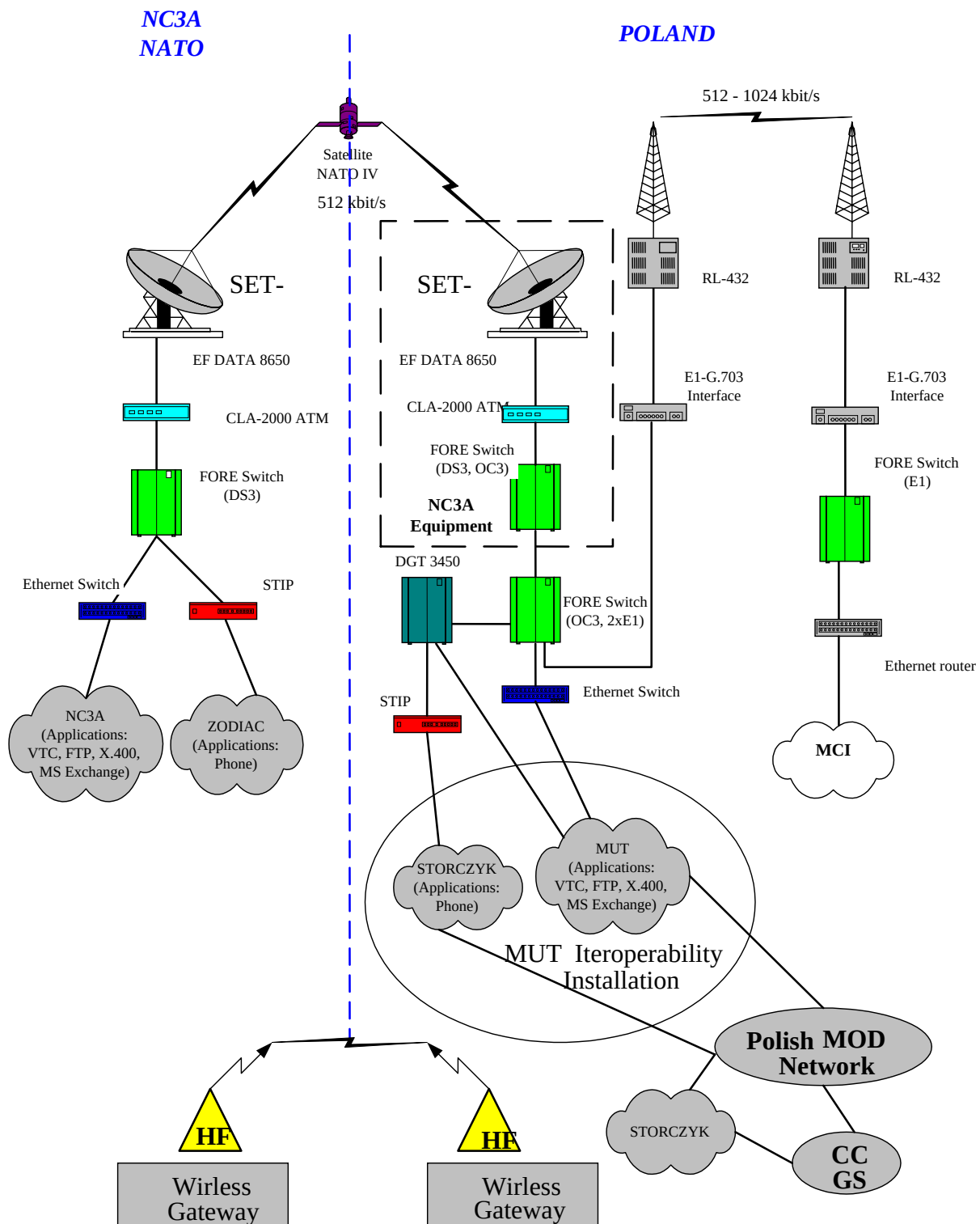
Figure 9. Configuration of MUT CSI demonstration
