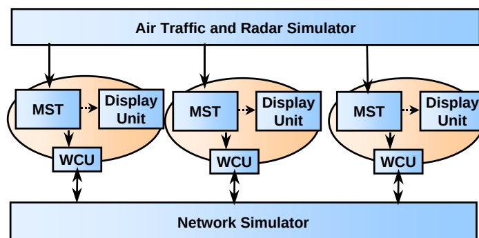
Figure 6. The WASP Prototype System
