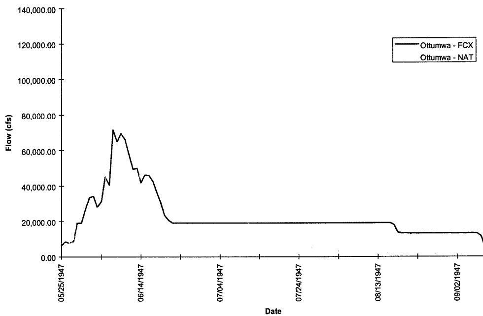
FIGURE D-2i. Ottumwa Hydrograph - Flood of 1947
