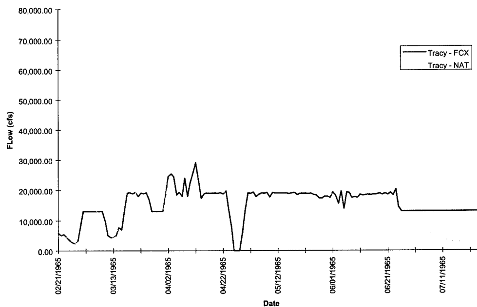
FIGURE D-4h. Tracy Hydrograph - Flood of 1965
