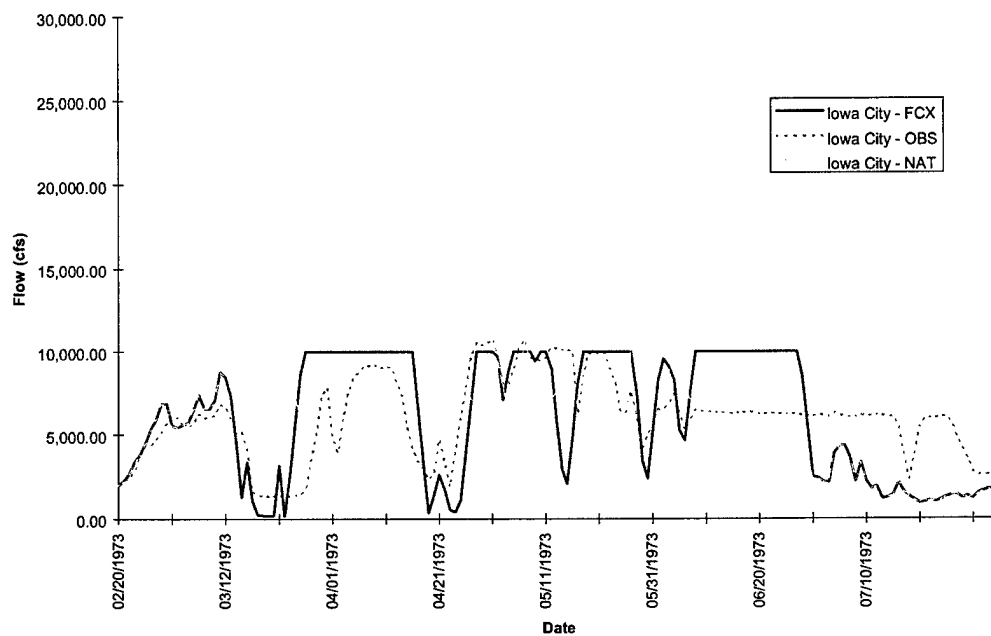
FIGURE D-5b. Iowa City Hydrograph - Flood of 1973
