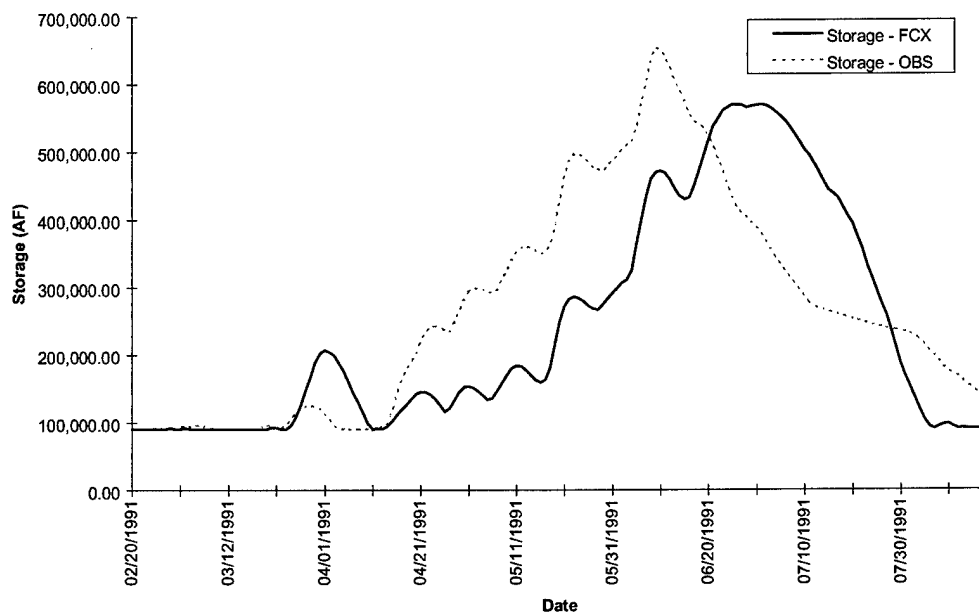
FIGURE D-9e. Saylorville Reservoir Storage - Flood of 1991
