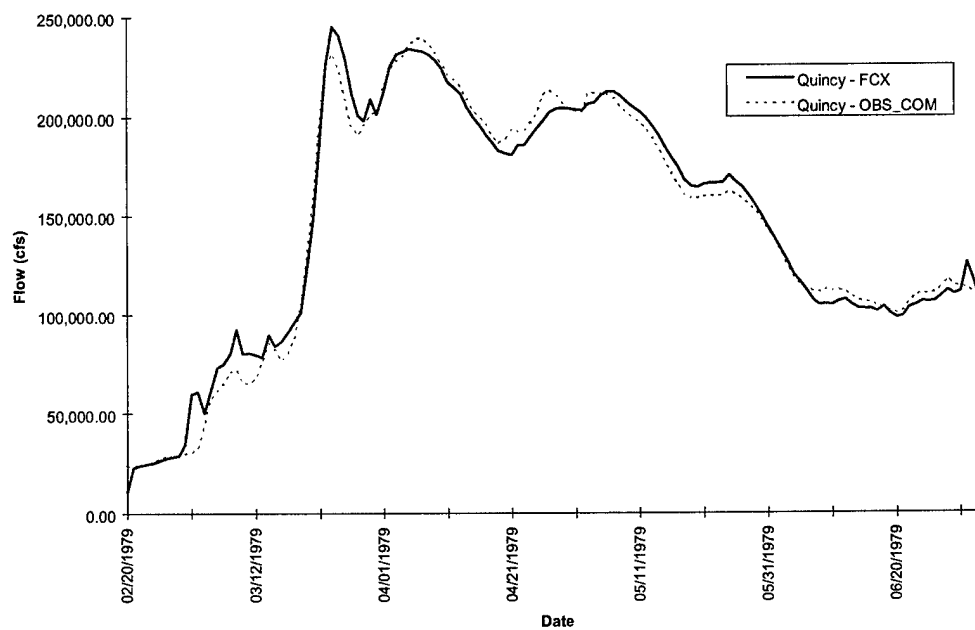
FIGURE D-7l. Quincy Hydrograph - Flood of 1979
