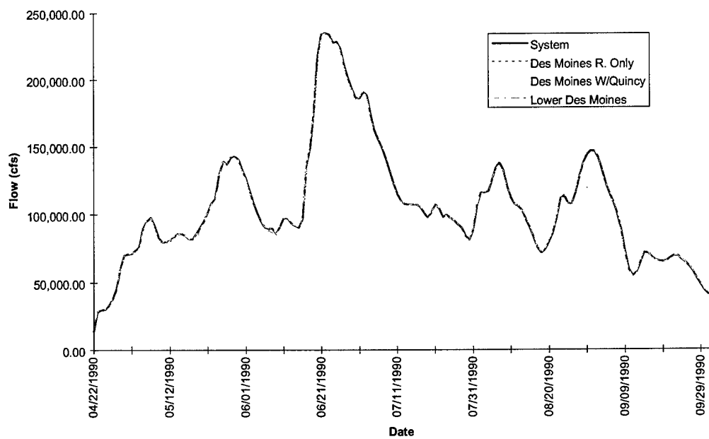
FIGURE E-80. Hydrograph of Model Results at Quincy - Flood of 1990
