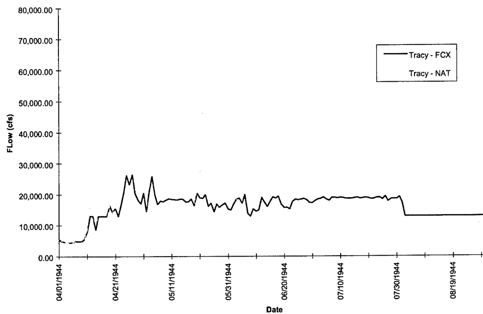
FIGURE D-1h. Tracy Hydrograph - Flood of 1944
