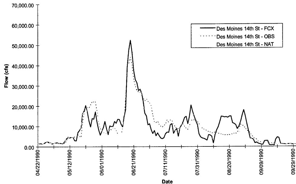
FIGURE D-8f. Des Moines 14 th Street - Flood of 1990
