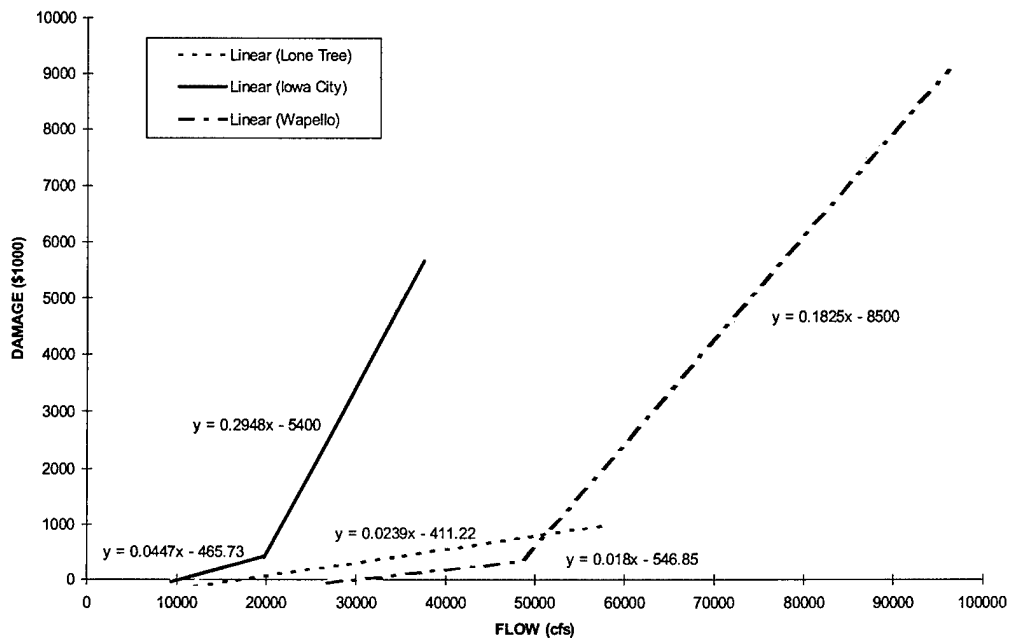
FIGURE 4-6 Iowa River Penalty Functions
