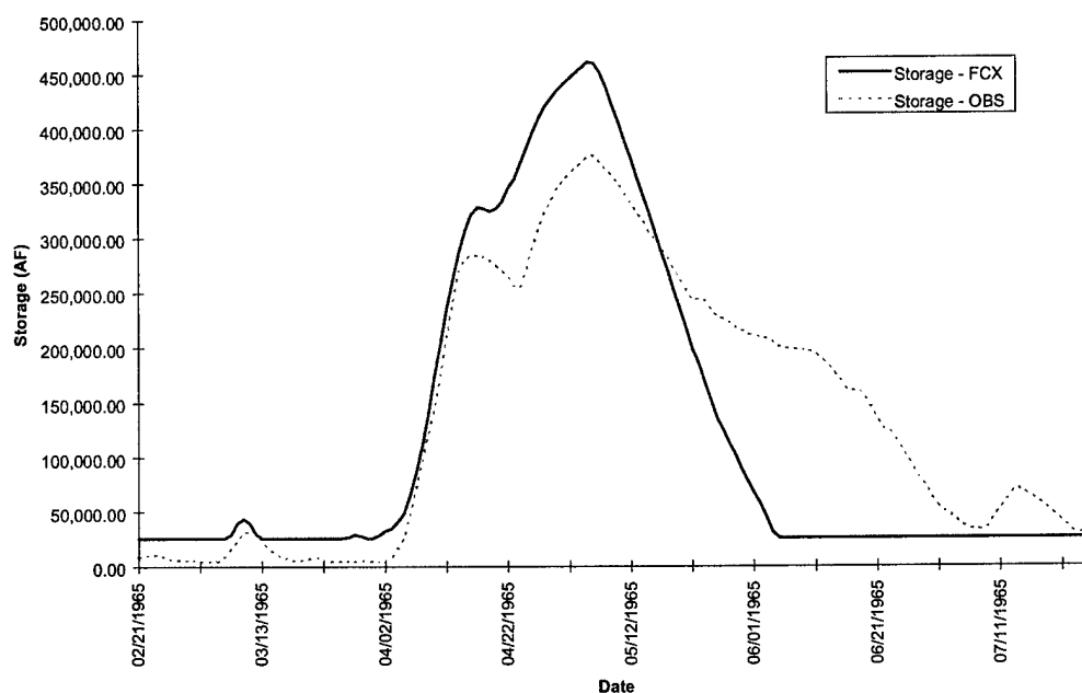
FIGURE D-4a. Coralville Reservoir Storage - Flood of 1965
