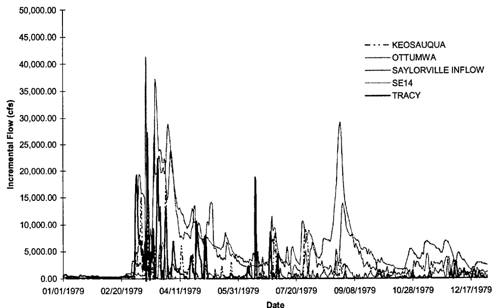
FIGURE C-14 Des Moines River Incremental Inflows - Flood of 1979
