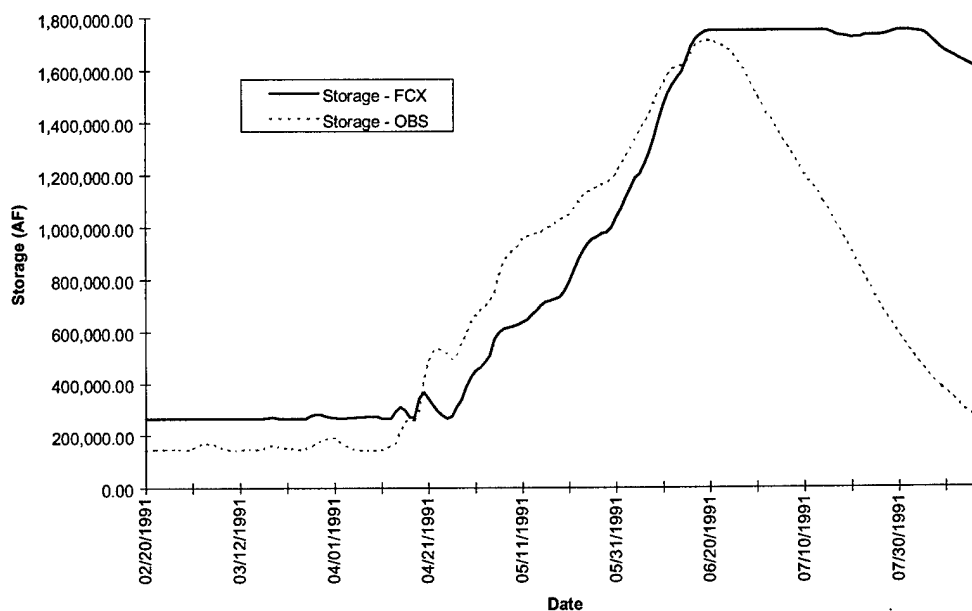
FIGURE D-9g. Lake Red Rock Storage - Flood of 1991
