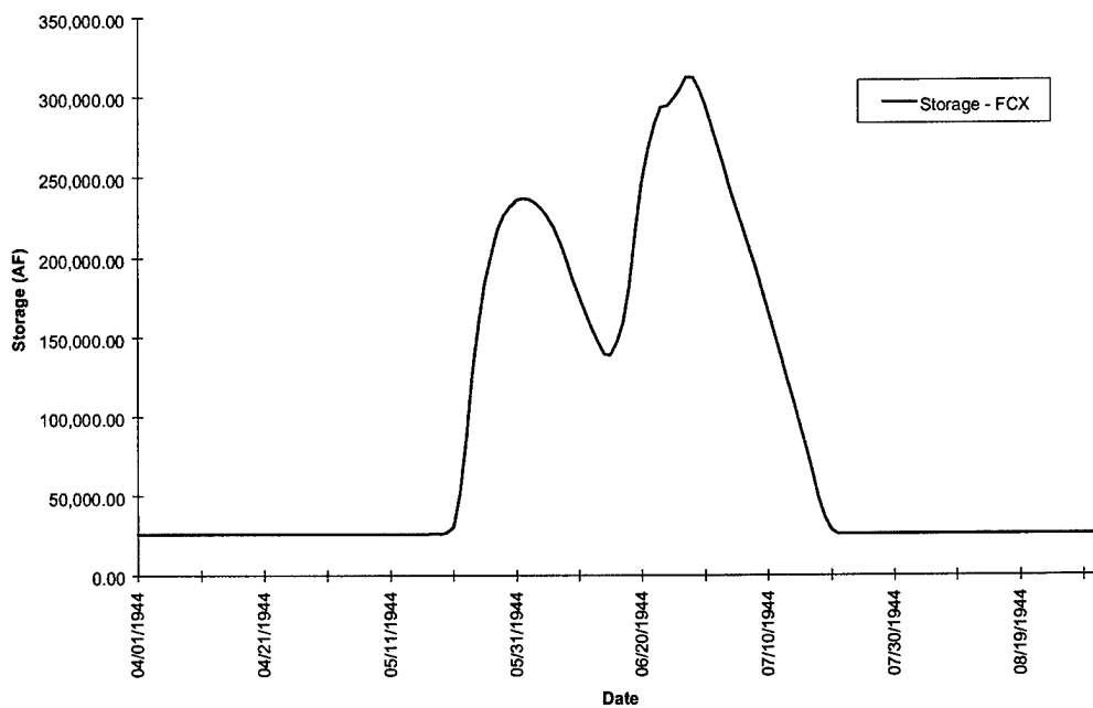
FIGURE D-1a. Coralville Reservoir Storage - Flood of 1944
