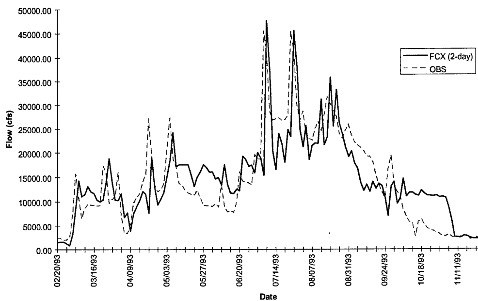
FIGURE D-10c. Lone Tree Hydrograph - Flood of 1993
