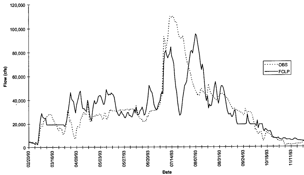
FIGURE 5-10 Ottumwa Hydrograph - Flood of 1993
