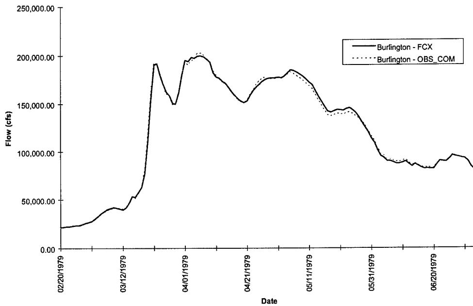
FIGURE D-7k. Burlington Hydrograph - Flood of 1979
