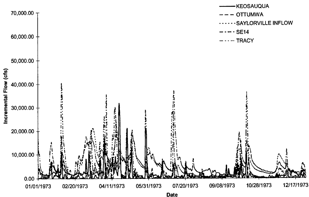
FIGURE C-10 Des Moines River Incremental Inflows - Flood of 1973
