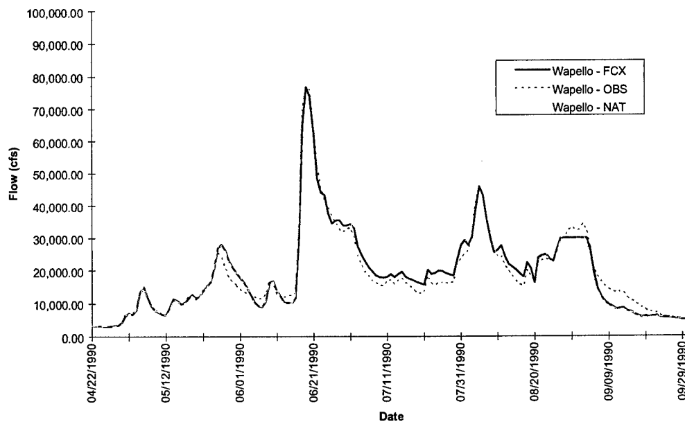
FIGURE D-8d. Wapello Hydrograph - Flood of 1990
