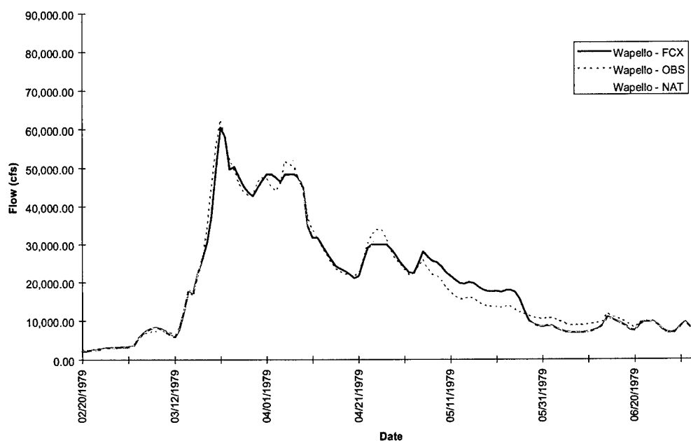
FIGURE D-7d. Wapello Hydrograph - Flood of 1979
