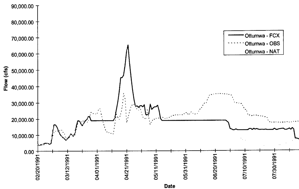
FIGURE D-9i. Ottumwa Hydrograph - Flood of 1991
