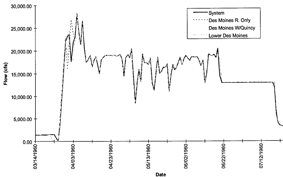
FIGURE E-3k. Hydrograph of Model Results at Tracy - Flood of 1960
