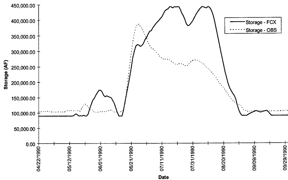
FIGURE D-8e. Saylorville Reservoir Storage - Flood of 1990
