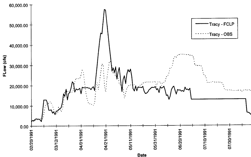
FIGURE 4-11 Hydrograph at Tracy - Flood of 1991
