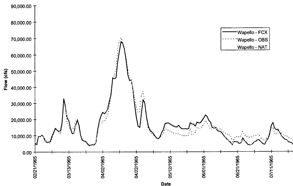
FIGURE D-4d. Wapello Hydrograph - Flood of 1965
