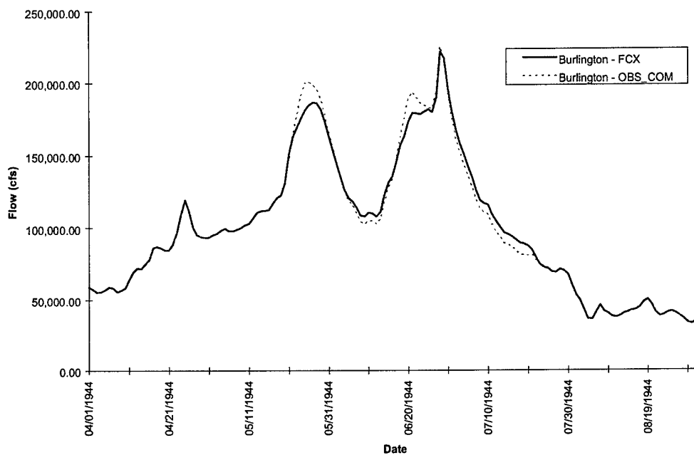
FIGURE D-1k. Burlington Hydrograph - Flood of 1944
