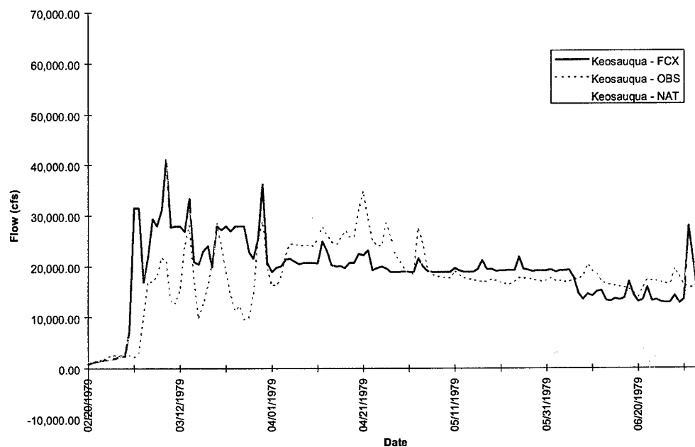
FIGURE D-7j. Keosauqua Hydrograph - Flood of 1979
