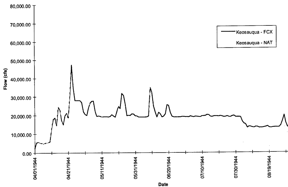
FIGURE D-1j. Keosauqua Hydrograph - Flood of 1944
