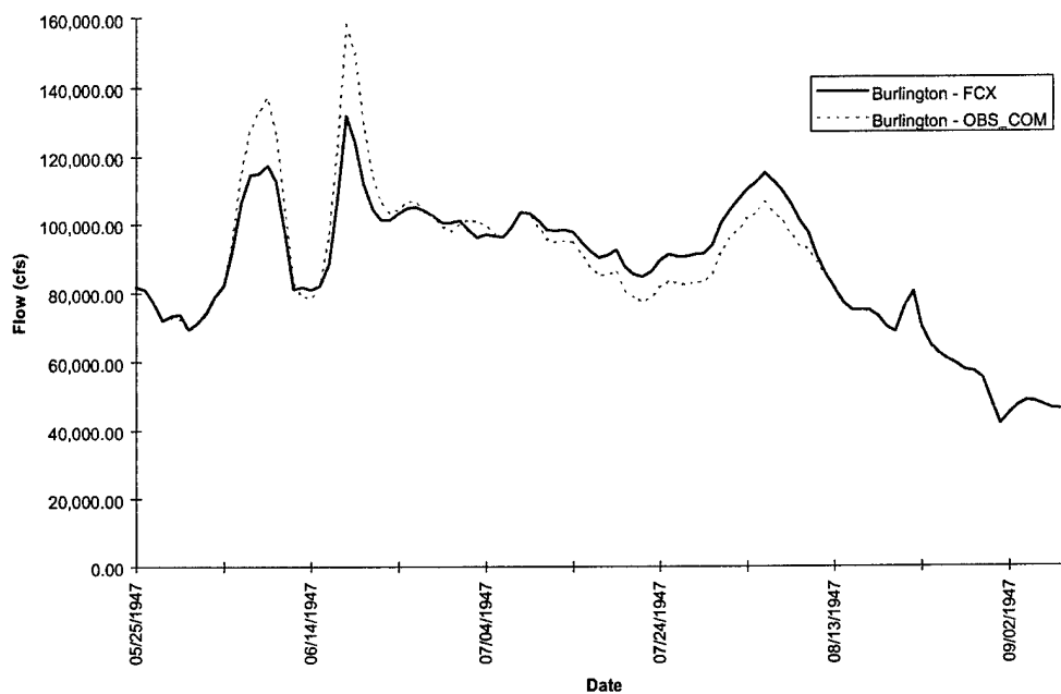
FIGURE D-2k. Burlington Hydrograph - Flood of 1947
