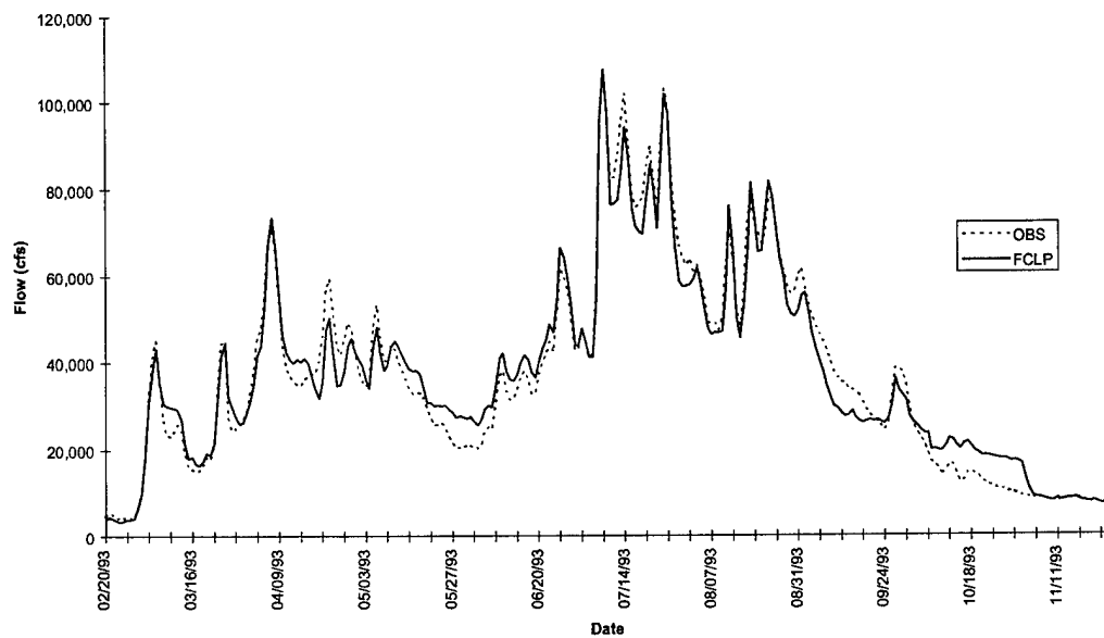
FIGURE 5-4 Wapello Hydrograph - Flood of 1993
