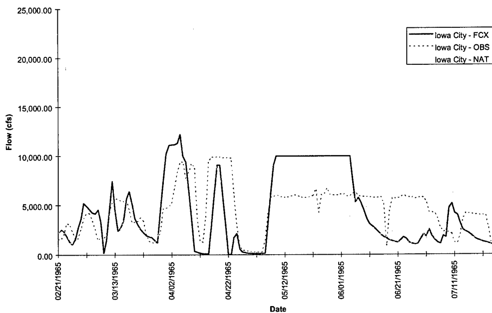
FIGURE D-4b. Iowa City Hydrograph - Flood of 1965
