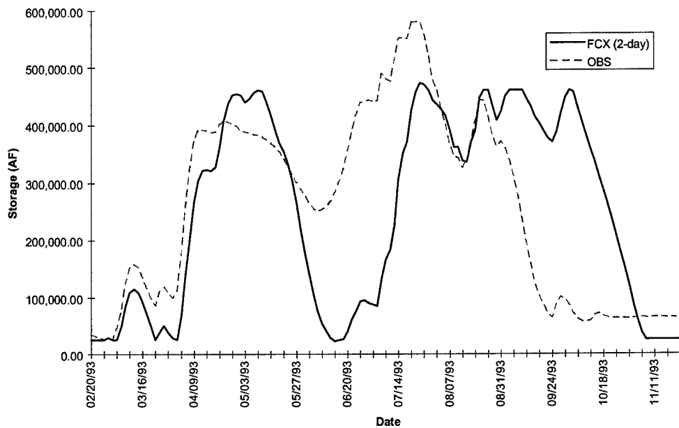
FIGURE D-10a. Coralville Reservoir Storage - Flood of 1993
