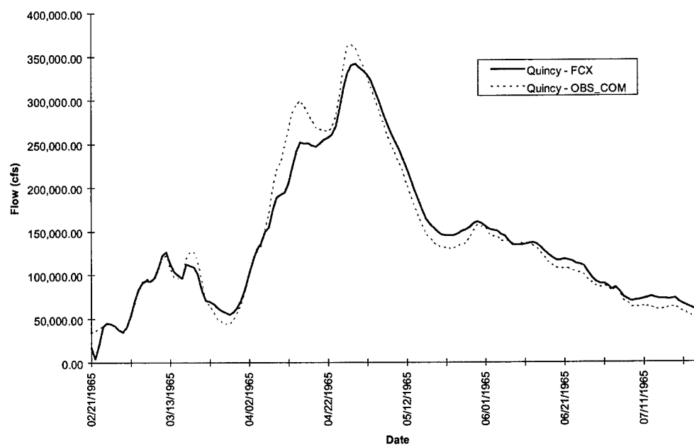
FIGURE D-4l. Quincy Hydrograph - Flood of 1965
