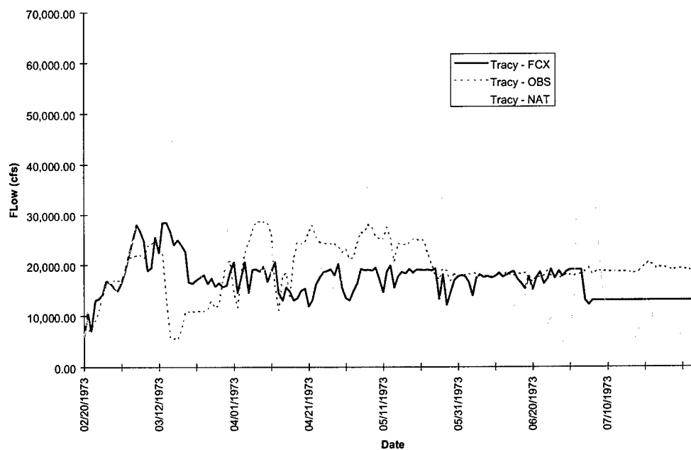
FIGURE D-5h. Tracy Hydrograph - Flood of 1973
