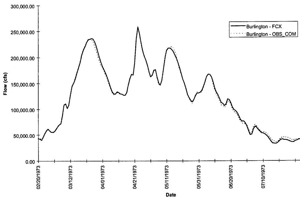
FIGURE D-5k. Burlington Hydrograph - Flood of 1973
