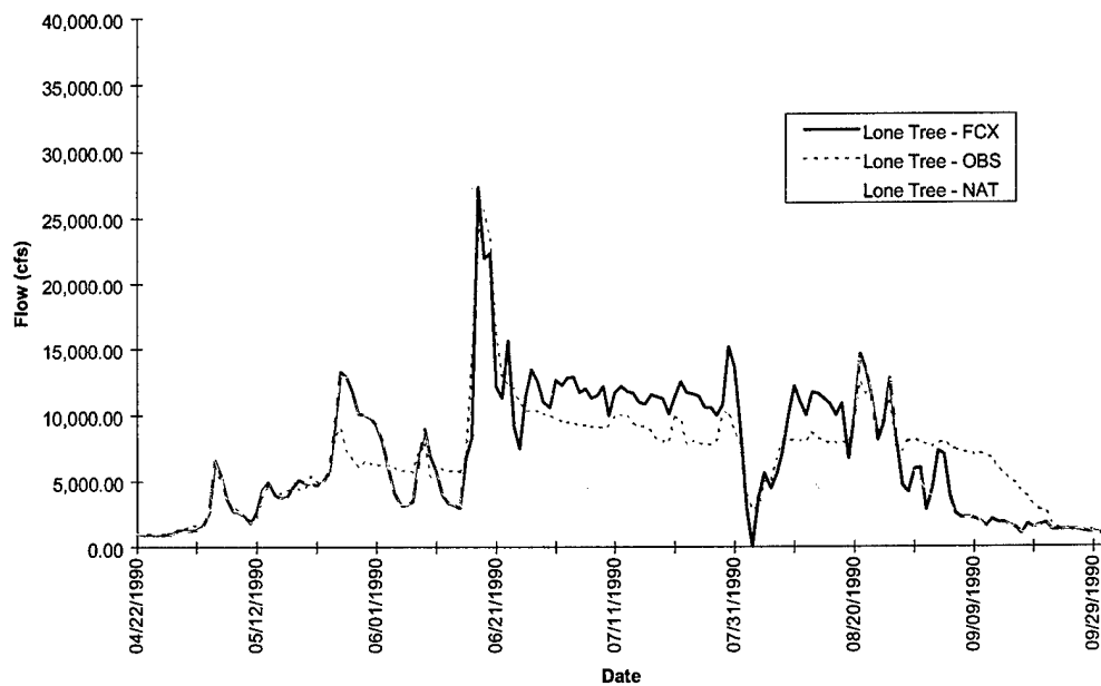
FIGURE D-8c. Lone Tree Hydrograph - Flood of 1990
