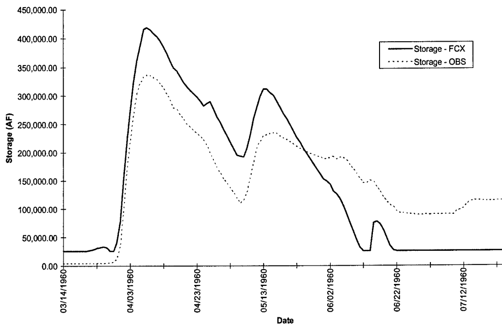
FIGURE D-3a. Coralville Reservoir Storage - Flood of 1960
