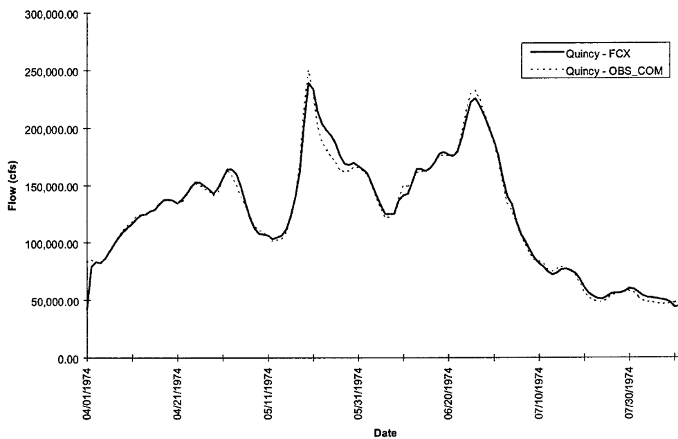
FIGURE D-6l. Quincy Hydrograph - Flood of 1974
