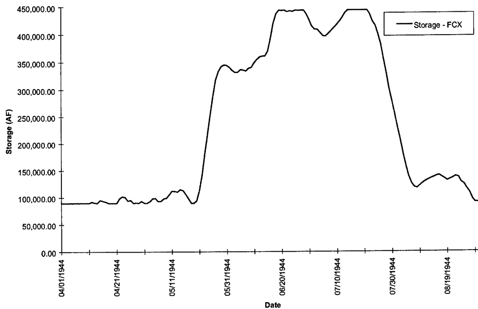
FIGURE D-1e. Saylorville Reservoir Storage - Flood of 1944
