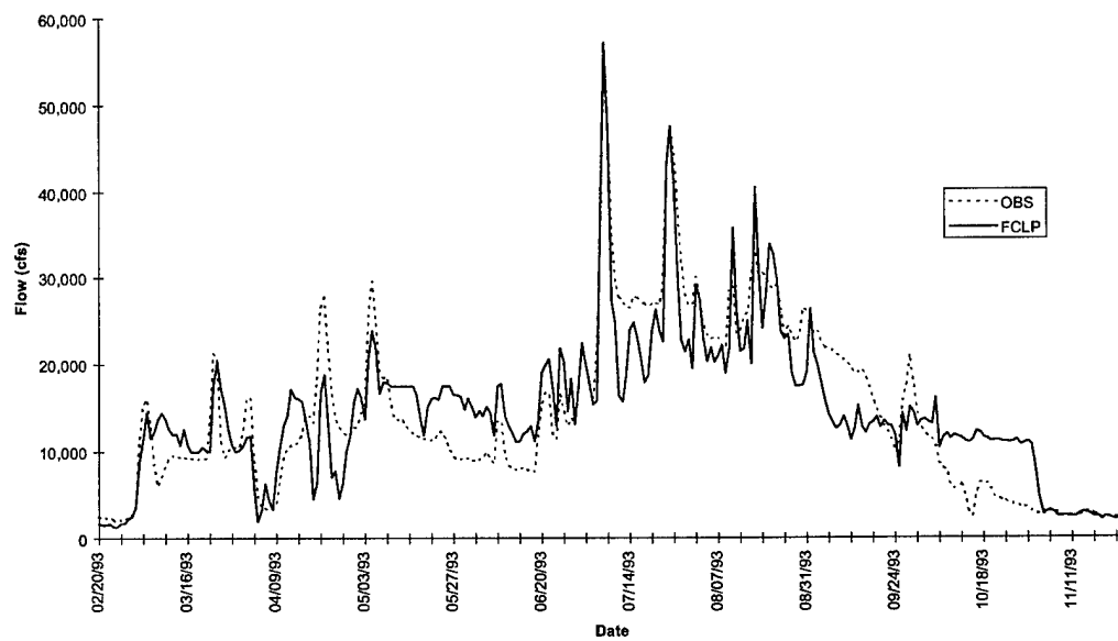
FIGURE 5-3 Lone Tree Hydrograph - Flood of 1993
