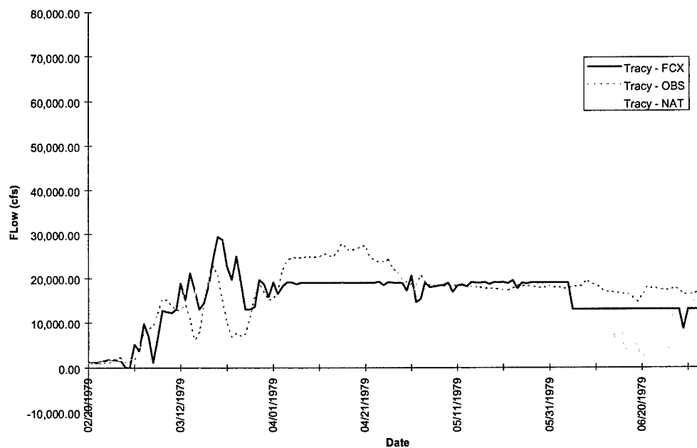
FIGURE D-7h. Tracy Hydrograph - Flood of 1979
