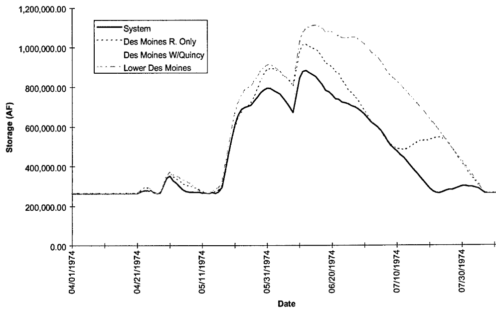
FIGURE E-6i. Model Results of Lake Red Rock Storage - Flood of 1974
