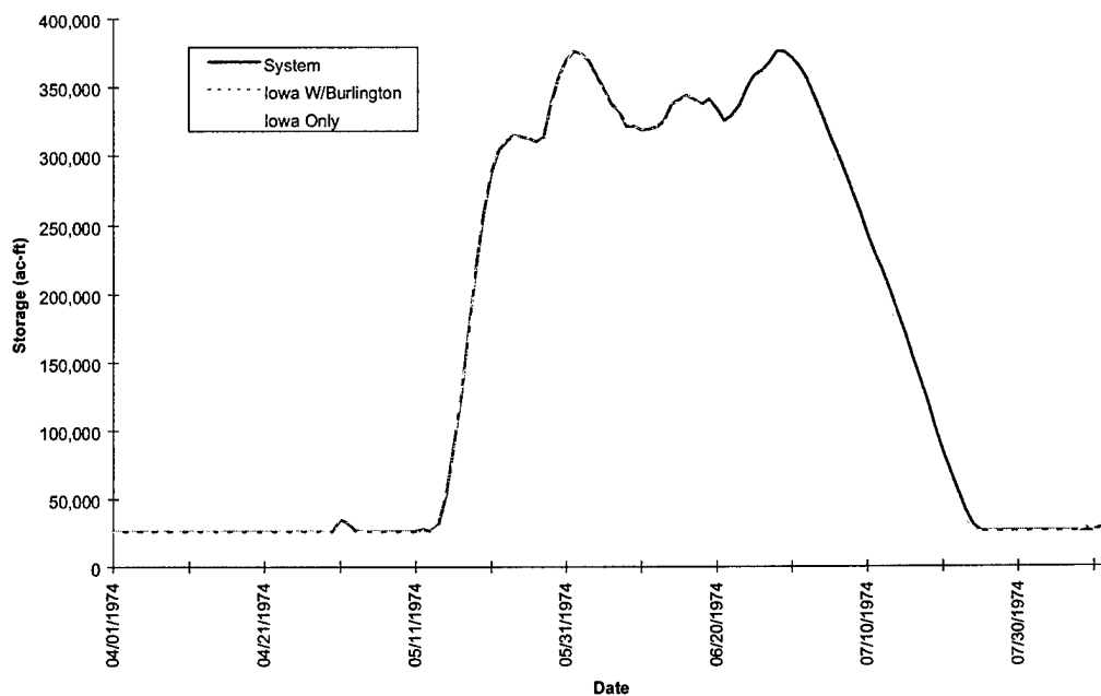
FIGURE E-6a. Model Results of Coralville Reservoir Storage - Flood of 1974
