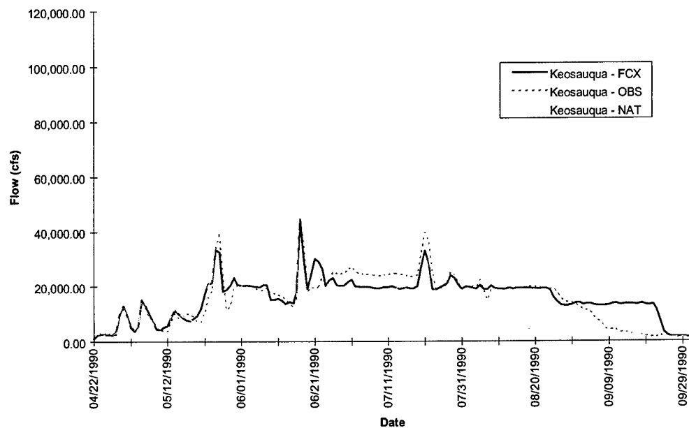
FIGURE D-8j. Keosauqua Hydrograph - Flood of 1990
