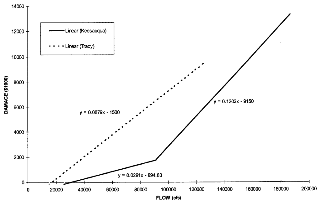
FIGURE 4-8 Des Moines River Penalty Functions
