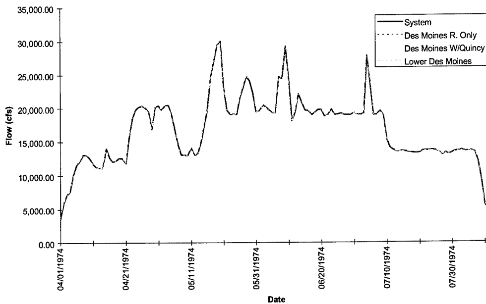
FIGURE E-6m. Hydrograph of Model Results at Keosauqua - Flood of 1974
