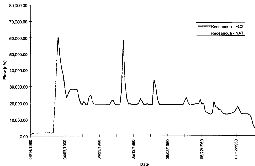
FIGURE D-3j. Keosauqua Hydrograph - Flood of 1960
