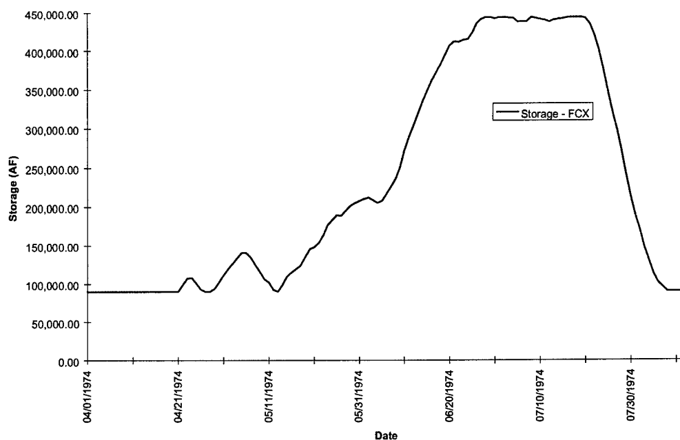
FIGURE D-6e. Saylorville Reservoir Storage - Flood of 1974
