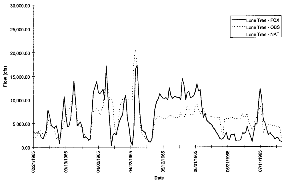
FIGURE D-4c. Lone Tree Hydrograph - Flood of 1965
