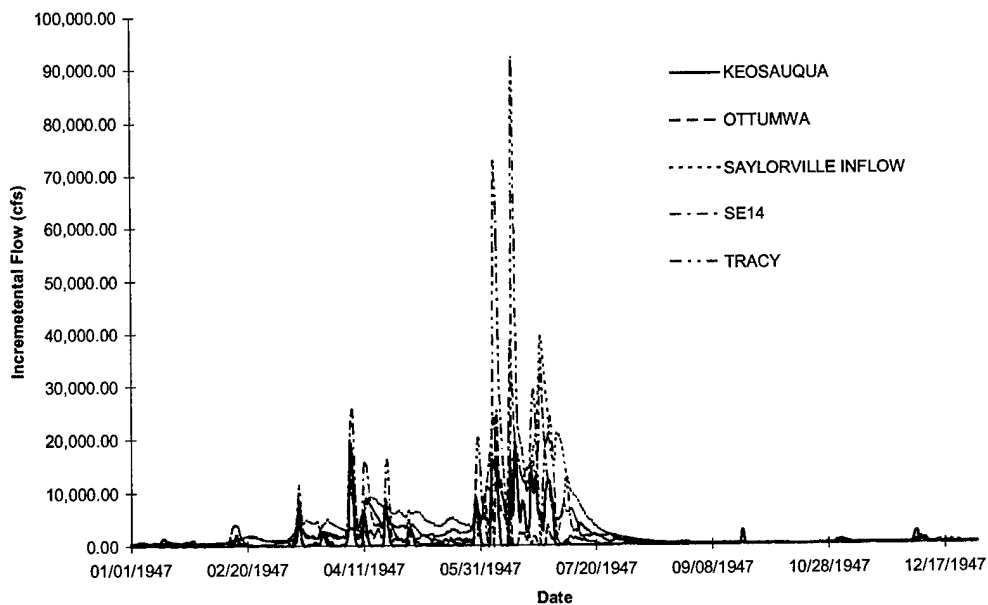
FIGURE C-4 Des Moines River Incremental Inflows - Flood of 1947
