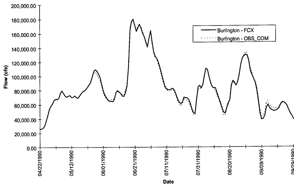
FIGURE D-8k. Burlington Hydrograph - Flood of 1990
