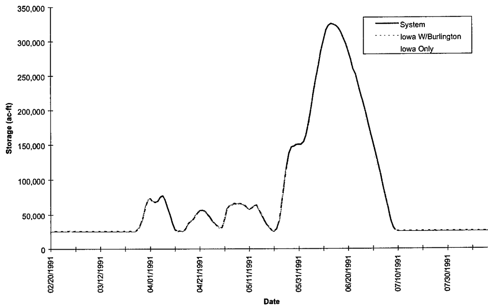
FIGURE E-9a. Model Results of Coralville Reservoir Storage - Flood of 1991
