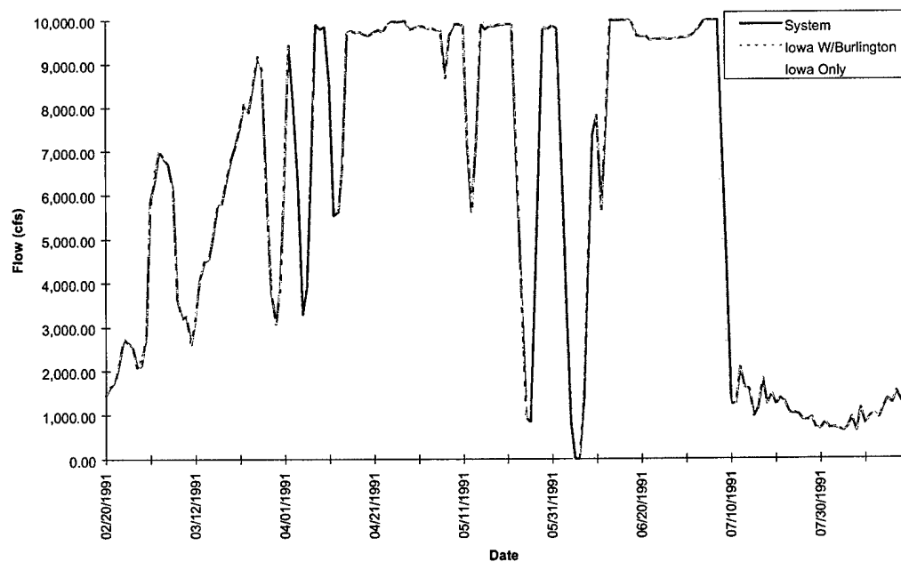
FIGURE E-9b. Model Results of Coralville Reservoir Release - Flood of 1991
