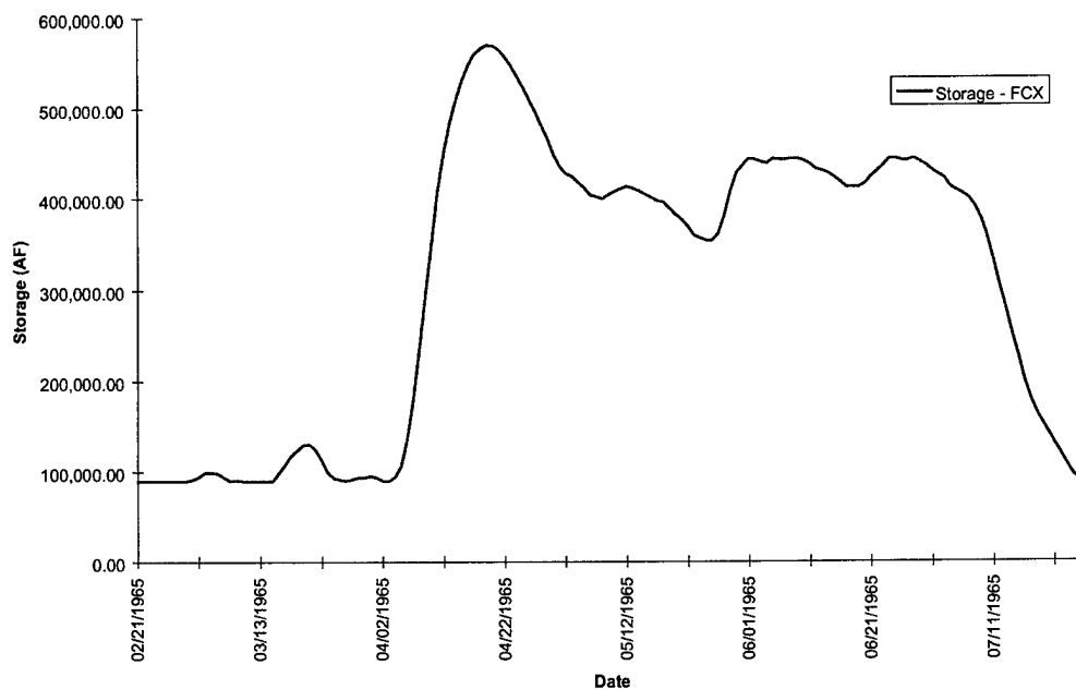
FIGURE D-4e. Saylorville Reservoir Storage - Flood of 1965
