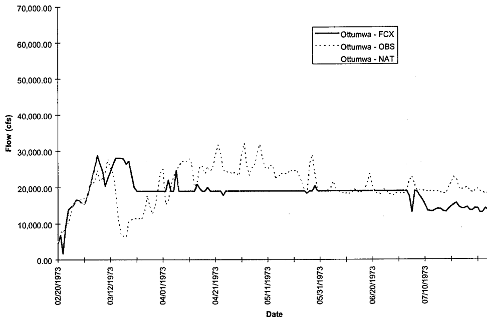
FIGURE D-5i. Ottumwa Hydrograph - Flood of 1973
