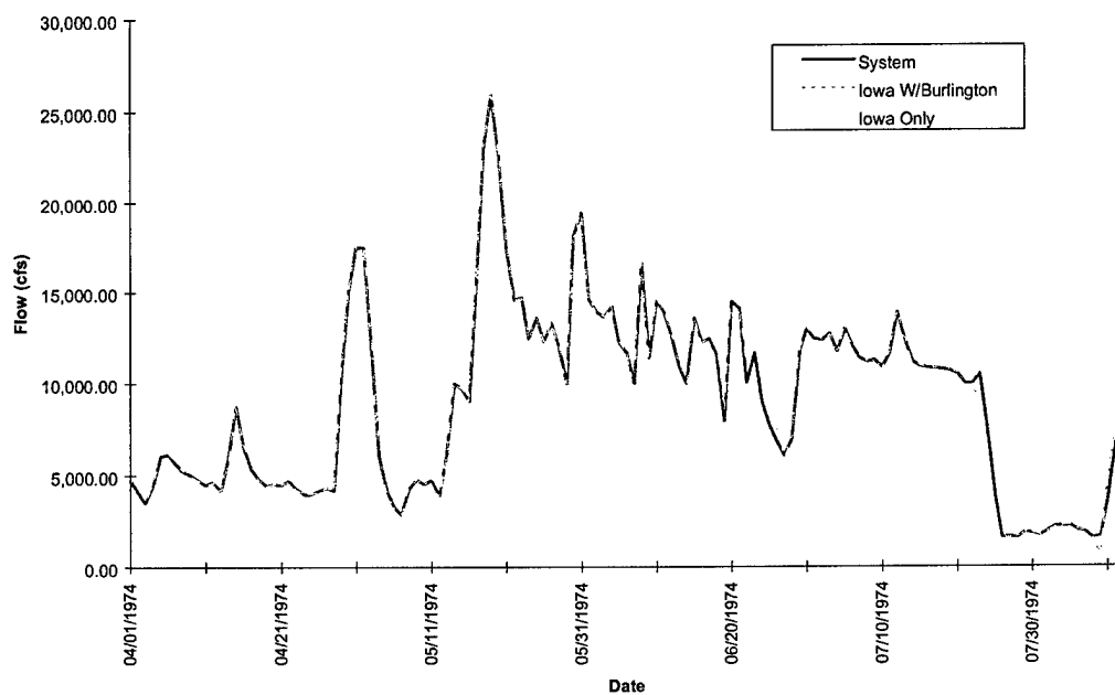
FIGURE E-6d. Hydrograph of Model Results at Lone Tree - Flood of 1974
