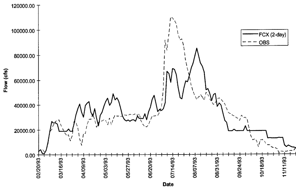
FIGURE D-10i. Ottumwa Hydrograph - Flood of 1993
