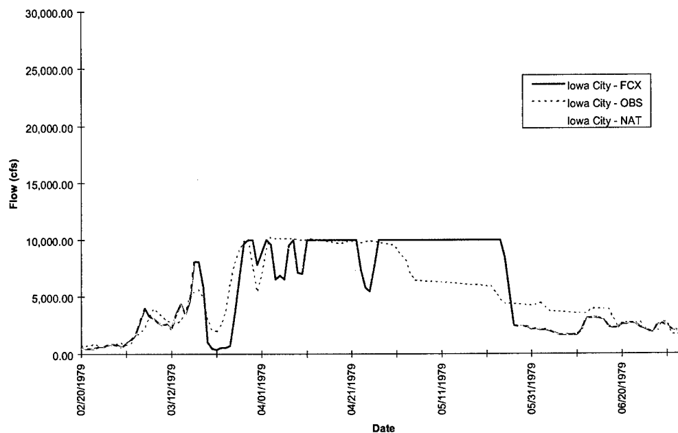
FIGURE D-7b. Iowa City Hydrograph - Flood of 1979
