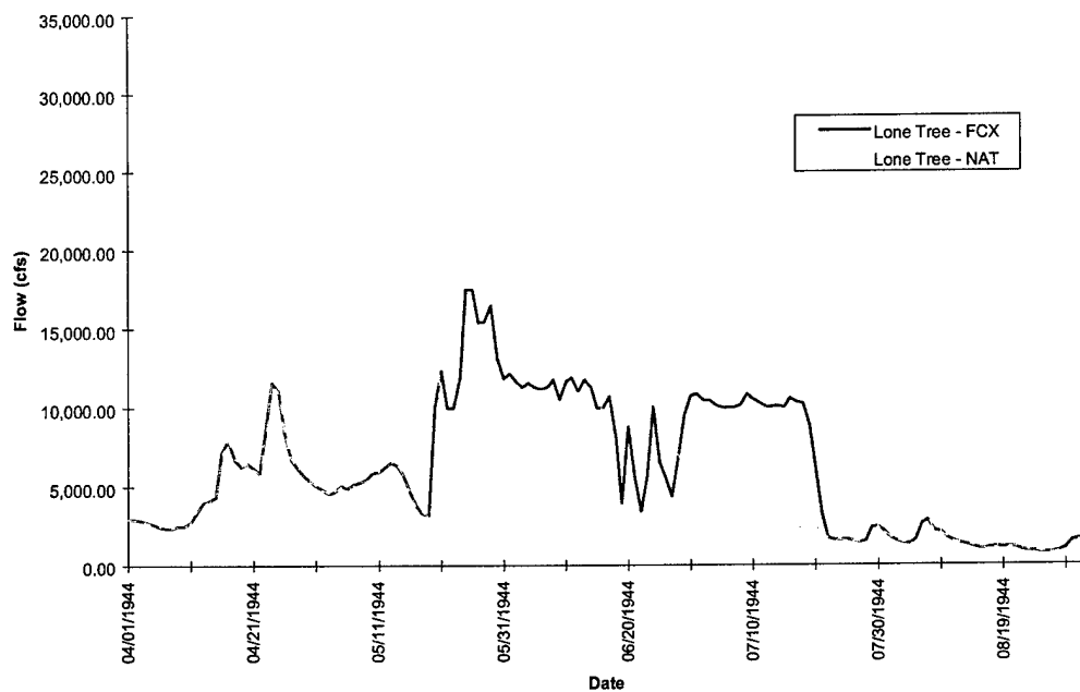
FIGURE D-1c. Lone Tree Hydrograph - Flood of 1944
