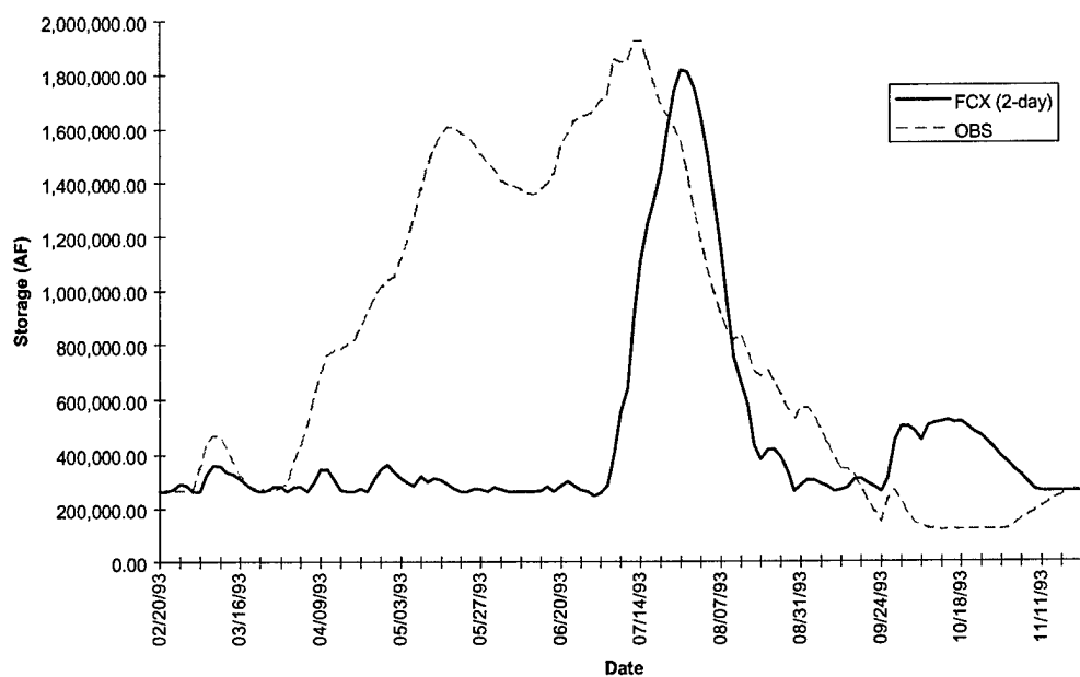
FIGURE D-10g. Lake Red Rock Storage - Flood of 1993
