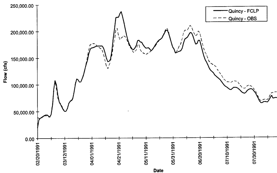
FIGURE 4-12 Hydrograph at Quincy - Flood of 1991
