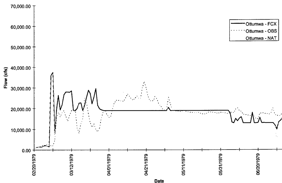
FIGURE D-7i. Ottumwa Hydrograph - Flood of 1979
