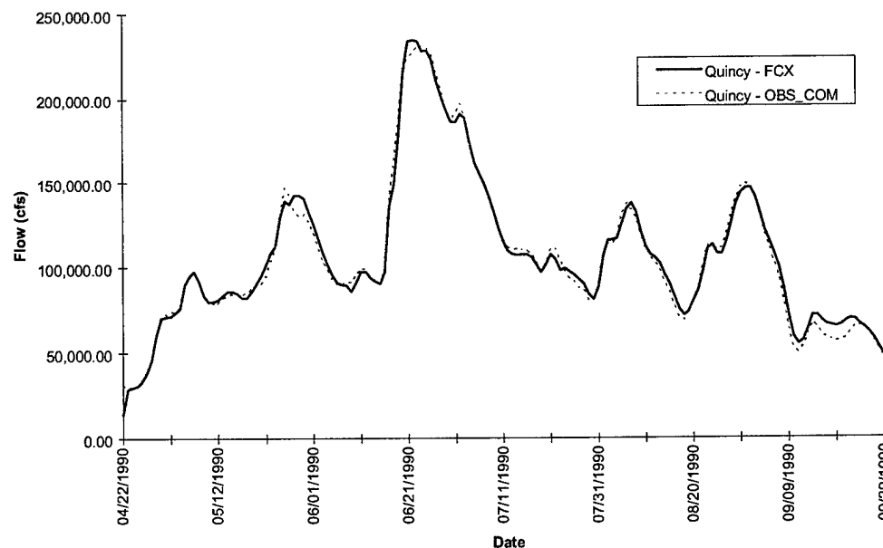
FIGURE D-8l. Quincy Hydrograph - Flood of 1990
