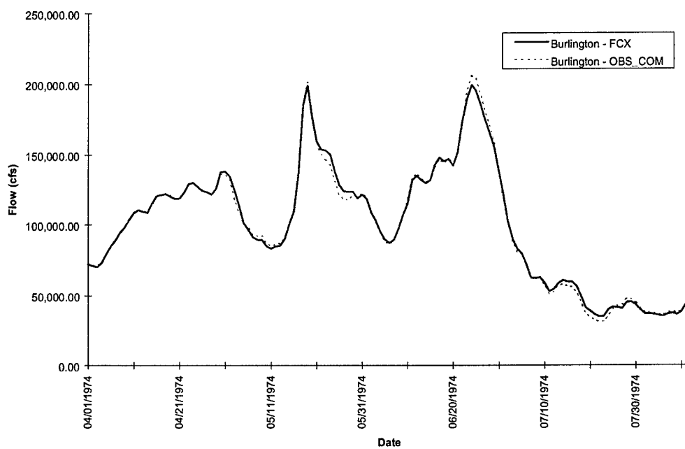
FIGURE D-6k. Burlington Hydrograph - Flood of 1974
