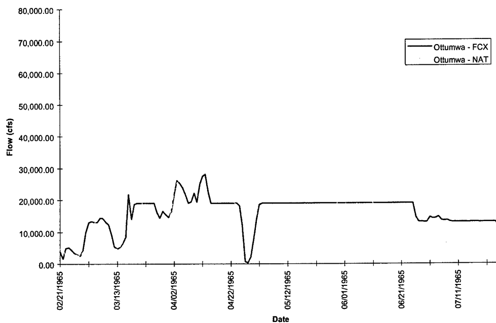
FIGURE D-4i. Ottumwa Hydrograph - Flood of 1965
