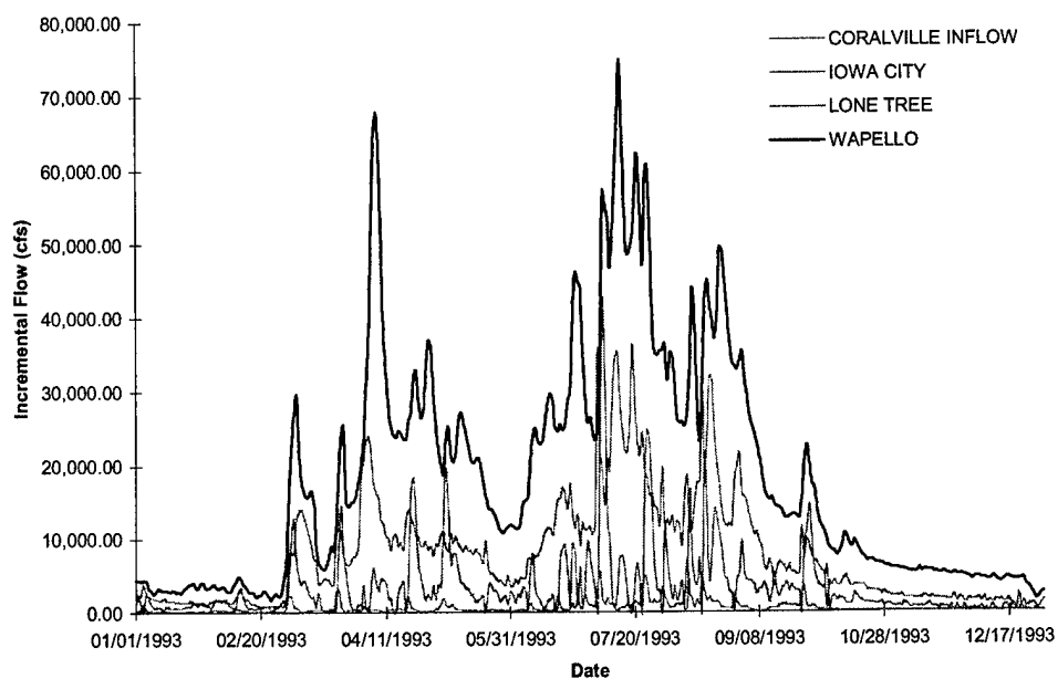
FIGURE C-19 Iowa River Incremental Inflows - Flood of 1993
