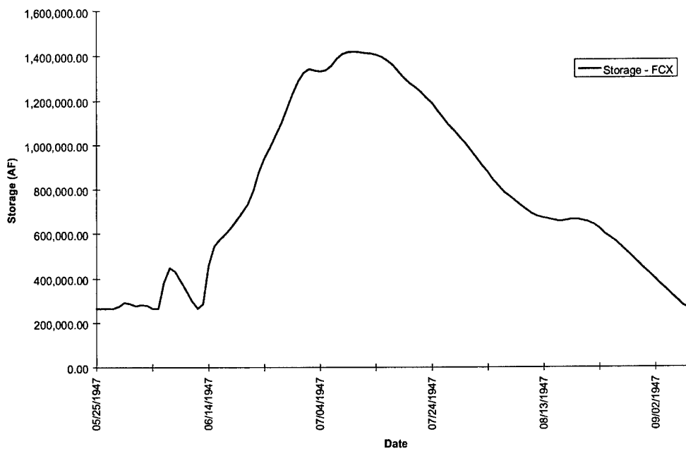
FIGURE D-2g. Lake Red Rock Storage - Flood of 1947
