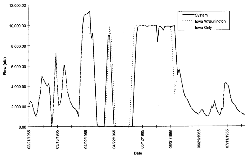
FIGURE E-4b. Model Results of Coralville Reservoir Release - Flood of 1965
