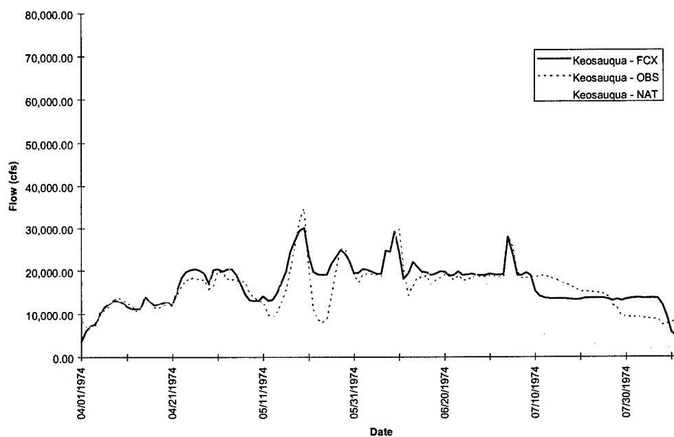
FIGURE D-6j. Keosauqua Hydrograph - Flood of 1974
