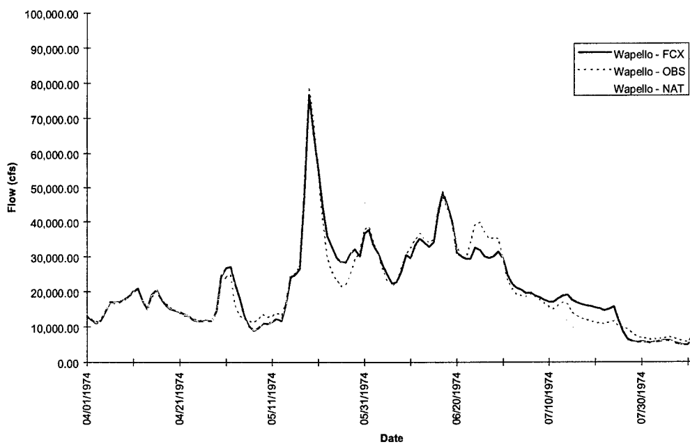
FIGURE D-6d. Wapello Hydrograph - Flood of 1974
