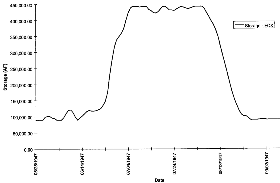
FIGURE D-2e. Saylorville Reservoir Storage - Flood of 1947
