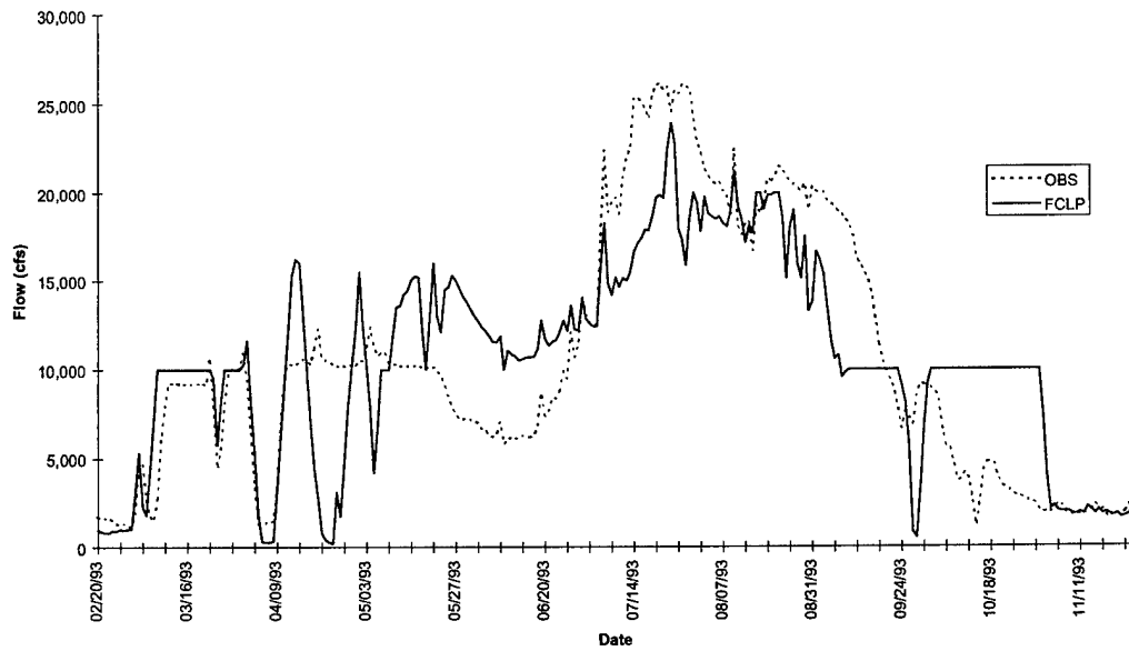
FIGURE 5-2 Iowa City Hydrograph - Flood of 1993
