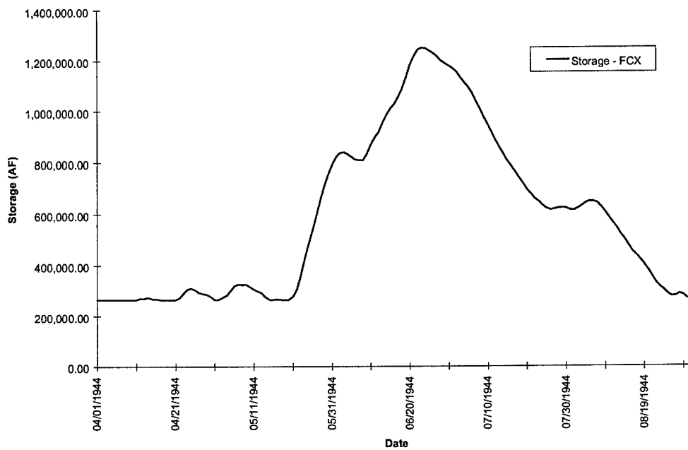
FIGURE D-1g. Lake Red Rock Storage - Flood of 1944
