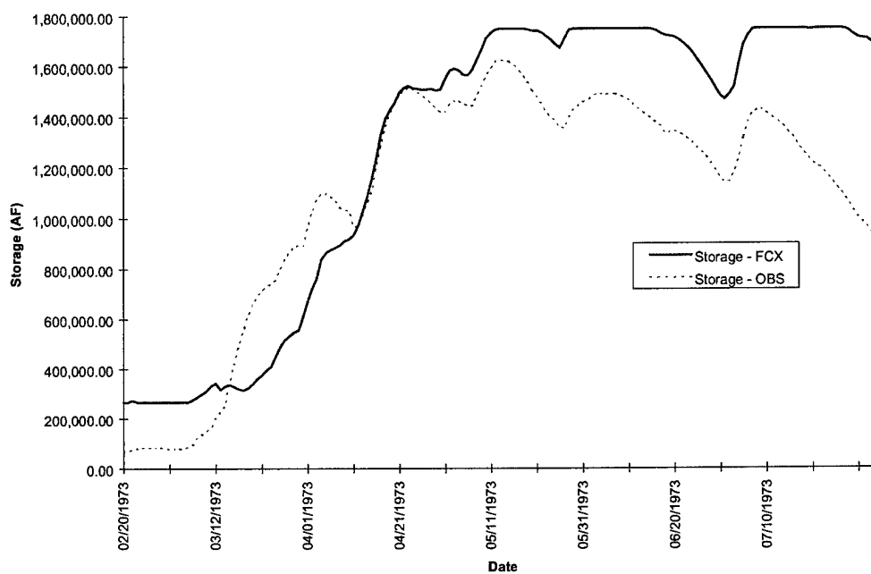
FIGURE D-5g. Lake Red Rock Storage - Flood of 1973
