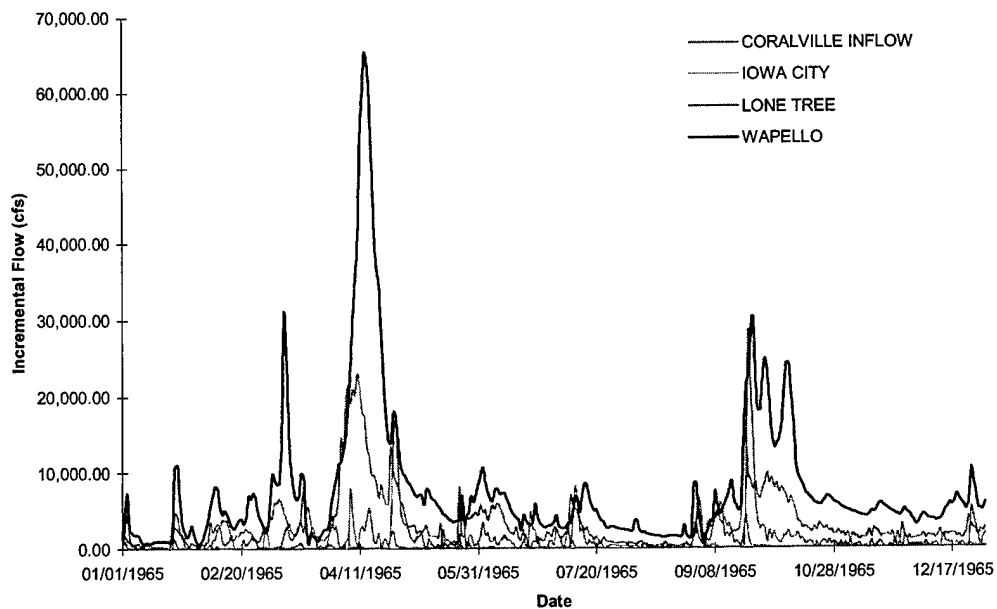
FIGURE C-7 Iowa River Incremental Inflows - Flood of 1965
