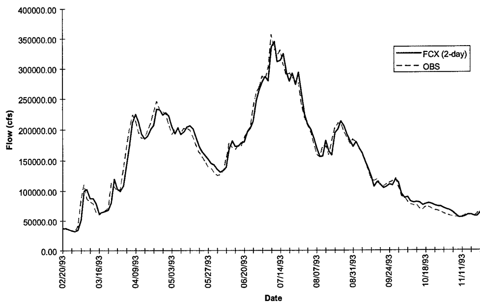
FIGURE D-10k. Burlington Hydrograph - Flood of 1993
