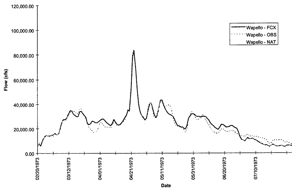
FIGURE D-5d. Wapello Hydrograph - Flood of 1973
