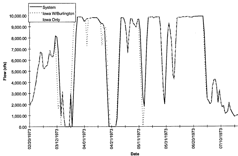
FIGURE E-5b. Model Results of Coralville Reservoir Release - Flood of 1973
