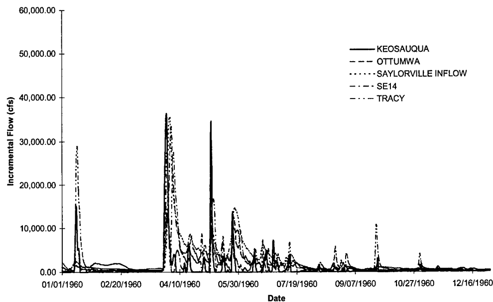
FIGURE C-6 Des Moines River Incremental Inflows - Flood of 1960
