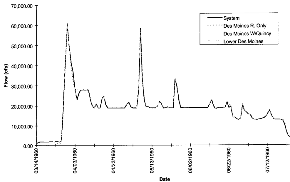
FIGURE E-3m. Hydrograph of Model Results at Keosauqua - Flood of 1960
