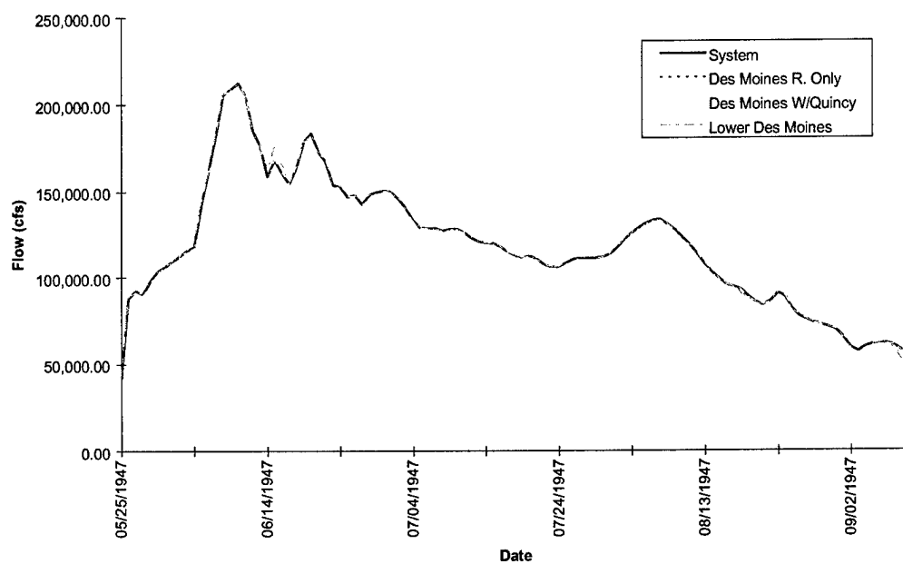
FIGURE E-2o. Hydrograph of Model Results at Quincy - Flood of 1947
