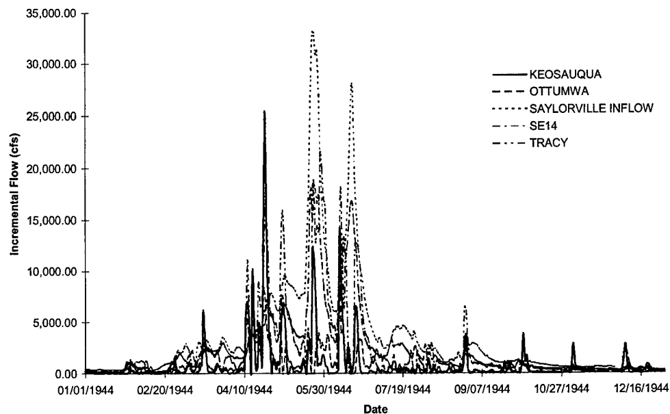
FIGURE C-2 Des Moines River Incremental Inflows - Flood of 1944
