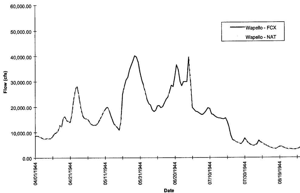
FIGURE D-1d. Wapello Hydrograph - Flood of 1944
