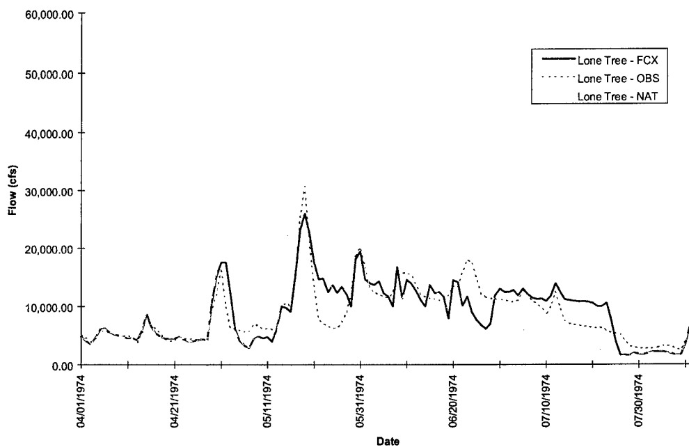
FIGURE D-6c. Lone Tree Hydrograph - Flood of 1974
