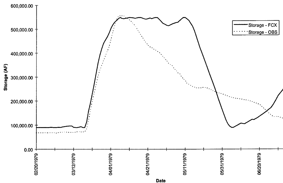
FIGURE D-7e. Saylorville Reservoir Storage - Flood of 1979
