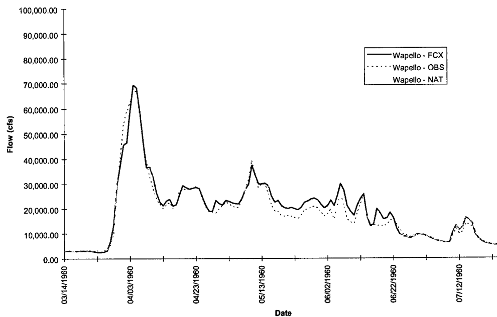
FIGURE D-3d. Wapello Hydrograph - Flood of 1960
