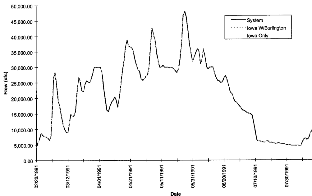
FIGURE E-9e. Hydrograph of Model Results at Wapello - Flood of 1991
