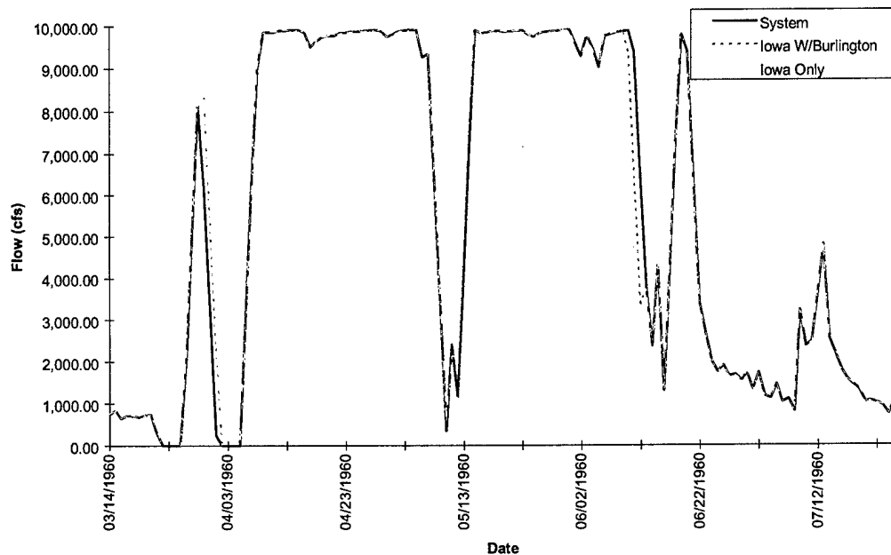
FIGURE E-3b. Model Results of Coralville Reservoir Release - Flood of 1960
