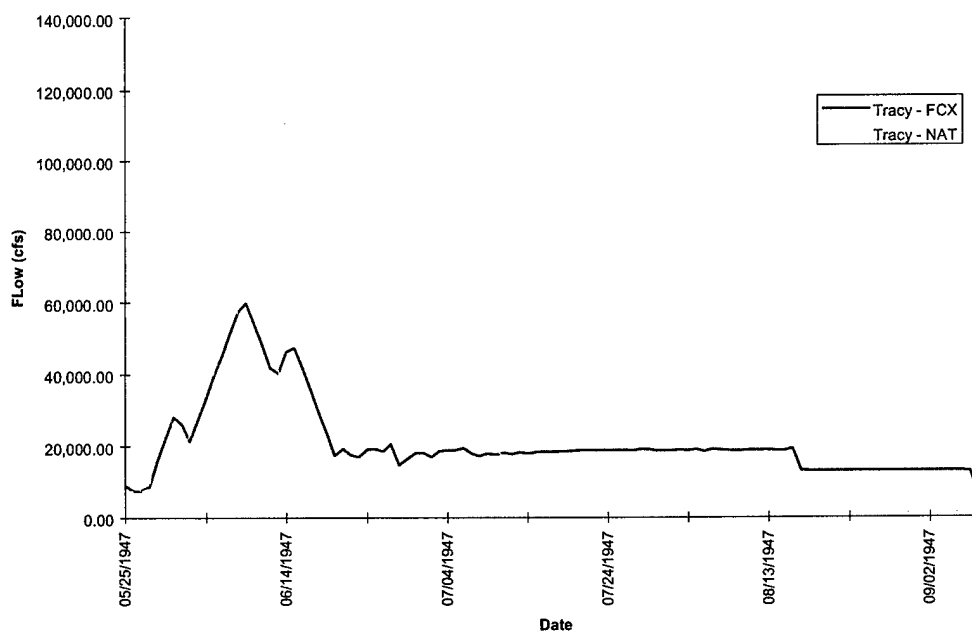
FIGURE D-2h. Tracy Hydrograph - Flood of 1947
