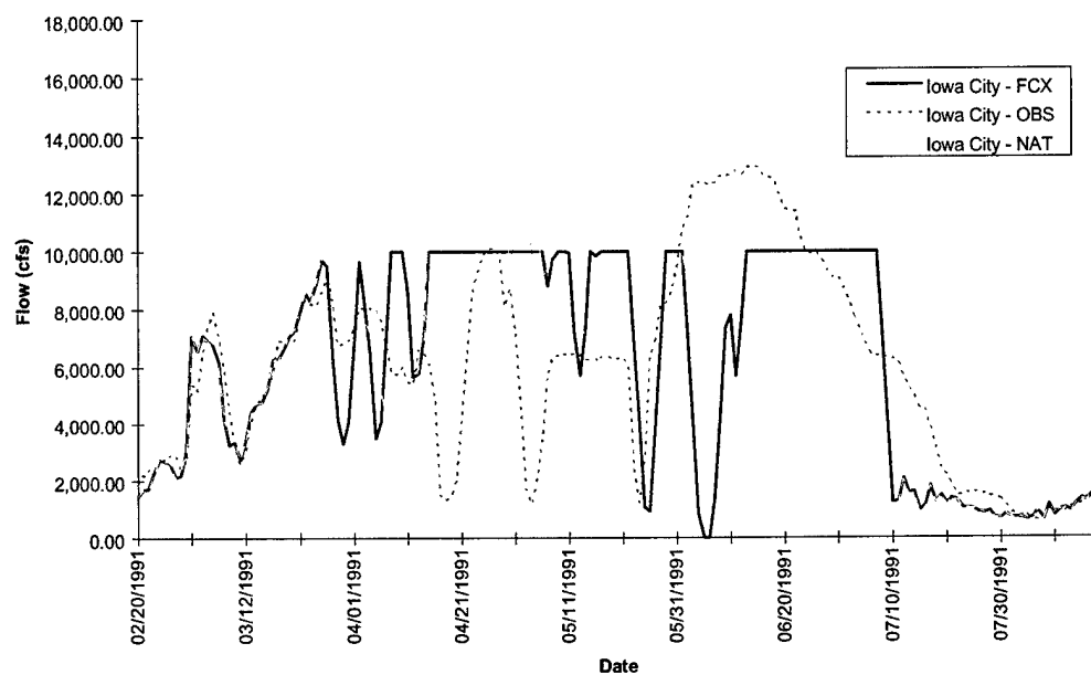
FIGURE D-9b. Iowa City Hydrograph - Flood of 1991
