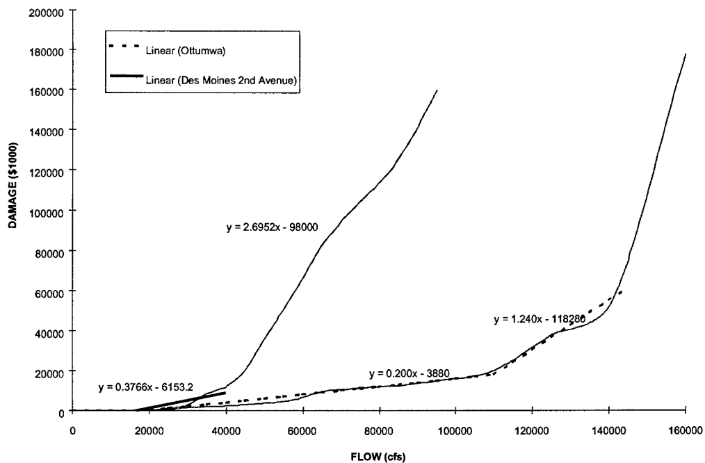
FIGURE 4-7 Des Moines River Penalty Functions
