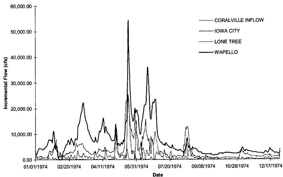
FIGURE C-11 Iowa River Incremental Inflows - Flood of 1974
