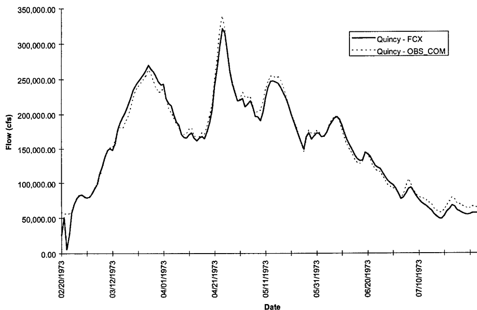
FIGURE D-5l. Quincy Hydrograph - Flood of 1973
