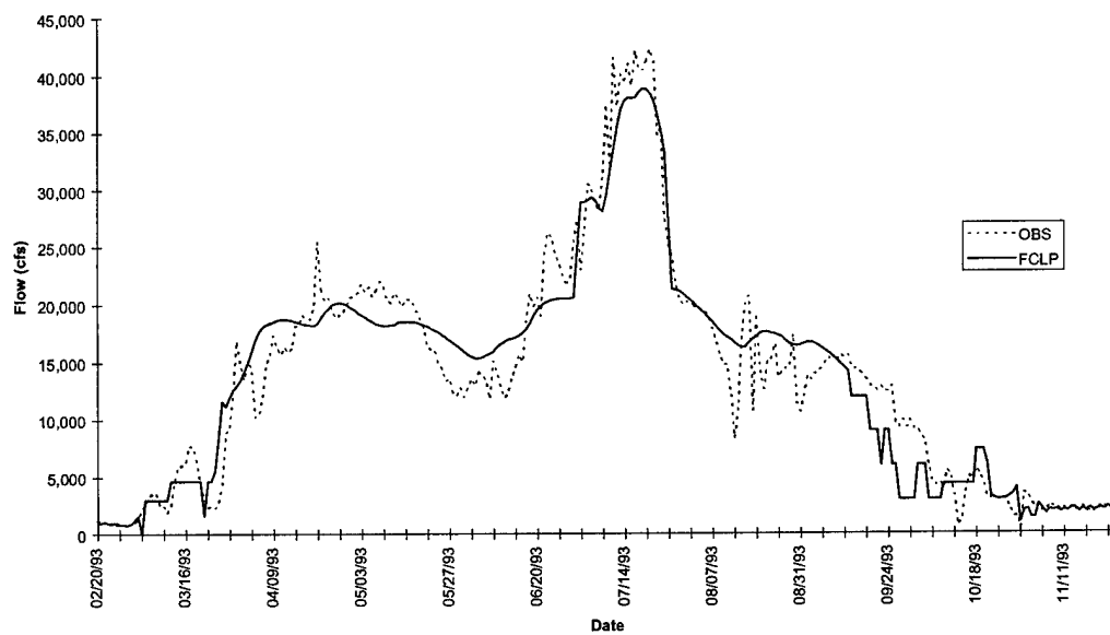
FIGURE 5-7 Des Moines 2 nd Avenue Hydrograph - Flood of 1993
