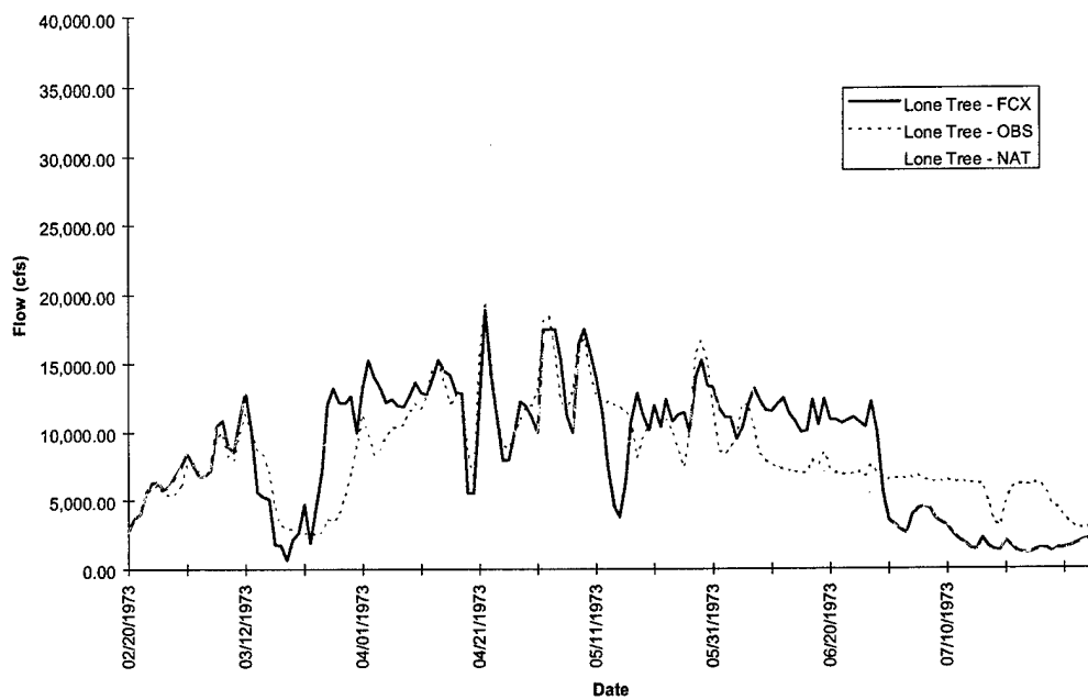
FIGURE D-5c. Lone Tree Hydrograph - Flood of 1973
