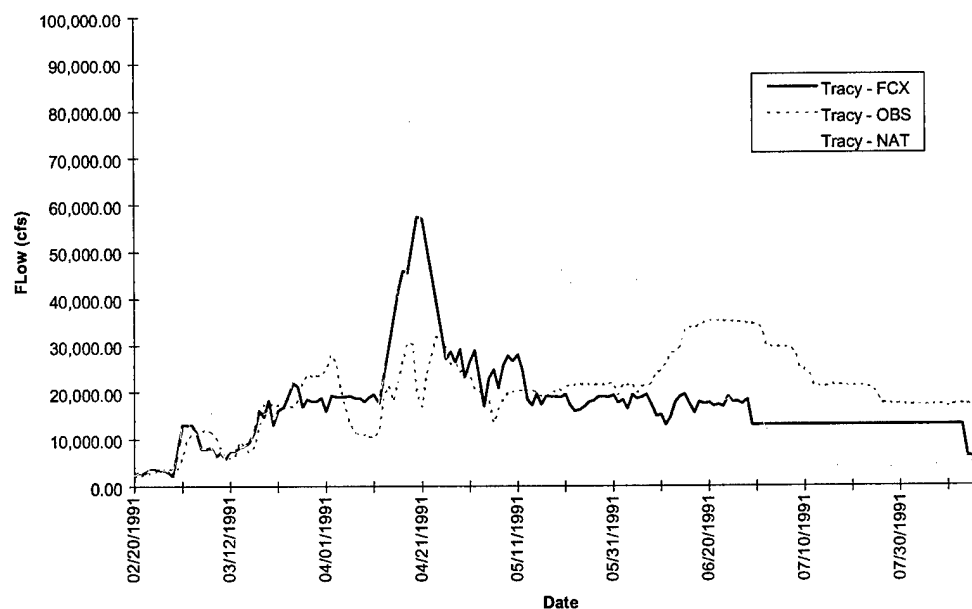
FIGURE D-9h. Tracy Hydrograph - Flood of 1991
