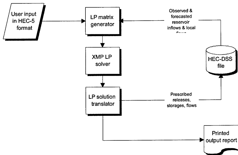
Figure 3. FCLP components
