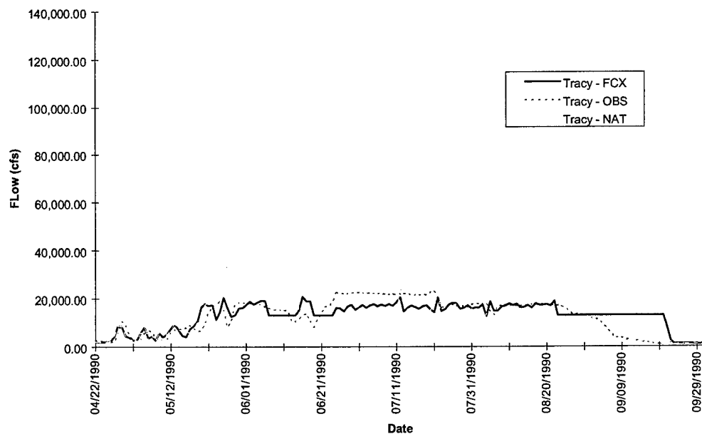
FIGURE D-8h. Tracy Hydrograph - Flood of 1990
