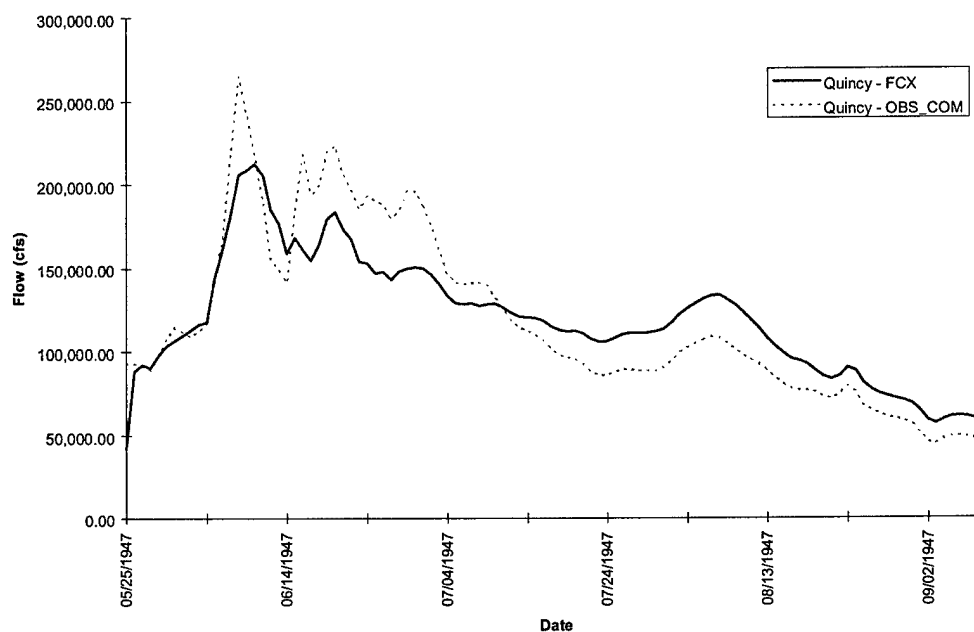
FIGURE D-2l. Quincy Hydrograph - Flood of 1947
