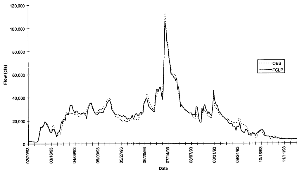
FIGURE 5-8 Des Moines 14 th Street Hydrograph - Flood of 1993
