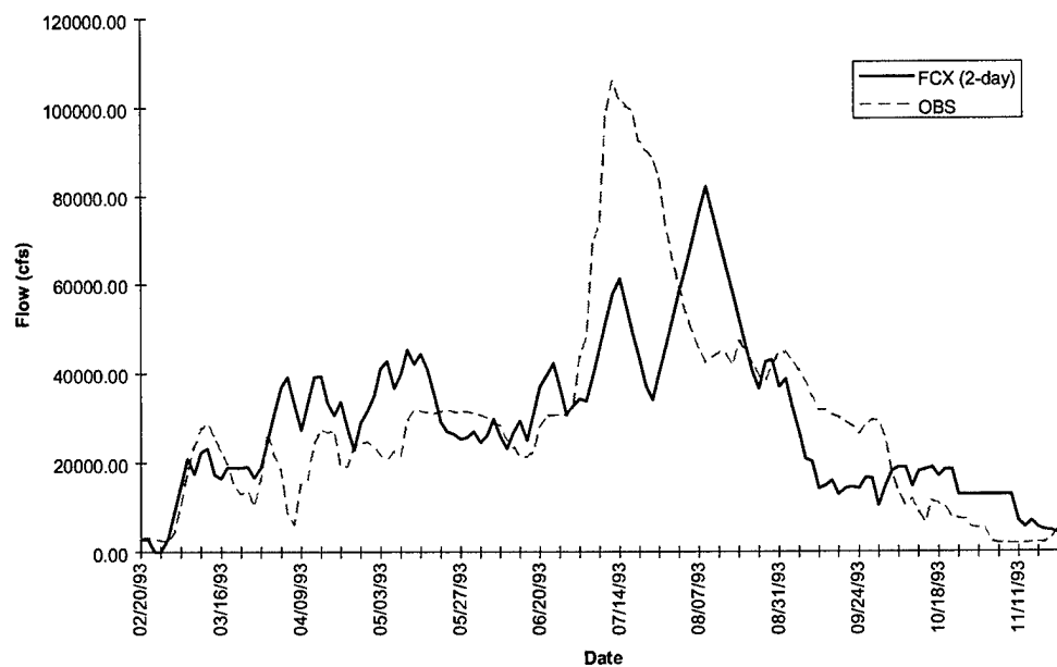
FIGURE D-10h. Tracy Hydrograph - Flood of 1993
