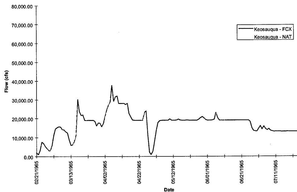
FIGURE D-4j. Keosauqua Hydrograph - Flood of 1965
