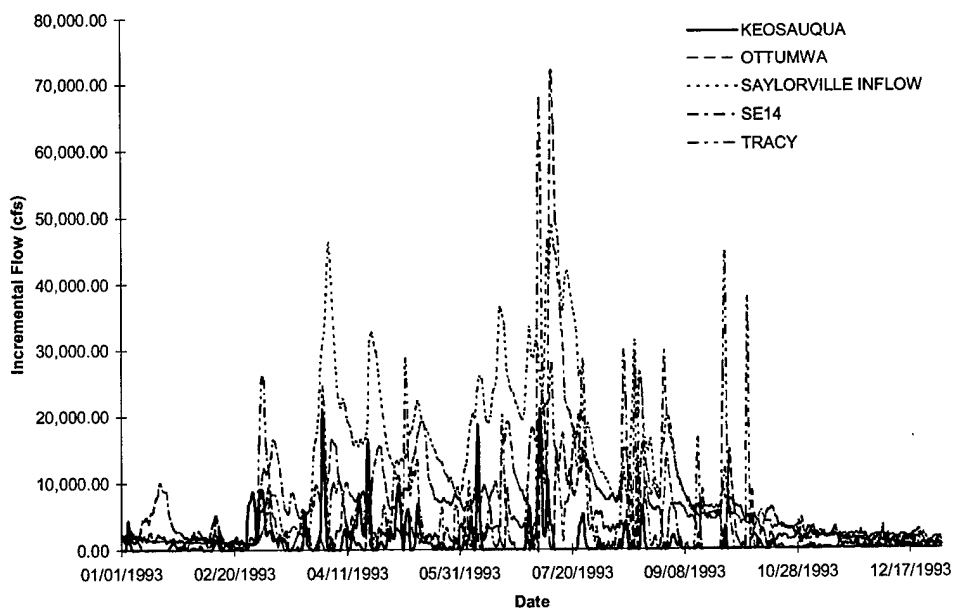
FIGURE C-20 Des Moines River Incremental Inflows - Flood of 1993
