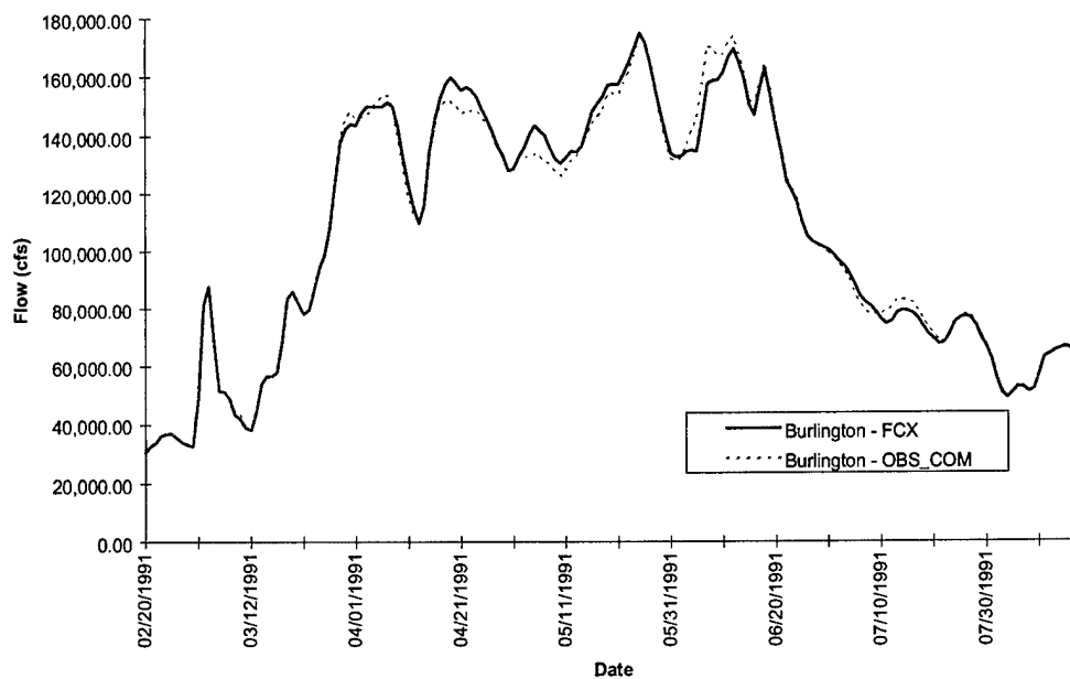
FIGURE D-9k. Burlington Hydrograph - Flood of 1991
