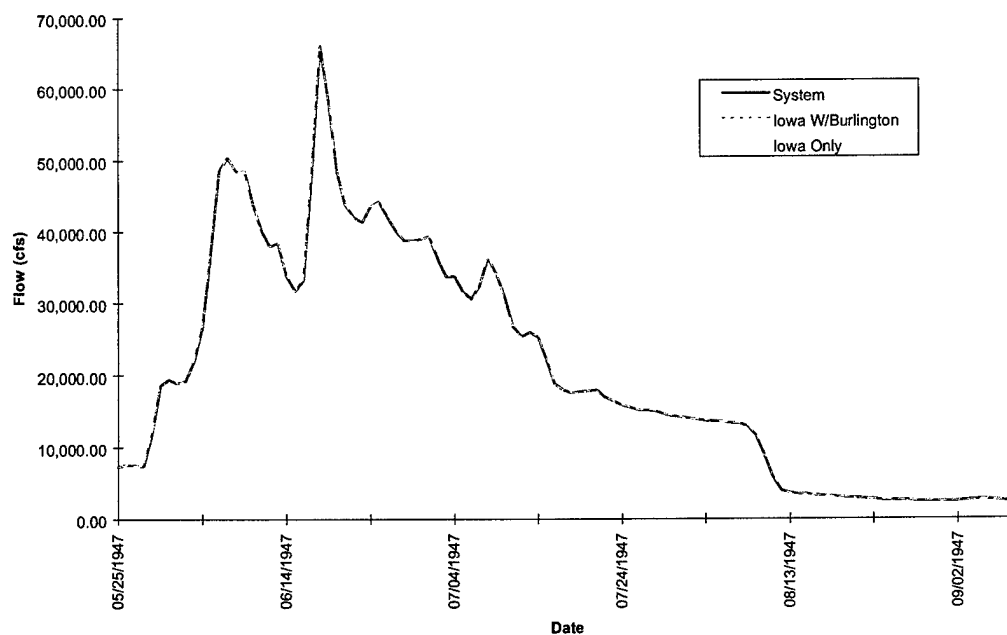
FIGURE E-2e. Hydrograph of Model Results at Wapello - Flood of 1947
