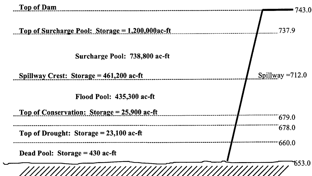
FIGURE 4-1 Coralville Reservoir Storage Levels. Values from 1990 Regulation Manual (1983 Survey)
