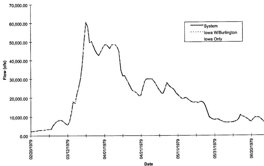
FIGURE E-7e. Hydrograph of Model Results at Wapello - Flood of 1979
