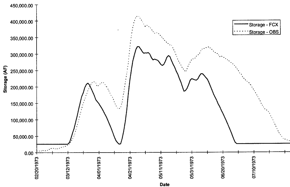
FIGURE D-5a. Coralville Reservoir Storage - Flood of 1973
