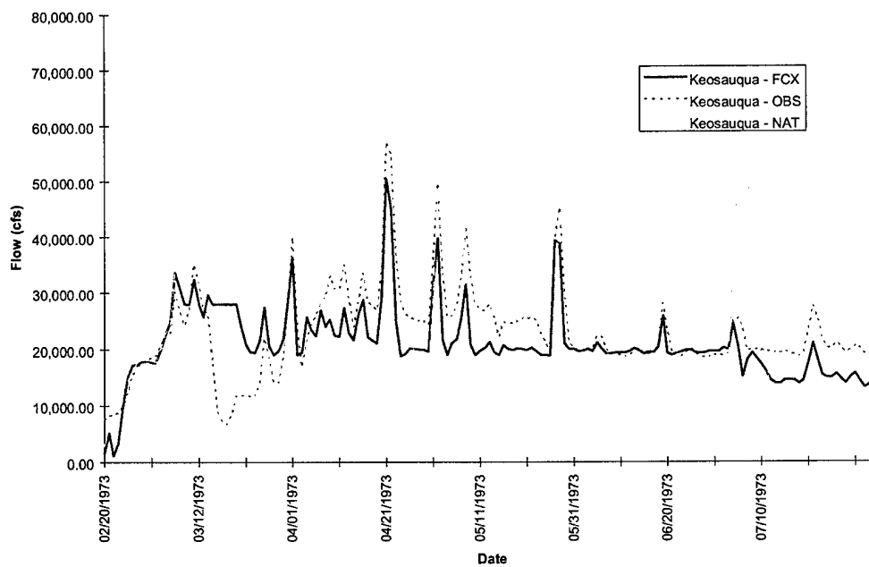
FIGURE D-5j. Keosauqua Hydrograph - Flood of 1973
