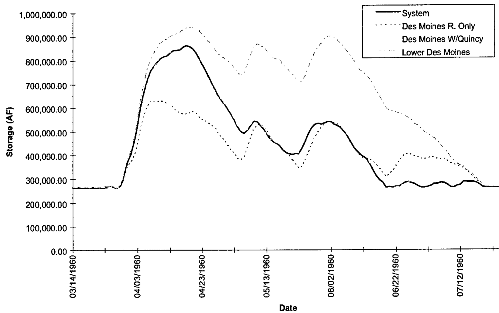
FIGURE E-3i. Model Results of Lake Red Rock Storage - Flood of 1960
