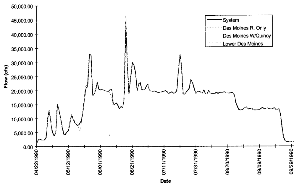
FIGURE E-8m. Hydrograph of Model Results at Keosauqua - Flood of 1990
