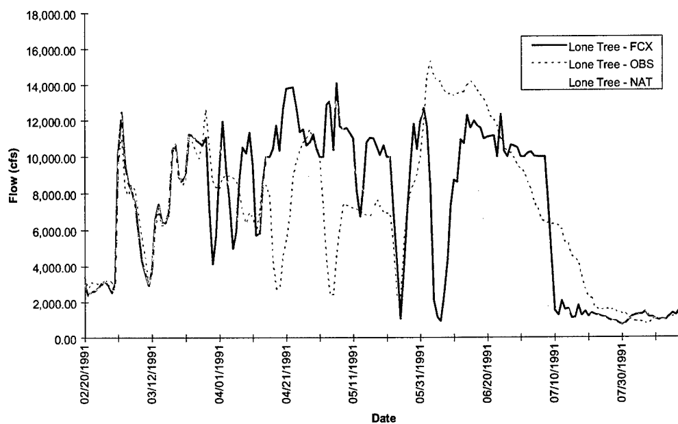
FIGURE D-9c. Lone Tree Hydrograph - Flood of 1991
