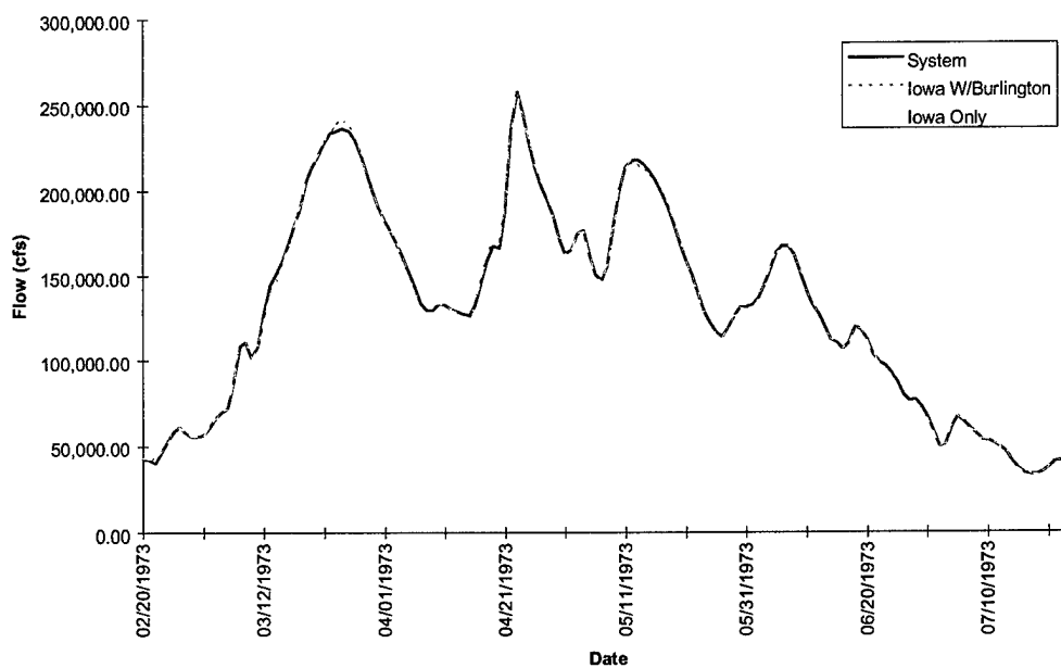
FIGURE E-5n. Hydrograph of Model Results at Burlington - Flood of 1973
