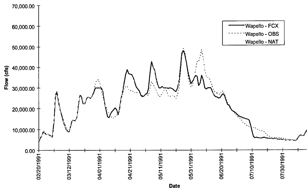
FIGURE D-9d. Wapello Hydrograph - Flood of 1991
