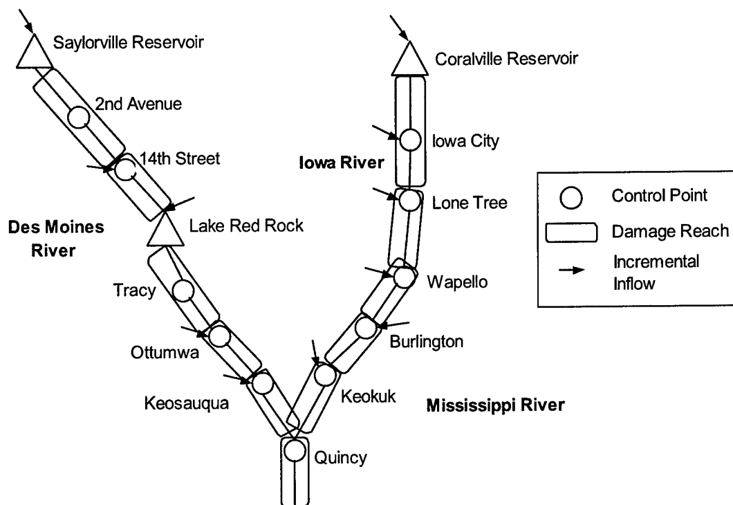
FIGURE 4-5 Damage Reaches for Flow-Damage Functions
