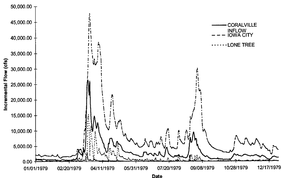
FIGURE C-13 Iowa River Incremental Inflows - Flood of 1979
