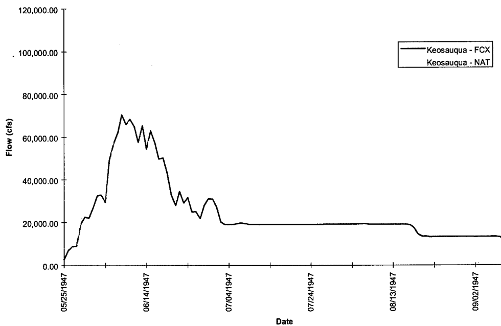
FIGURE D-2j. Keosauqua Hydrograph - Flood of 1947
