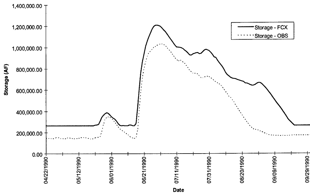
FIGURE D-8g. Lake Red Rock Storage - Flood of 1990
