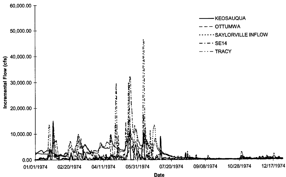
FIGURE C-12 Des Moines River Incremental Inflows - Flood of 1974
