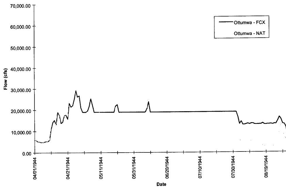
FIGURE D-1i. Ottumwa Hydrograph - Flood of 1944
