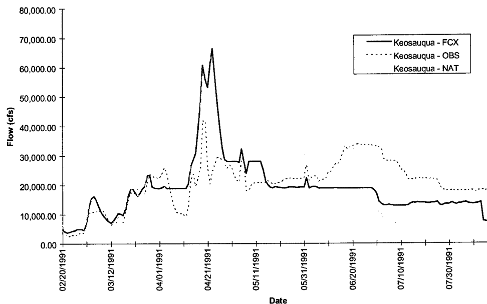
FIGURE D-9j. Keosauqua Hydrograph - Flood of 1991
