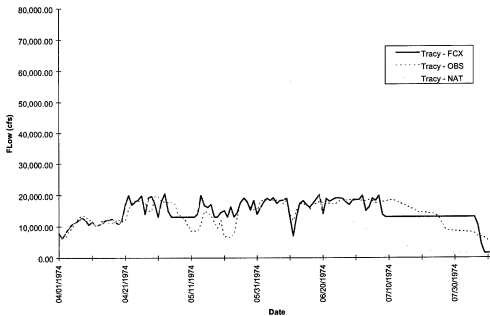
FIGURE D-6h. Tracy Hydrograph - Flood of 1974
