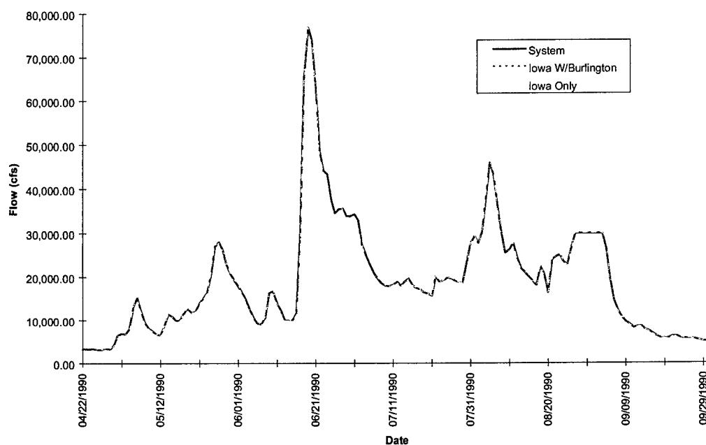
FIGURE E-8e. Hydrograph of Model Results at Wapello - Flood of 1990
