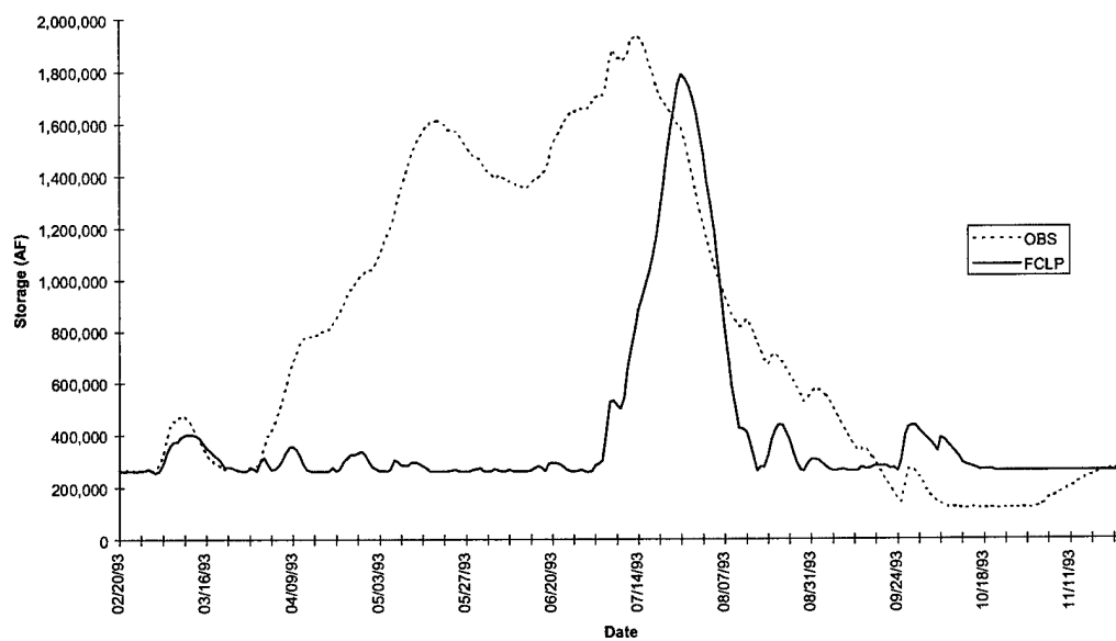
FIGURE 5-9 Lake Red Rock Storage - Flood of 1993
