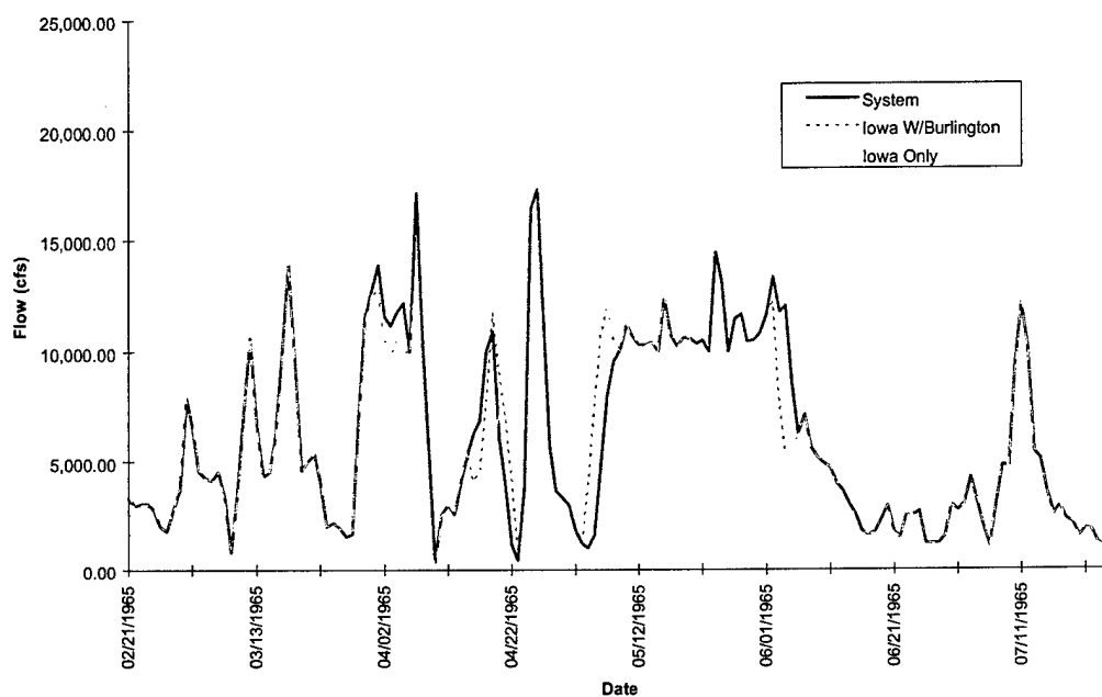
FIGURE E-4d. Hydrograph of Model Results at Lone Tree - Flood of 1965
