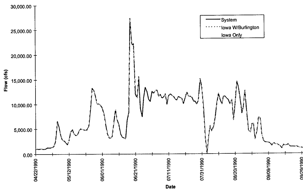
FIGURE E-8d. Hydrograph of Model Results at Lone Tree - Flood of 1990
