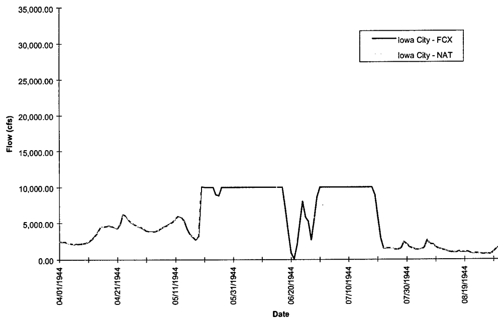
FIGURE D-1b. Iowa City Hydrograph - Flood of 1944
