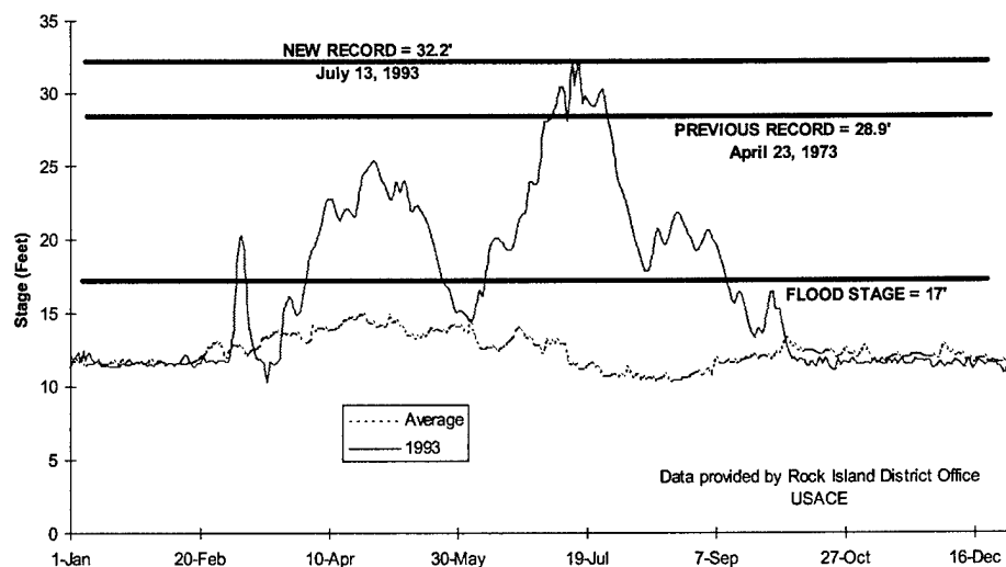
FIGURE 2-3 1993 Hydrograph for Mississippi River at Quincy, Illinois
