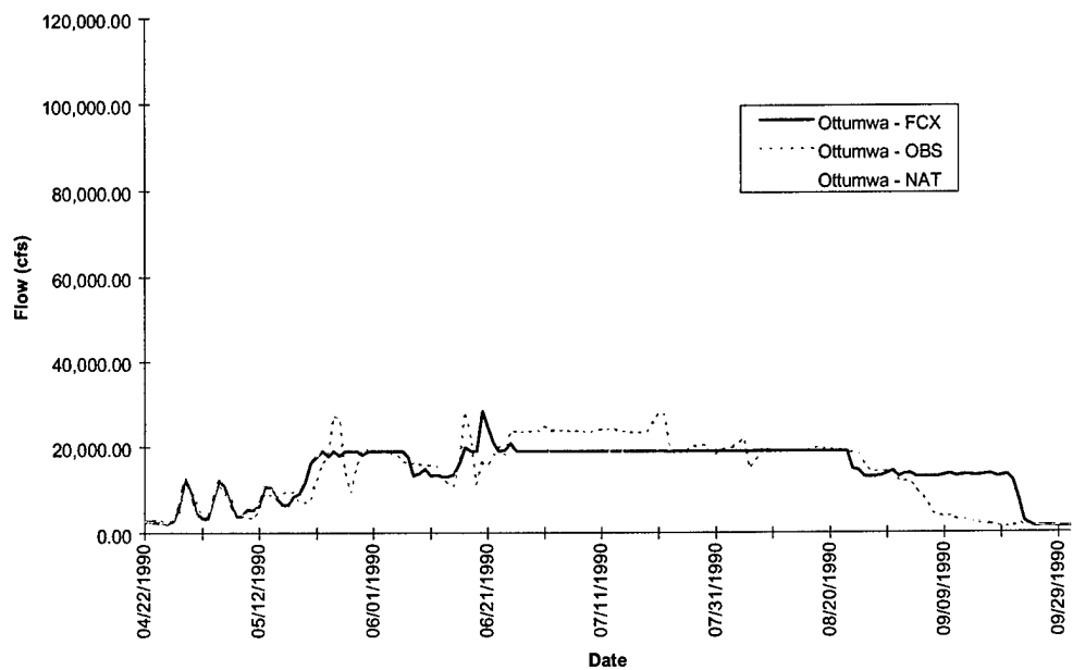
FIGURE D-8i. Ottumwa Hydrograph - Flood of 1990
