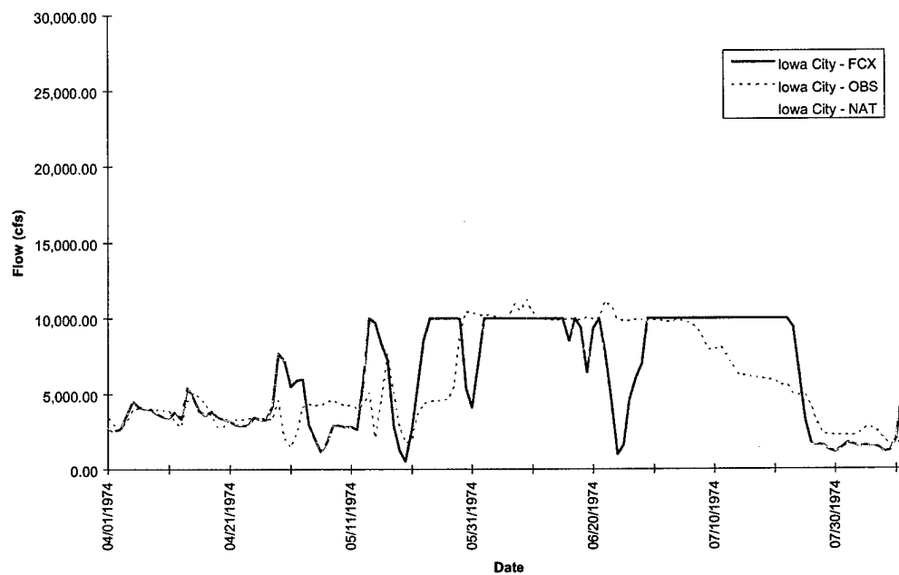
FIGURE D-6b. Iowa City Hydrograph - Flood of 1974
