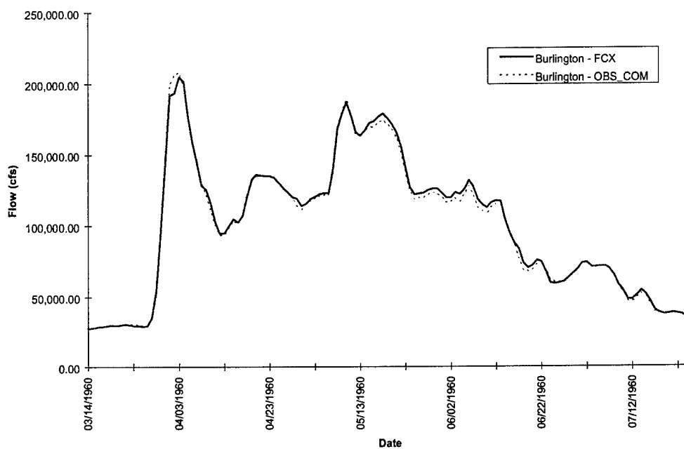
FIGURE D-3k. Burlington Hydrograph - Flood of 1960
