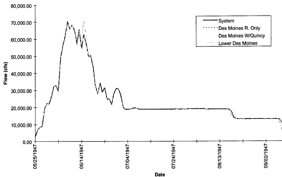
FIGURE E-2m. Hydrograph of Model Results at Keosauqua - Flood of 1947
