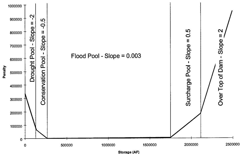
FIGURE 4-4 Storage Penalty Function for Lake Red Rock
