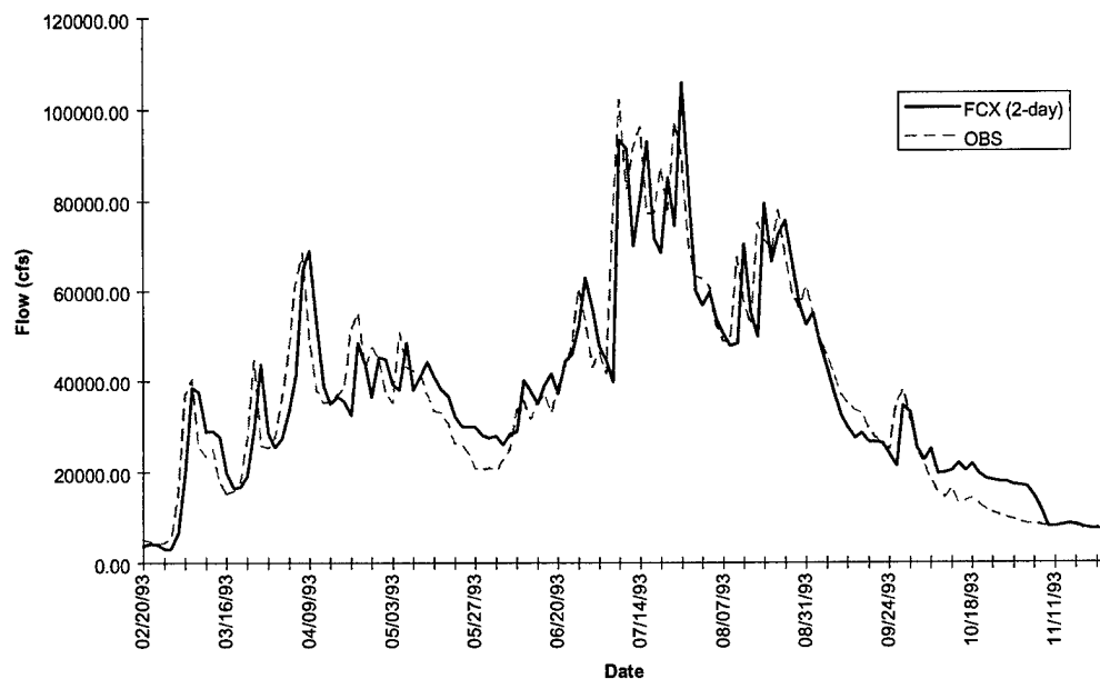
FIGURE D-10d. Wapello Hydrograph - Flood of 1993
