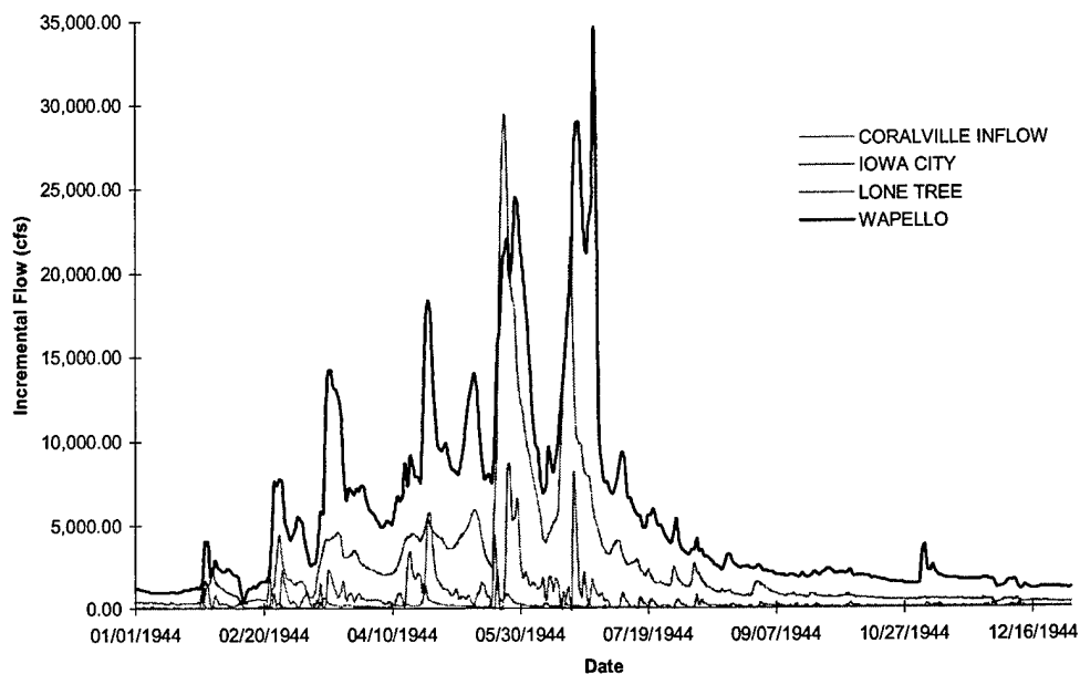
FIGURE C-1 Iowa River Incremental Inflows - Flood of 1944
