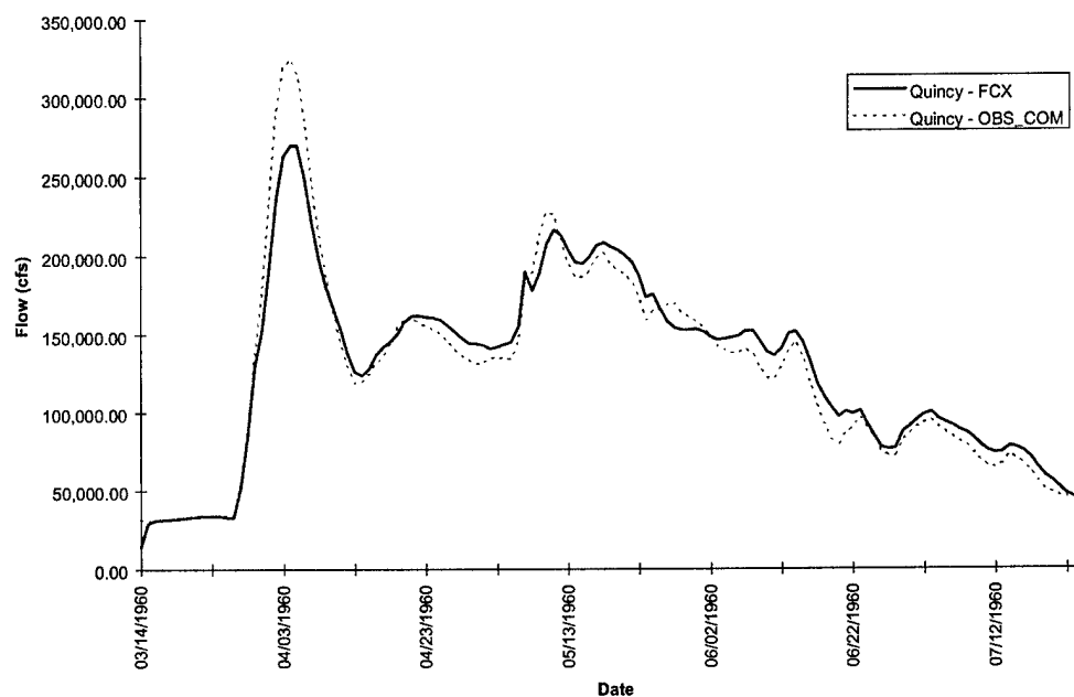
FIGURE D-3l. Quincy Hydrograph - Flood of 1960
