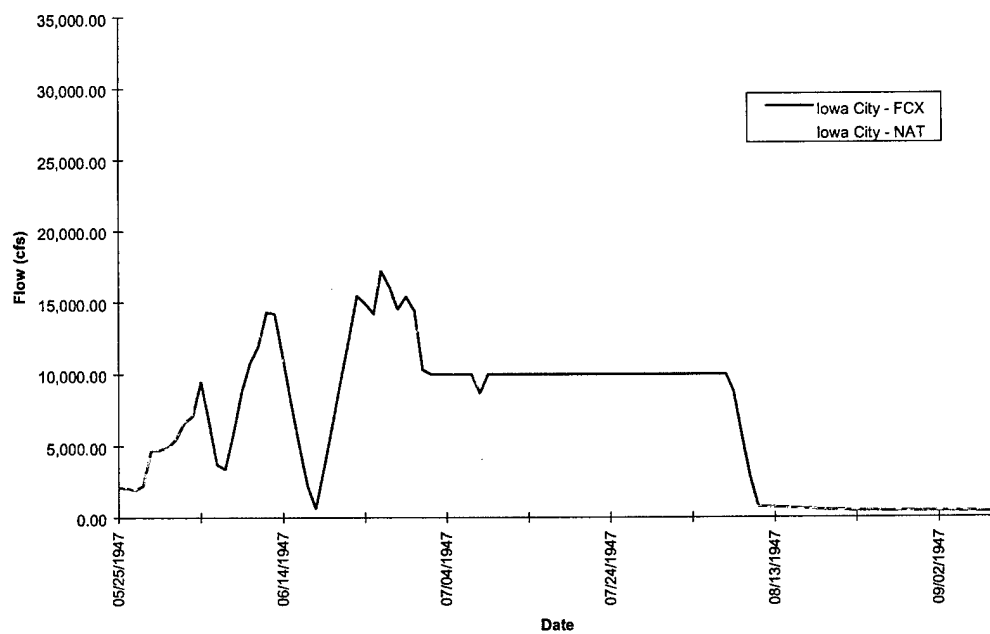
FIGURE D-2b. Iowa City Hydrograph - Flood of 1947
