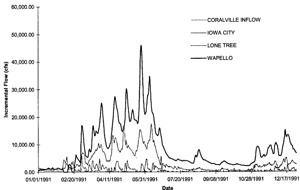
FIGURE C-17 Iowa River Incremental Inflows - Flood of 1991
