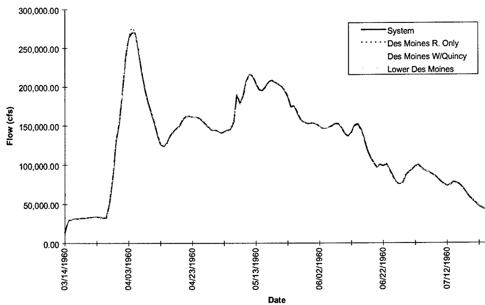
FIGURE E-30. Hydrograph of Model Results at Quincy - Flood of 1960
