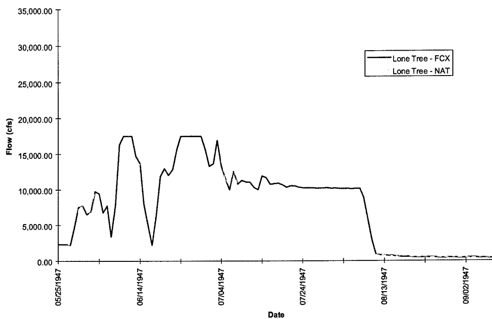
FIGURE D-2c. Lone Tree Hydrograph - Flood of 1947
