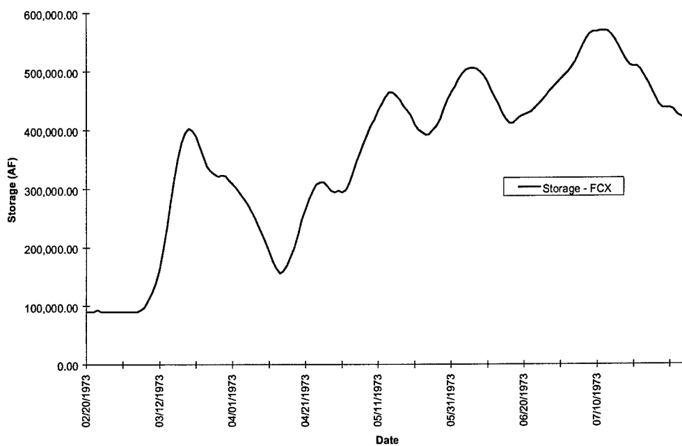
FIGURE D-5e. Saylorville Reservoir Storage - Flood of 1973
