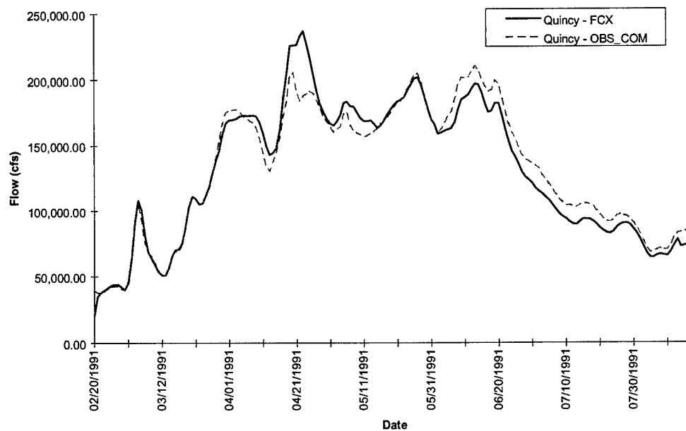
FIGURE D-9l. Quincy Hydrograph - Flood of 1991
