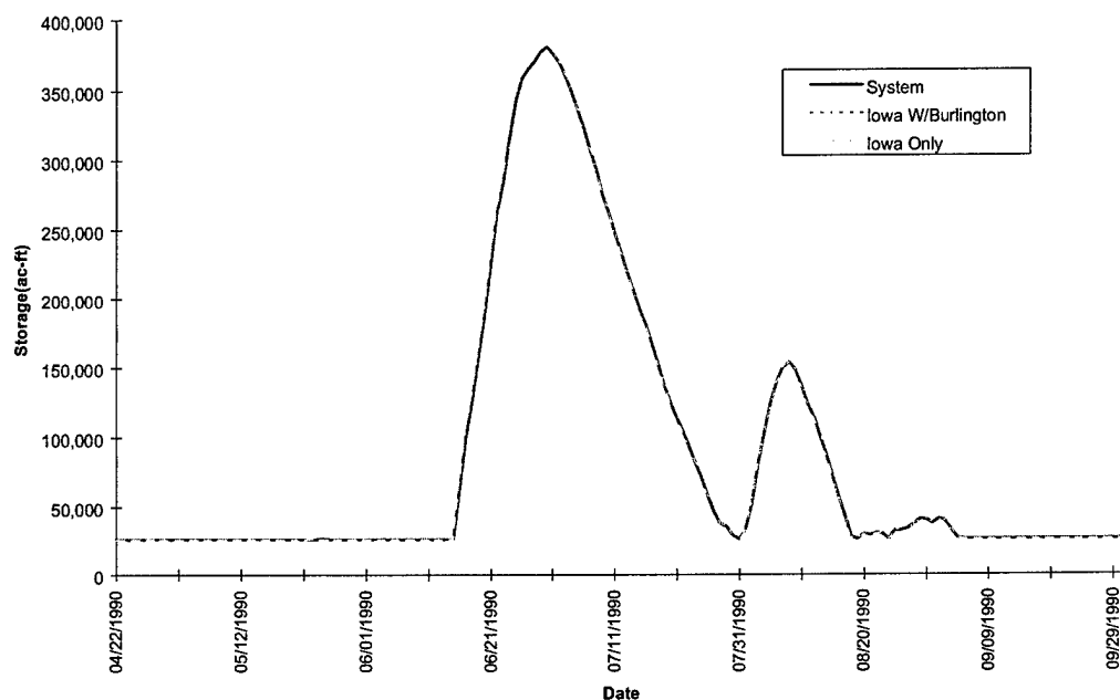
FIGURE E-8a. Model Results of Coralville Reservoir Storage - Flood of 1990
