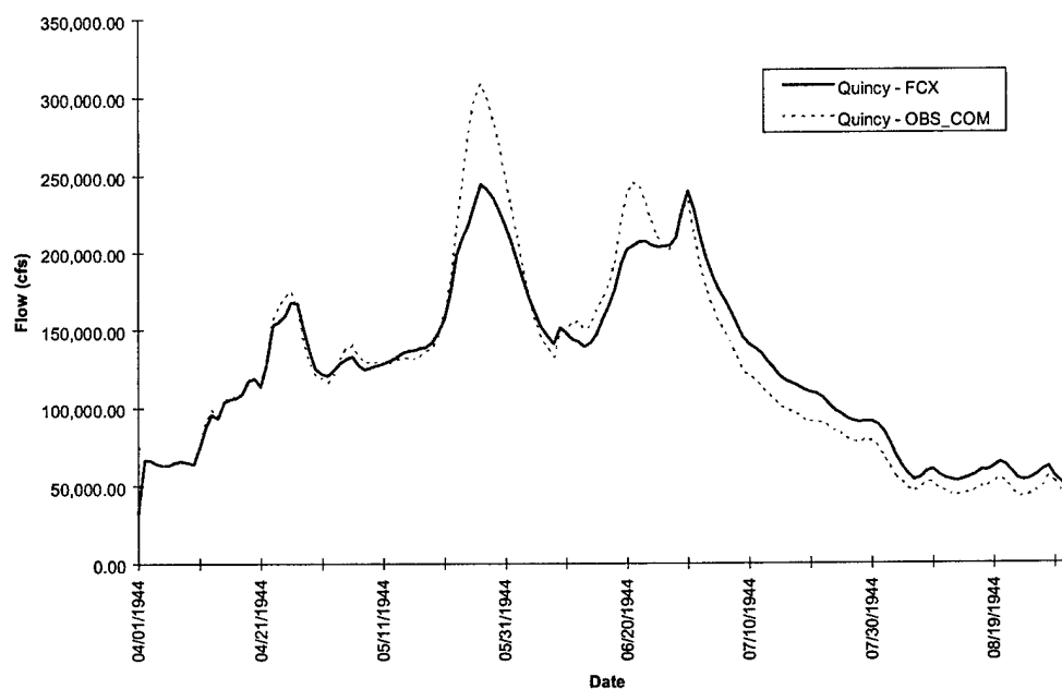
FIGURE D-1l. Quincy Hydrograph - Flood of 1944
