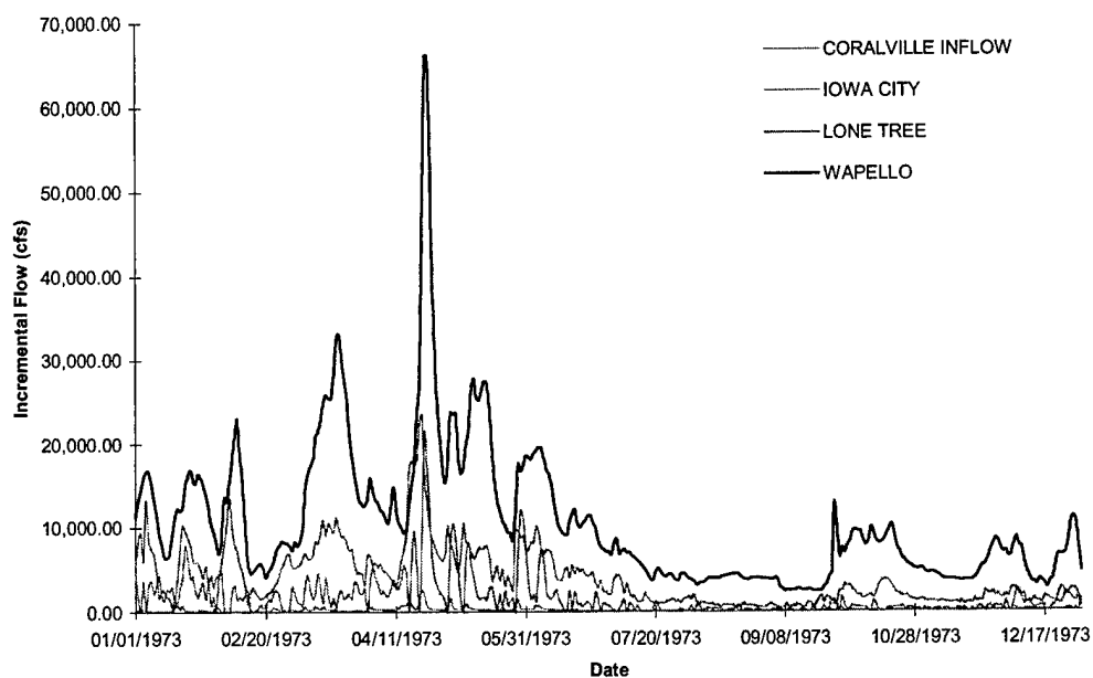
FIGURE C-9 Iowa River Incremental Inflows - Flood of 1973
