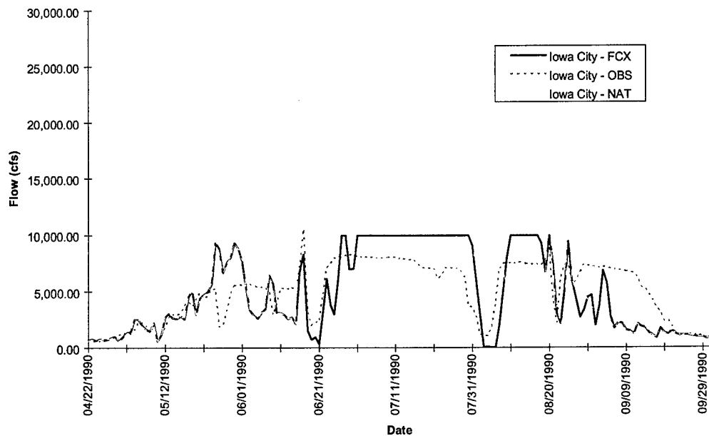
FIGURE D-8b. Iowa City Hydrograph - Flood of 1990
