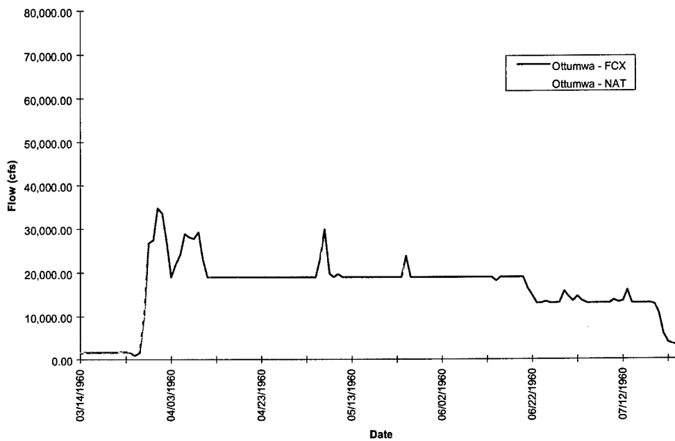
FIGURE D-3i. Ottumwa Hydrograph - Flood of 1960
