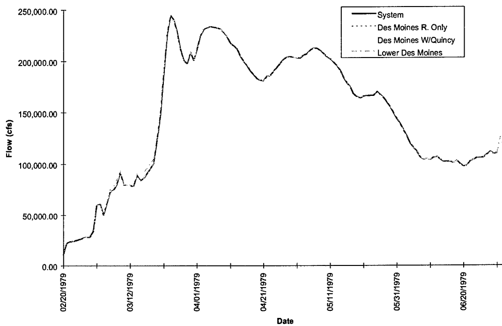
FIGURE E-70. Hydrograph of Model Results at Quincy - Flood of 1979
