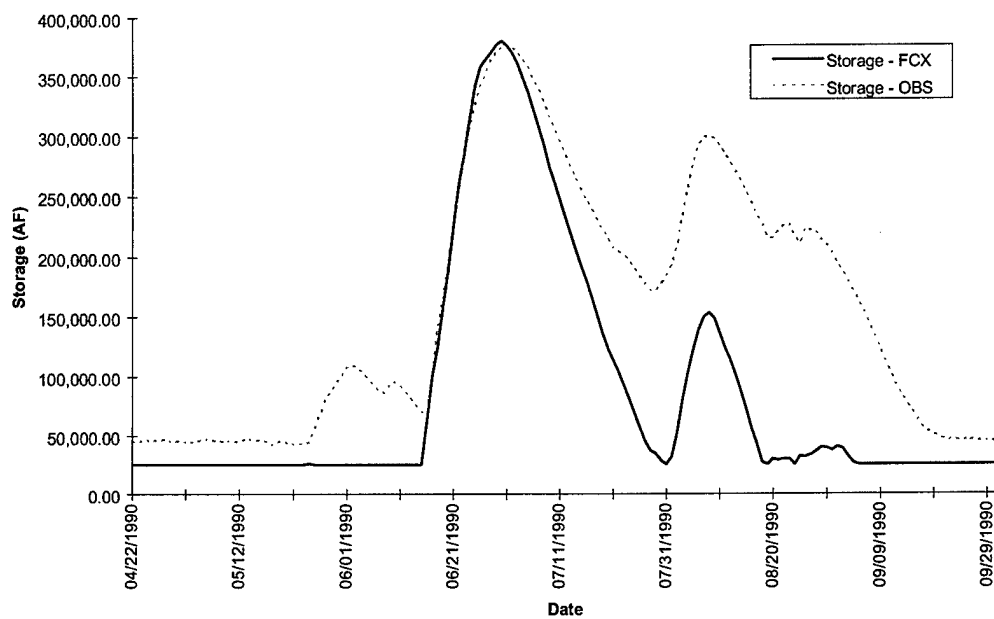
FIGURE D-8a. Coralville Reservoir Storage - Flood of 1990
