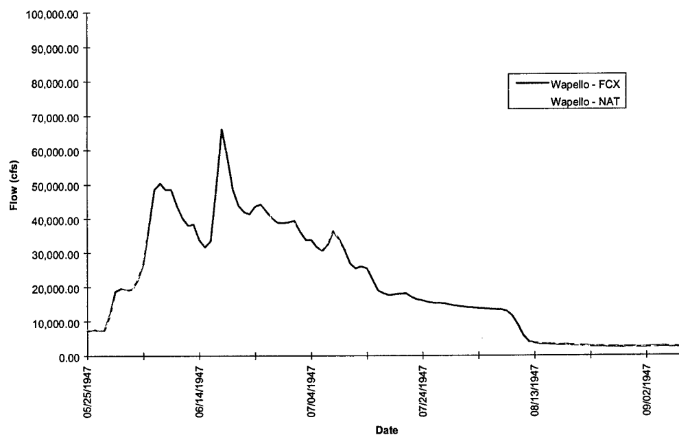
FIGURE D-2d. Wapello Hydrograph - Flood of 1947
