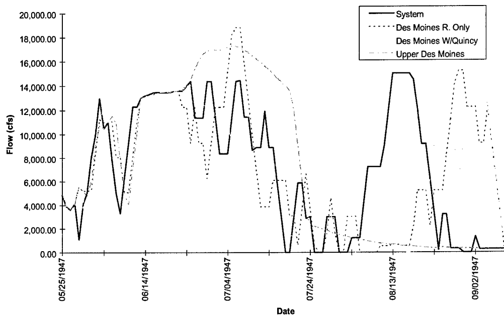
FIGURE E-2g. Model Results of Saylorville Reservoir Release - Flood of 1947
