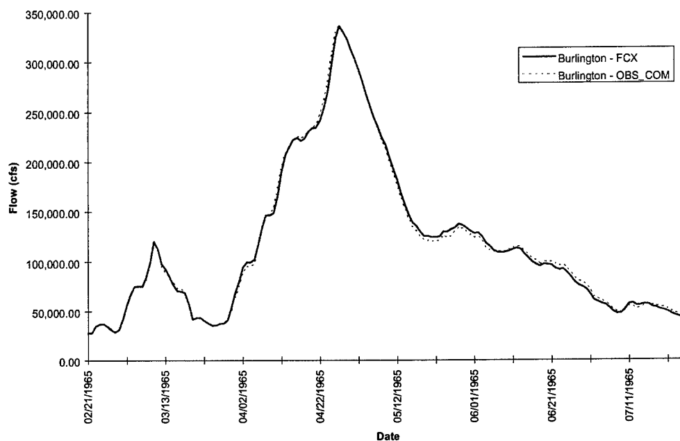
FIGURE D-4k. Burlington Hydrograph - Flood of 1965
