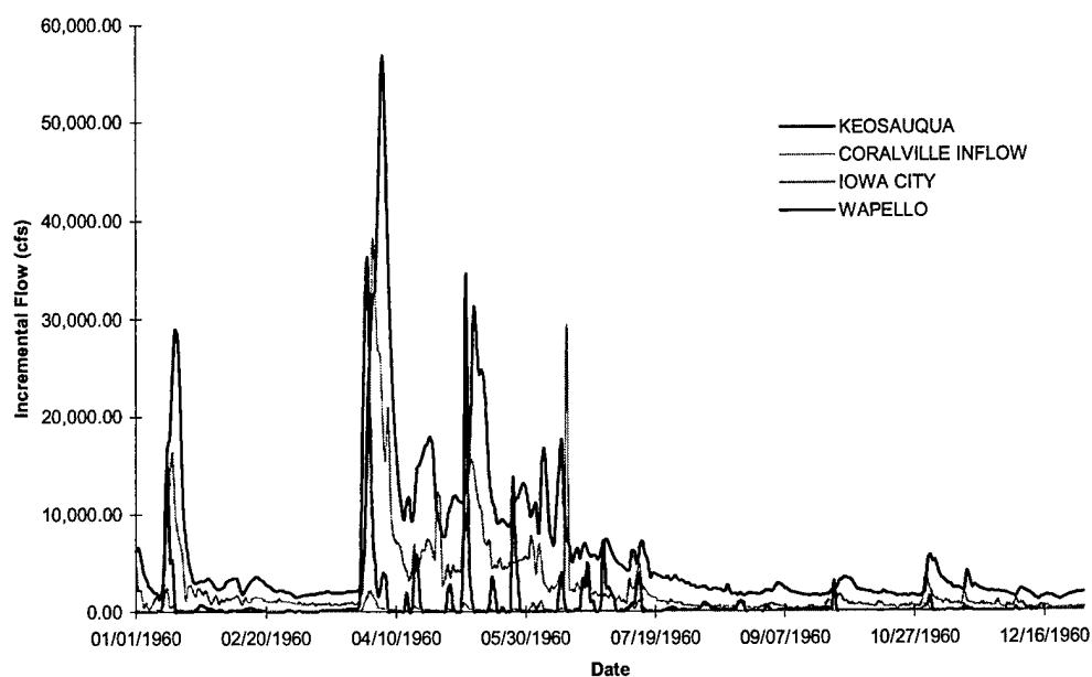
FIGURE C-5 Iowa River Incremental Inflows - Flood of 1960
