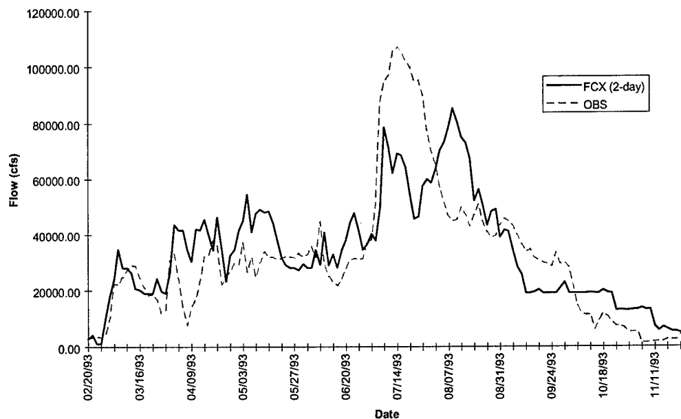
FIGURE D-10j. Keosauqua Hydrograph - Flood of 1993
