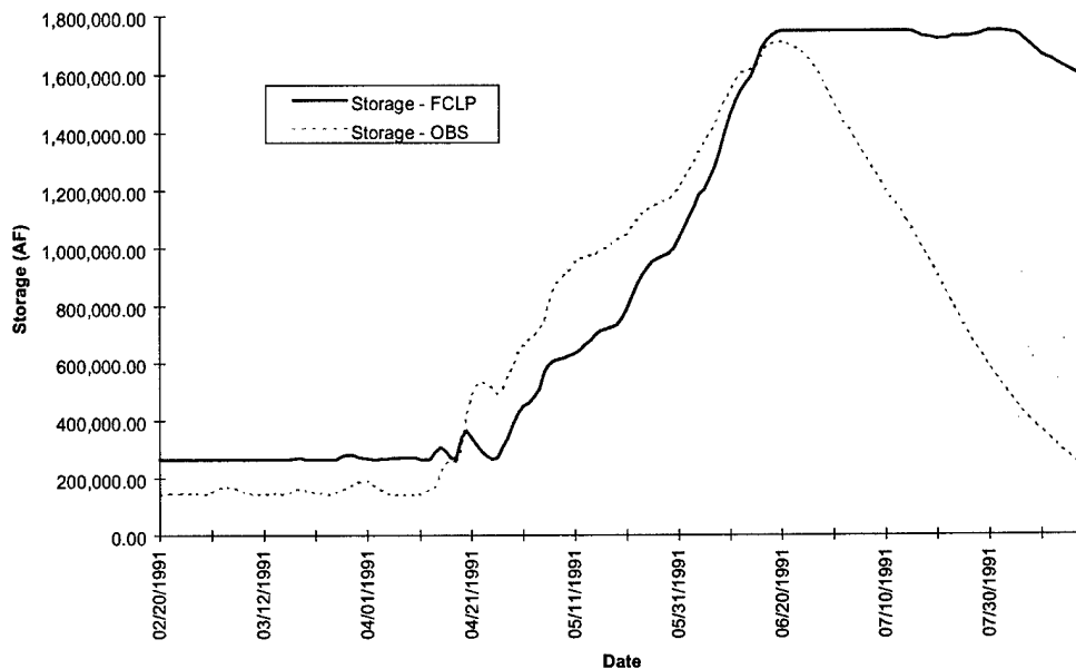
FIGURE 4-10 Lake Red Rock Storage - Flood of 1991
