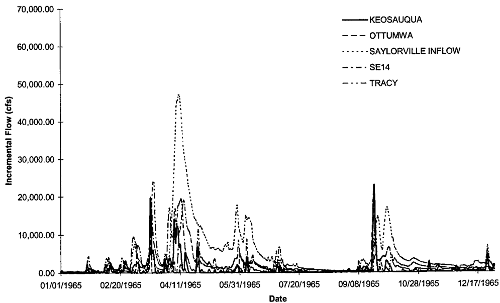
FIGURE C-8 Des Moines River Incremental Inflows - Flood of 1965
