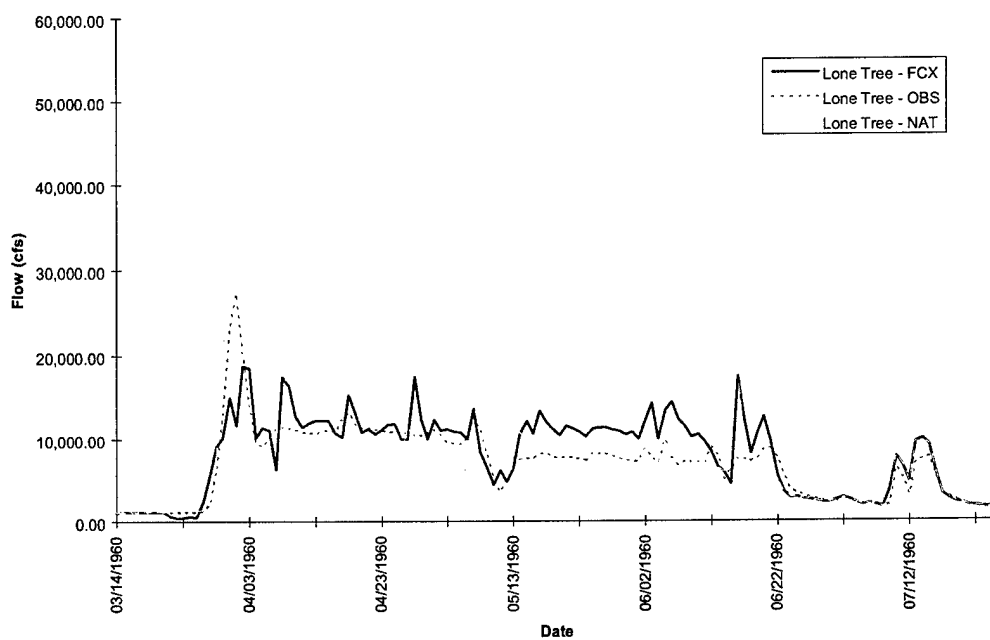
FIGURE D-3c. Lone Tree Hydrograph - Flood of 1960
