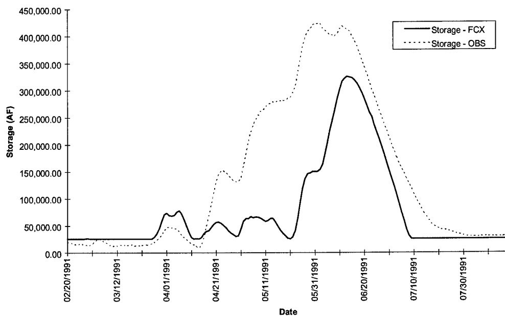
FIGURE D-9a. Coralville Reservoir Storage - Flood of 1991
