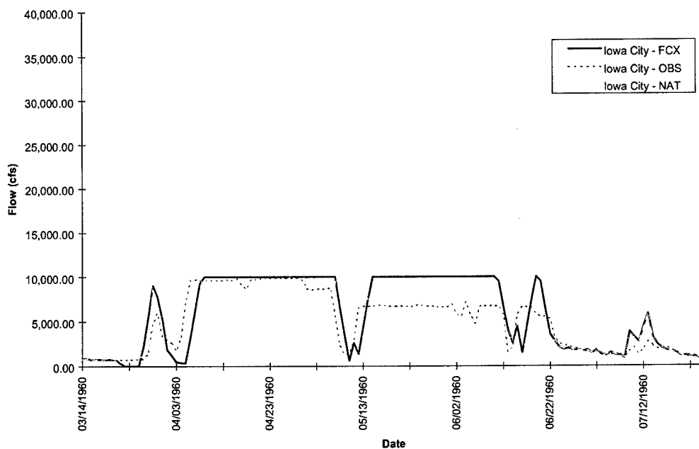
FIGURE D-3b. Iowa City Hydrograph - Flood of 1960
