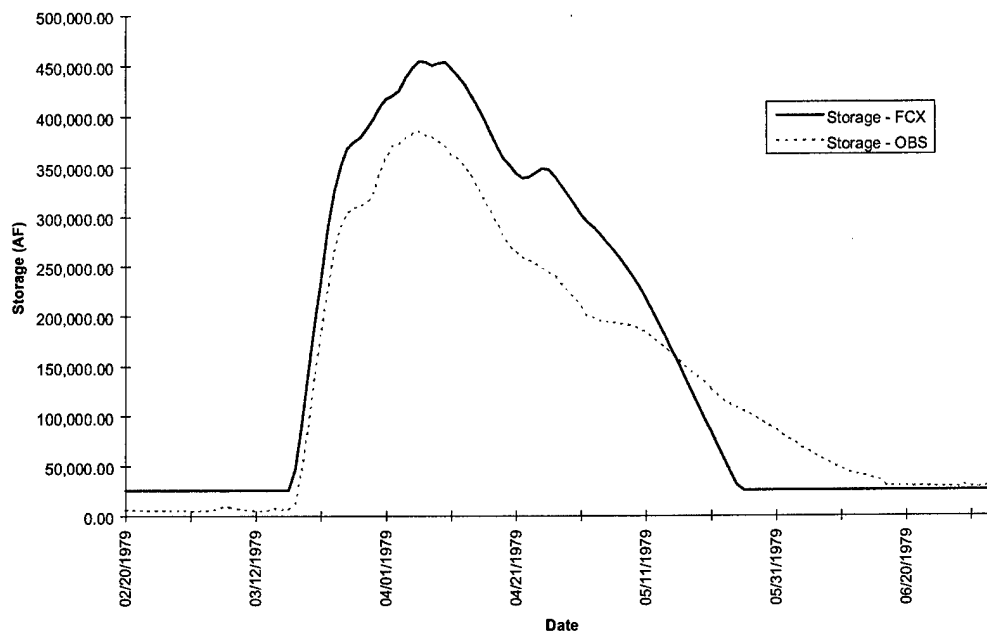
FIGURE D-7a. Coralville Reservoir Storage - Flood of 1979
