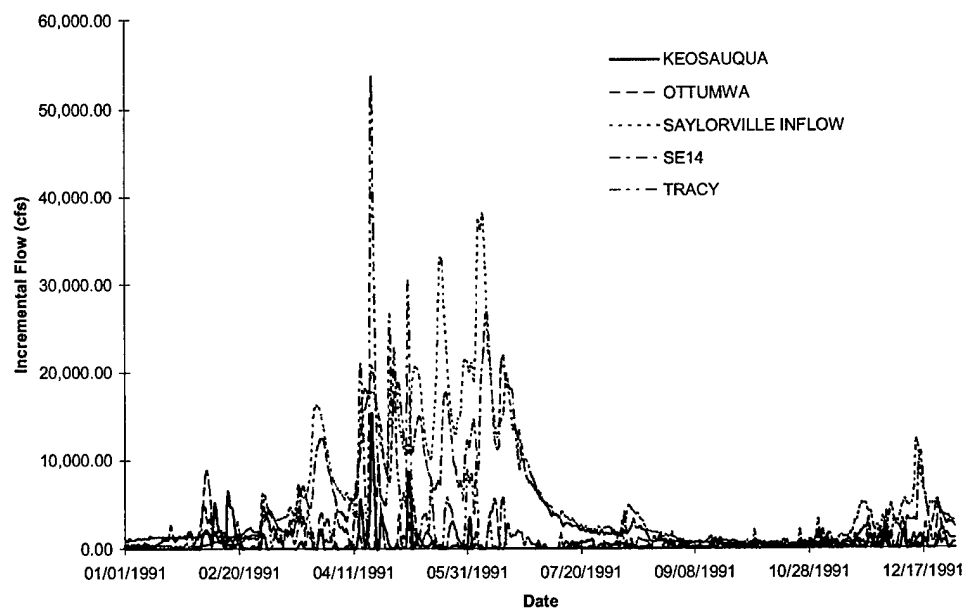
FIGURE C-18 Des Moines River Incremental Inflows - Flood of 1991
