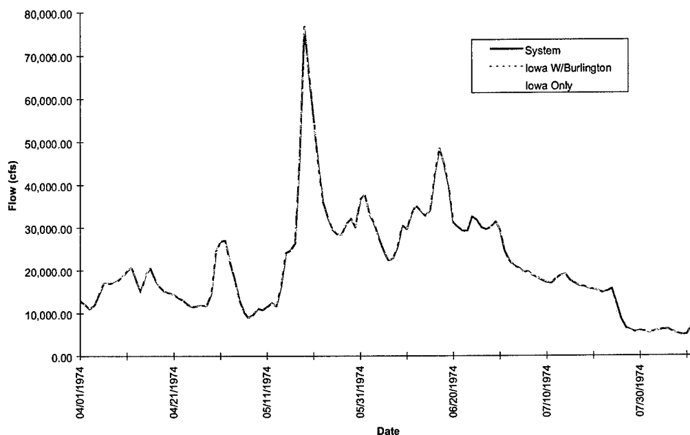
FIGURE E-6e. Hydrograph of Model Results at Wapello - Flood of 1974
