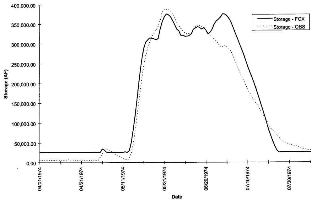
FIGURE D-6a. Coralville Reservoir Storage - Flood of 1974
