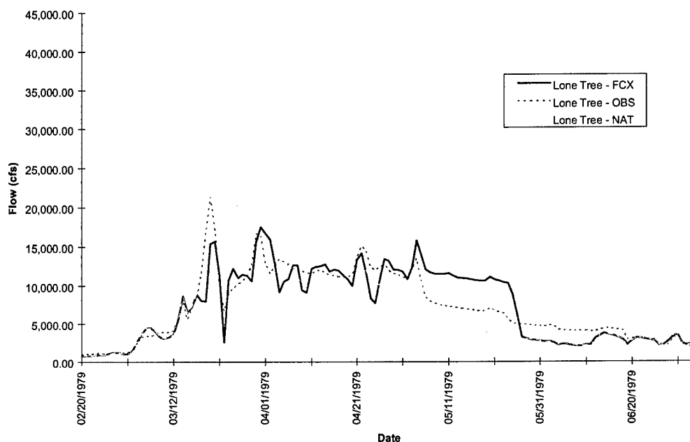
FIGURE D-7c. Lone Tree Hydrograph - Flood of 1979
