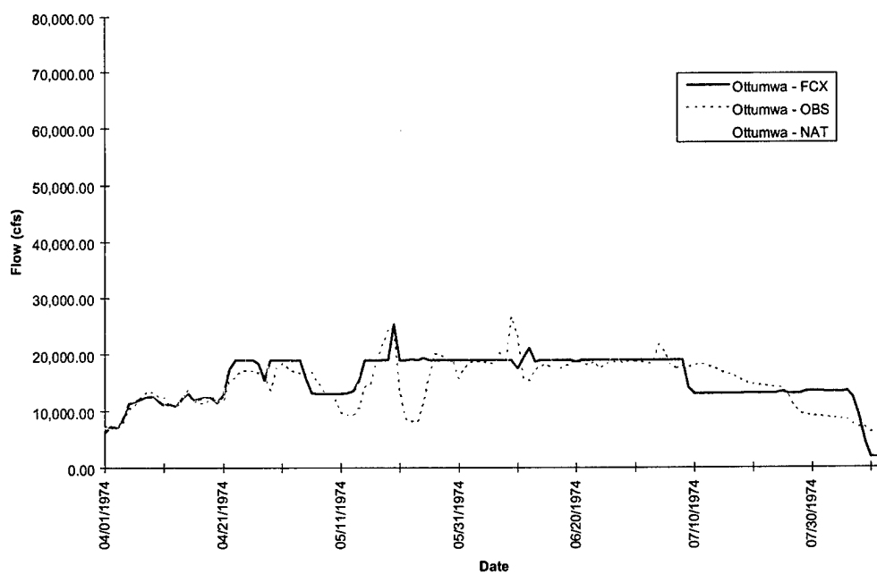
FIGURE D-6i. Ottumwa Hydrograph - Flood of 1974
