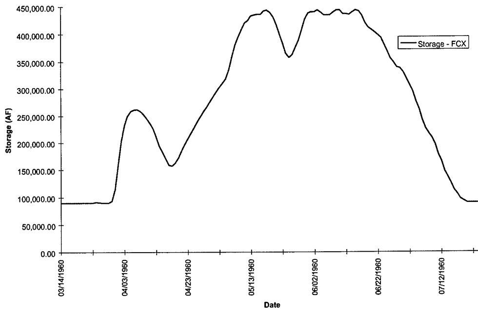
FIGURE D-3e. Saylorville Reservoir Storage - Flood of 1960
