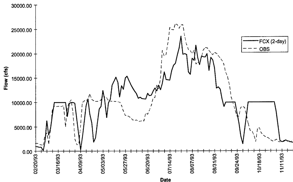
FIGURE D-10b. Iowa City Hydrograph - Flood of 1993
