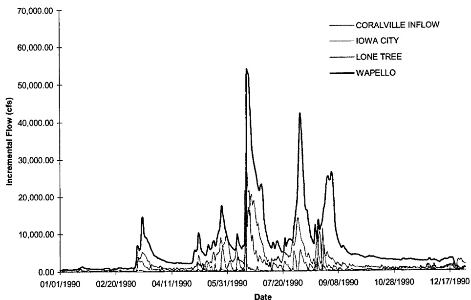
FIGURE C-15 Iowa River Incremental Inflows - Flood of 1990
