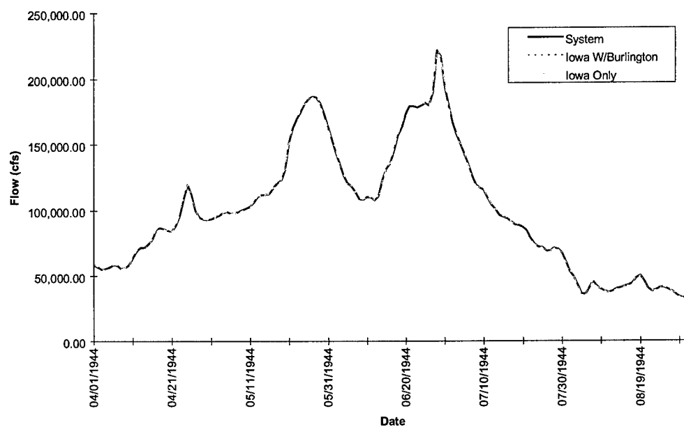
FIGURE E-1n. Hydrograph of Model Results at Burlington - Flood of 1944
