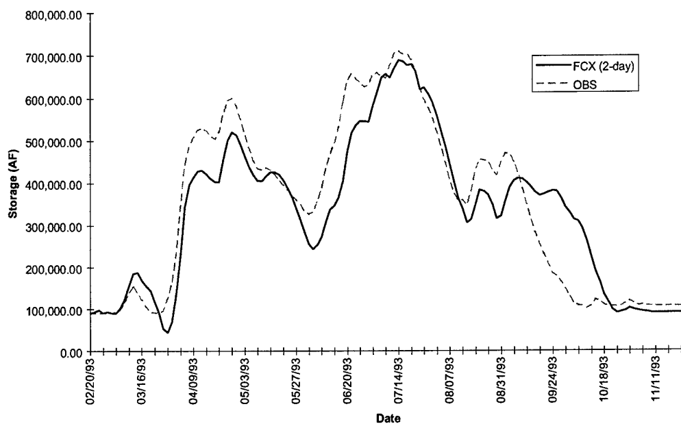
FIGURE D-10e. Saylorville Reservoir Storage - Flood of 1993
