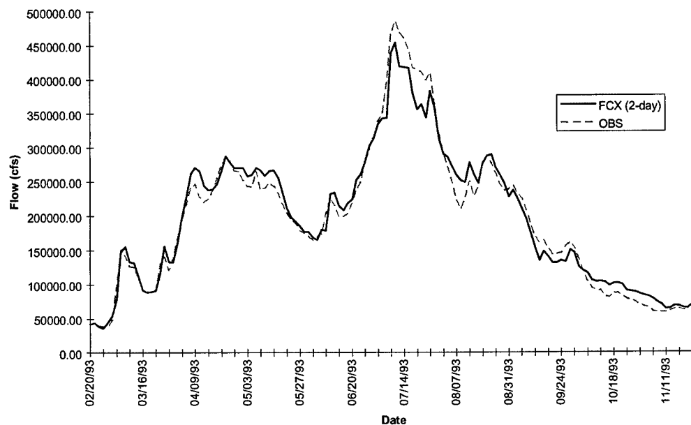
FIGURE D-10l. Quincy Hydrograph - Flood of 1993
