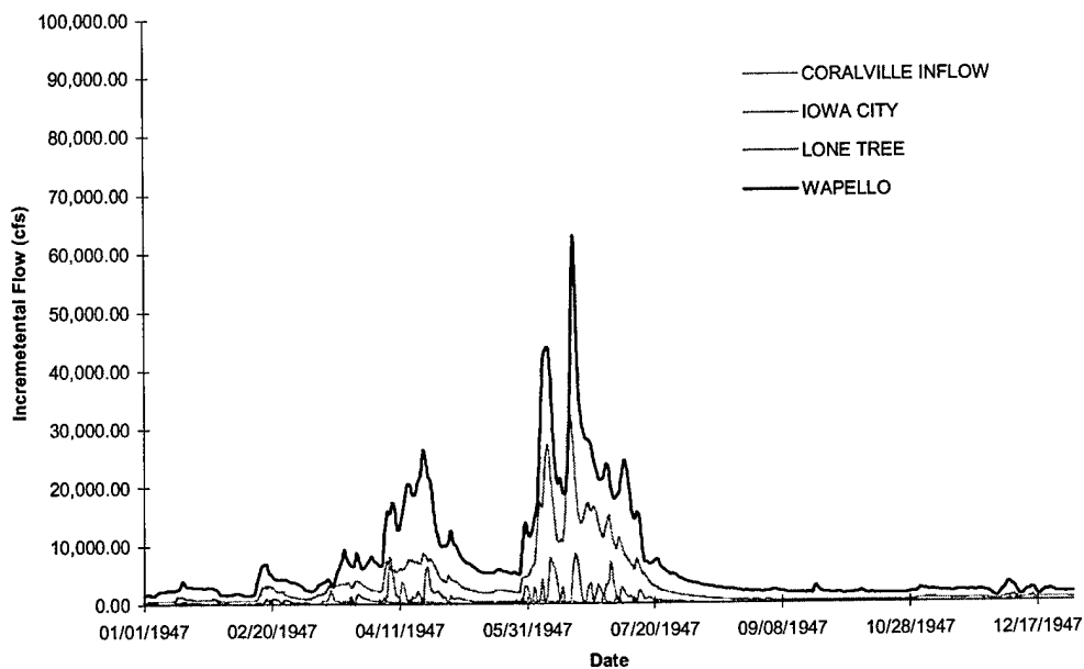
FIGURE C-3 Iowa River Incremental Inflows - Flood of 1947
