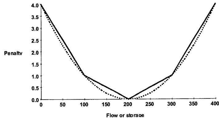
Figure 1. Linear approximation of nonlinear function
