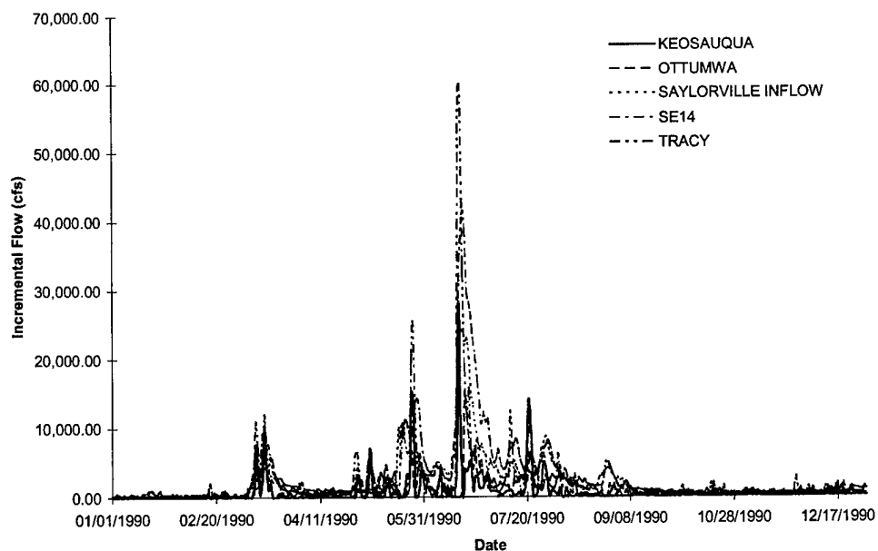
FIGURE C-16 Des Moines River Incremental Inflows - Flood of 1990
