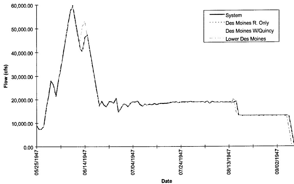
FIGURE E-2k. Hydrograph of Model Results at Tracy - Flood of 1947
