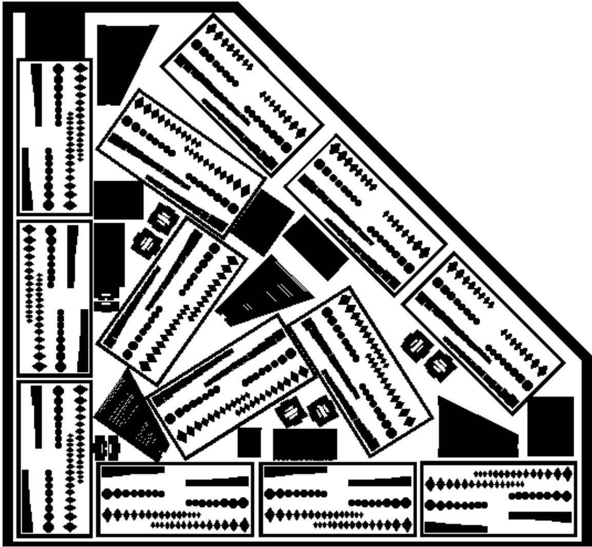
Figure 4.8 Image of an array of structures used to study crystal plane selectivity for GaAs etched with citric acid: \text{K}_3\text{C}_7\text{H}_5\text{O}_2:\text{H}_2\text{O}_2 . The structural layer was mechanically removed from the top to show this behavior in the sacrificial layer.
