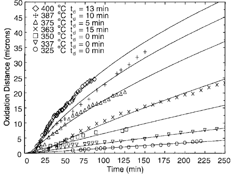
Figure 2.15 Graphical illustration of the effects of time and temperature on oxidation progress [14].
