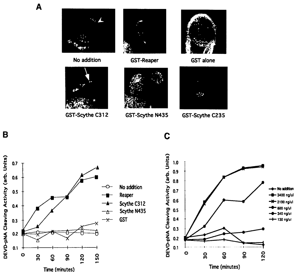
Fig. 2. ScytheC312 induces morphological characteristics of apoptosis and DEVDase activation. The indicated GST fusion proteins (final concentration 600 ng/ \mu l) or an equivalent amount of GST protein alone were added to Xenopus egg extract in the presence of sperm chromatin to form synthetic nuclei in the extracts (1000 nuclei/ \mu l) and an ATP regeneration system. (A) Photomicrographs of representative nuclei upon staining with the DNA intercalating dye, Hoescht 33258, 90 min after protein addition: dotted arrow = uncondensed interphase chromatin contained within an intact nuclear envelope, solid arrow = condensed, apoptotically fragmented chromatin, * = background staining of membranes present in the extract. (B) At the indicated times, 2 \mu l of extract were collected for a DEVD-pNA cleavage assay. (C) The indicated amounts of ScytheC312 were added to extracts and, at the indicated times, 2 \mu l of extract were collected for a DEVD-pNA cleavage assay.
