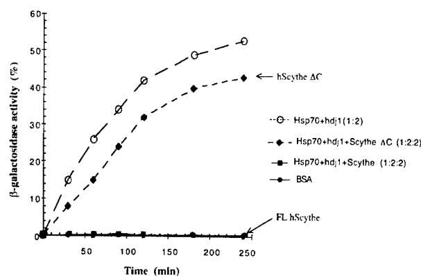
Fig. 3. Scythe functions as a negative regulator of Hsp70 chaperone activity. The inhibitory effect of full-length human Scythe (FL hScythe, 3.2 \mu M) and a truncated Scythe mutant lacking the 'BAG' domain (Scythe \Delta C, 3.2 \mu M) on Hsp70-dependent refolding was examined by the percentage recovered activity of unfolded \beta -galactosidase (3.2 nM) diluted into a refolding buffer containing ATP (1 mM), Hsp70 (1.6 \mu M) and Hdj-1 (3.2 \mu M). As a control for spontaneous refolding, denatured \beta -galactosidase (3.2 nM) was diluted into refolding buffer containing 3.2 \mu M bovine serum albumin (BSA).
