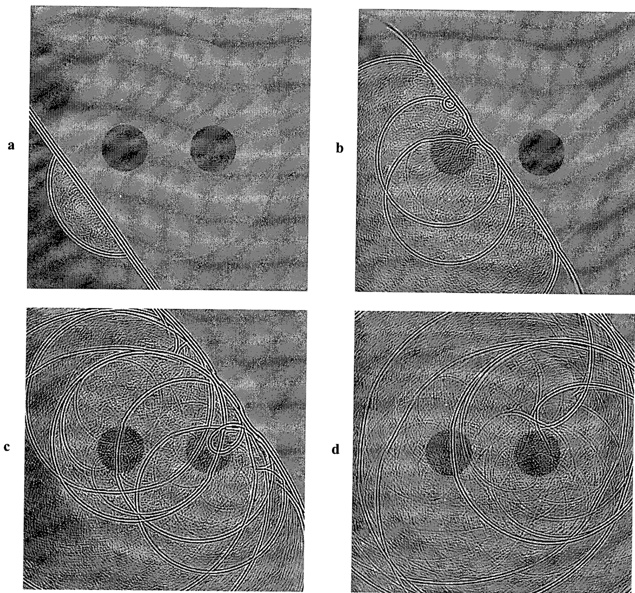
Figure 8: Computed pressure fields for a 48 mm diameter tissue-mimicking phantom. Panels (a)–(d) show the total acoustic pressure at intervals of 12 \mu s, superimposed on an image of the phantom. The area shown in each panel is 61 mm \times 61 mm. Wavefields are plotted using a bipolar logarithmic scale with a dynamic range of 60 dB.
