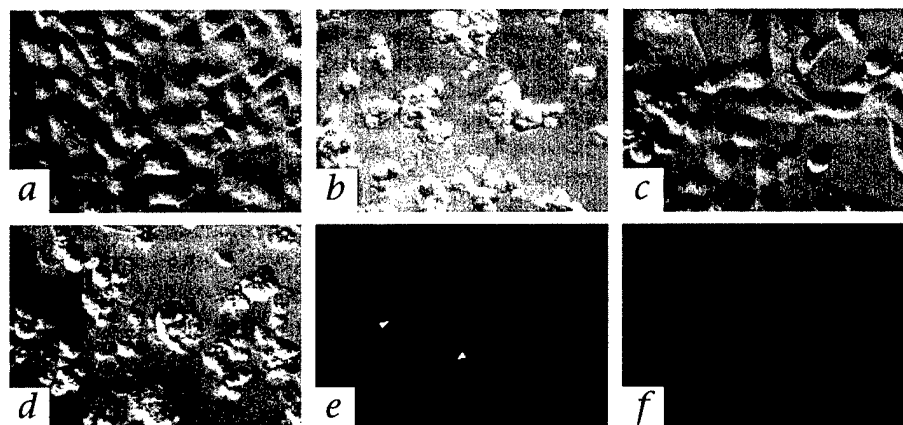
Fig. 3 CNGRC-GG-D(KLAKLAK)_2 and (RGD-4C)-GG-D(KLAKLAK)_2 induce apoptosis. a , KS1767 cells treated with 100 \mu M of non-targeted CARAC-GG-D(KLAKLAK)_2 (negative control) remain unaffected after 48 h. b , KS1767 cells treated with 100 \mu M of CNGRC-GG-D(KLAKLAK)_2 undergo apoptosis, as shown at 48 h. Condensed nuclei and plasma membrane blebbing are evident. c , KS1767 cells treated with 10 \mu M of an equimolar mixture of (RGD-4C) and D(KLAKLAK)_2 (negative control) remain unaffected after 48 h. d , KS1767 cells treated with 10 \mu M of (RGD-4C)-GG-D(KLAKLAK)_2 undergo apoptosis, as shown at 48 h. Condensed nuclei and plasma membrane blebbing are evident. Scale bar represents 250 \mu m. e and f , KS1767 cells treated with 100 \mu M of CNGRC -biotin ( e ) or CARAC -biotin ( f ) for 24 h and subsequently
