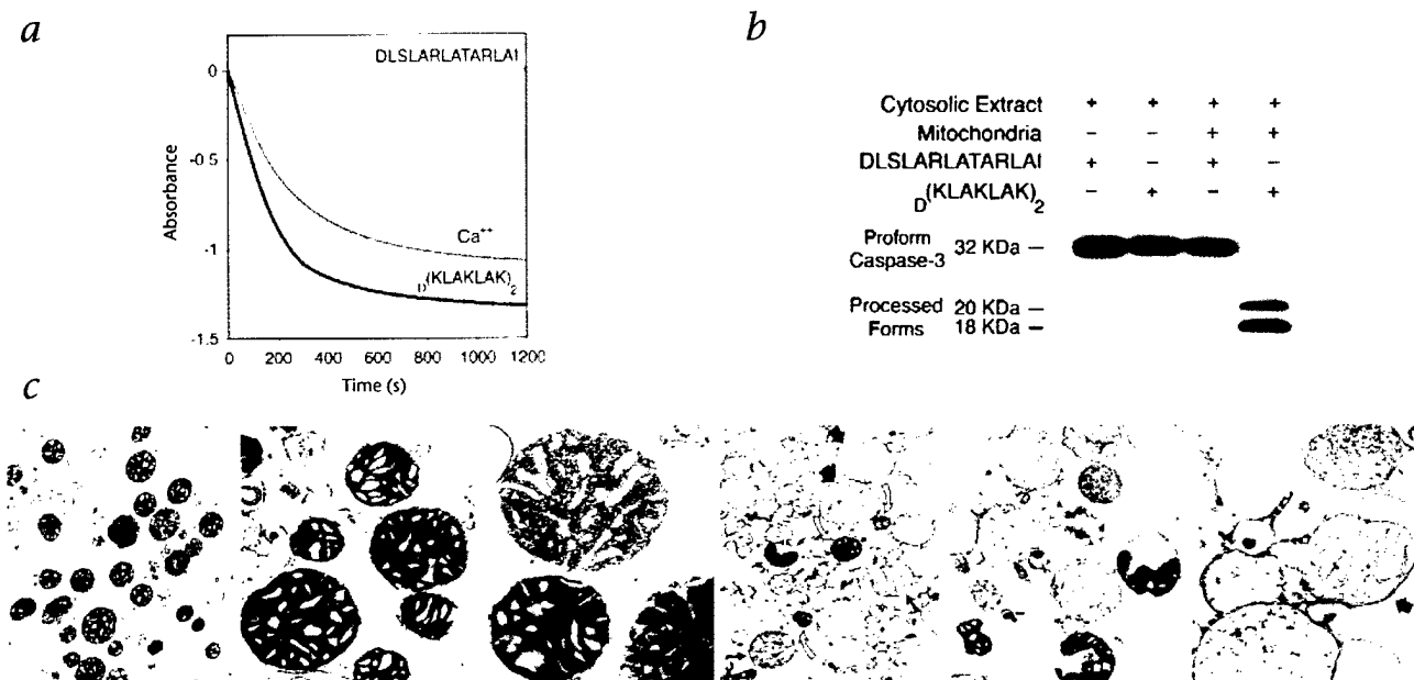
Fig. 2 D(KLAKLAK)_2 disrupts mitochondrial membranes. a , D(KLAKLAK)_2 or Ca^{2+} (positive control) induced mitochondrial swelling, whereas the non- \alpha -helix-former D(LSLARL) (negative control) did not, as shown by mitochondrial swelling curves (optical absorbance spectrum). b , D(KLAKLAK)_2 activates cell-free apoptosis in a system composed of normal mitochondria and cytosolic extract, but D(LSLARL) does not. An immunoblot of caspase-3 cleavage from pro-form (32-kDa) to processed forms (18- and 20-kDa) demonstrates a mitochondria-dependent cell-free apoptosis (left margin, sizes). Results were reproduced in two independent experiments. c , Morphologic alterations in isolated mito-
