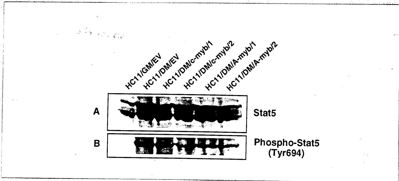
FIG. 4. Expression and activation of Stat5 in HC11 cells with deregulated expression of A-myb and c-myb during proliferation and differentiation. HC11 were induced to differentiate as follows: cells were grown to confluence and maintained in complete growth medium (GM), after which epidermal growth factor (EGF) was withdrawn and cells switched to priming medium containing hydrocortisone (HC) for 1 day and then to induction medium containing HC + prolactin (PRL) for 3 days. (A) Western blot analysis of Stat5 protein in mock-transfected HC11 cells in GM (HC11/GM/EV) and DM (HC11/DM/EV), c-myb transfected cells (HC11/DM/ c-myb /1 and HC11/DM/ c-myb /2) and A-myb transfected cells (HC11/DM/ A-myb /1 and HC11/DM/ A-myb /2). The primary antibody (which binds to both Stat5a and Stat5b) and the procedure are described in materials and methods. (B) Activation of Stat5 by tyrosine phosphorylation in different HC11 cells described in panel a. The blot was stripped and reprobed with primary antibody specific to Stat5 phosphorylated at Tyr 694.
