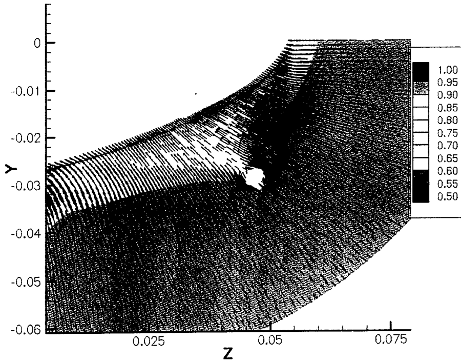
Fig. 24 Secondary velocity vectors at the outboard propeller plane.
