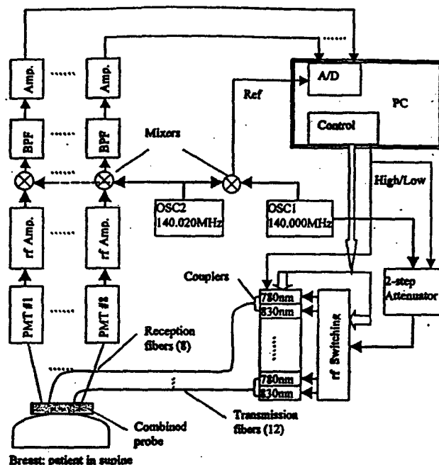
Fig. 3. Schematic of the NIR frequency-domain imaging system. The modulation frequency is 140 MHz. The 12 dual-wavelength source channels are switched on sequentially by a PC, and 8 detector channels receive signals in parallel. BPF, bandpass filter; OSC, oscillator.
