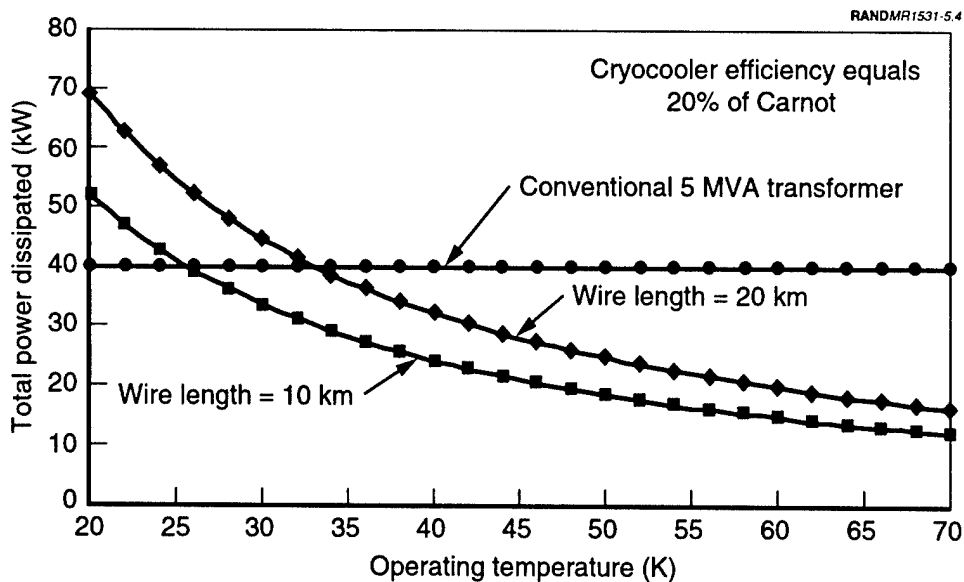
Figure 5.4—Dependence on the Operating Temperature of the Total Power Dissipated by a 5 MVA HTS Transformer
