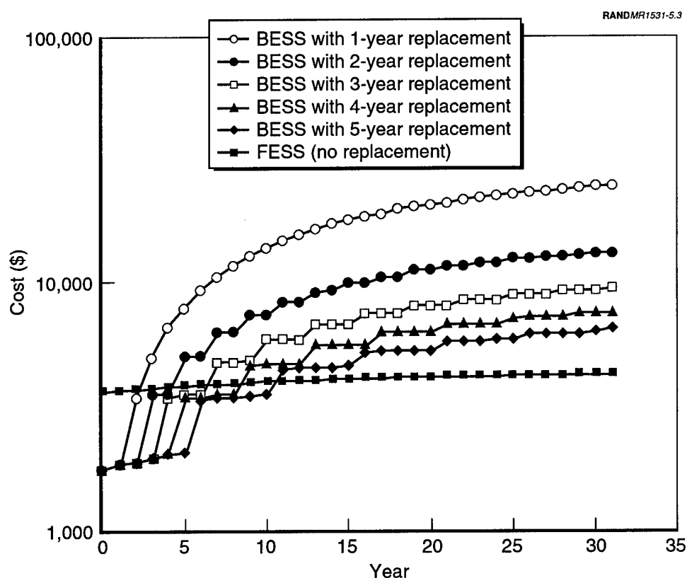
Figure 5.3—Effects of Replacement Schedule on Life-Cycle Costs for BESSs and a FESS
