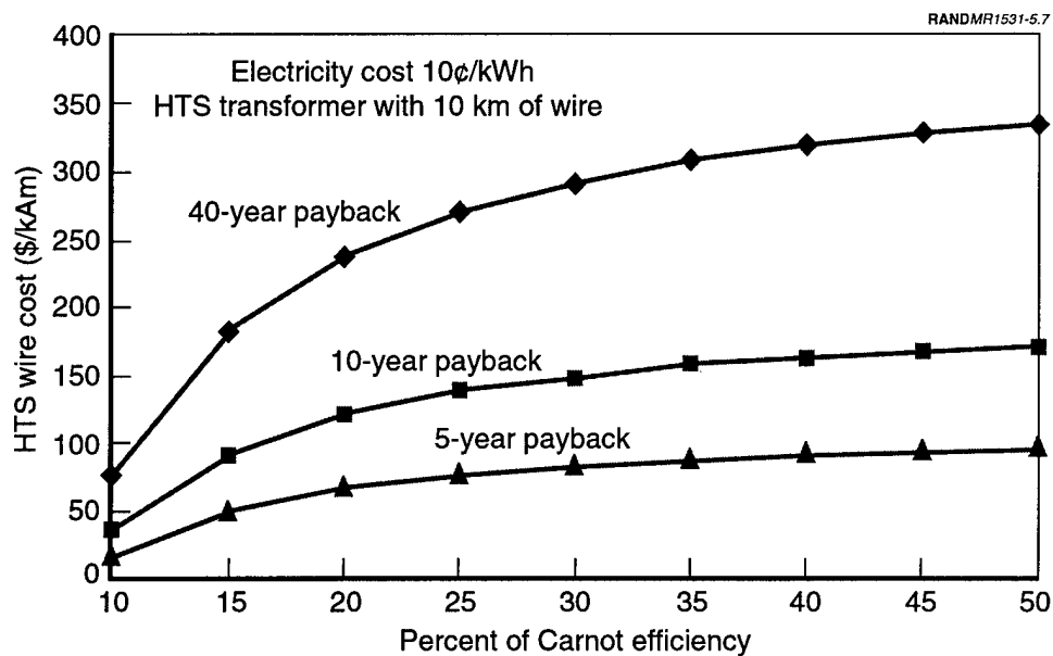
Figure 5.7—Discounted Payback Time for a 5 MVA HTS Transformer Compared with a Conventional Transformer as a Function of HTS Wire Cost and Cryocooler Efficiency, Electricity Cost of 10¢ per kWh
