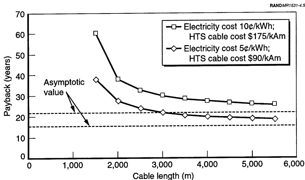
Figure 4.5—Discounted Payback Time Versus Cable Length for HTS Cable Compared with XLPE Cable, Cryocooler Efficiency 27 Percent of Carnot
