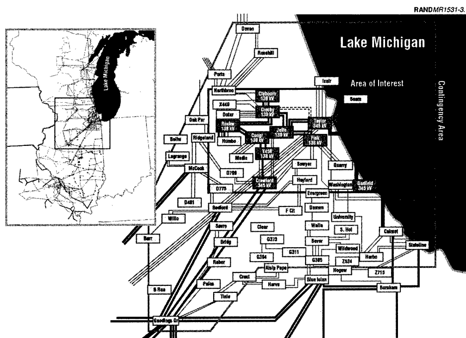
Figure 3.1—Portion of Downtown Chicago Grid Showing Area of Interest and Contingency Area, Commonwealth Edison Control Area Within MAIN Transmission Grid Shown in Inset
