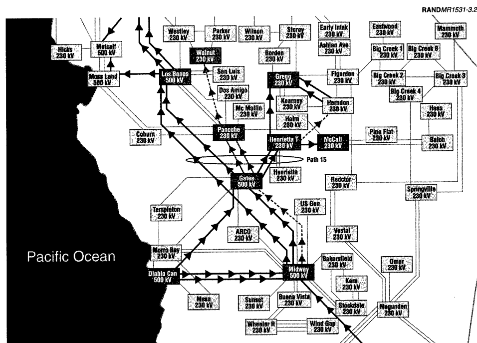
Figure 3.2—Portion of the California Grid Showing Path 15
