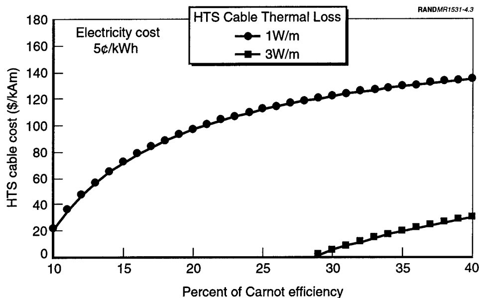
Figure 4.3—Boundaries Showing that HTS Cables with Cable Cost and Cryocooler Efficiency Values Below the Curves Have a Lower Life-Cycle Cost Per Unit of Power Delivered than the XLPE Cable, Electricity Cost of 5¢ per kWh
