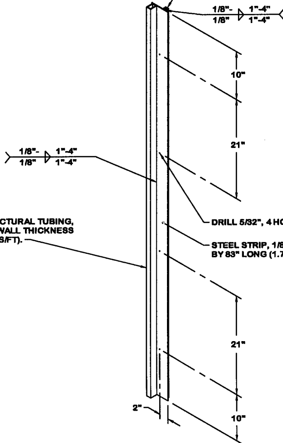
VIEW A
