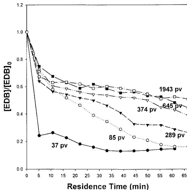
Fig. 7. Ethylene dibromide (EDB) concentration profile through the pilot plant. V = 600 mL/min. The concentrations at each sample point increase over time (from 37 to 1943 pore volumes) until steady state conditions are reached. Once steady state is reached the profile is stable for hundreds of pore volumes, 645-1943 pore volumes. The initial rapid drop is due to nonequilibrium mass transfer. The removal of EDB from canisters 2-12 is dominated by the rate of the surface reaction.
