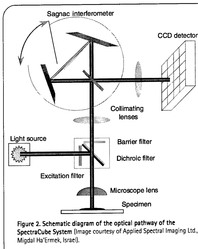
Figure 2. Schematic diagram of the optical pathway of the SpectraCube System (Image courtesy of Applied Spectral Imaging Ltd., Migdal Ha'Ermek, Israel).
