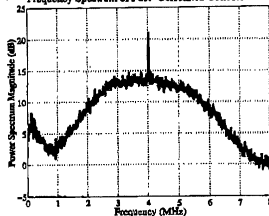
Frequency Spectrum of Post-Correlated Collected Data
