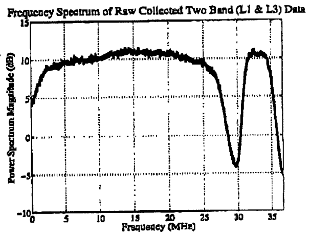
Figure 18. Frequency Domain Representation of the Collected Dual Band Data
