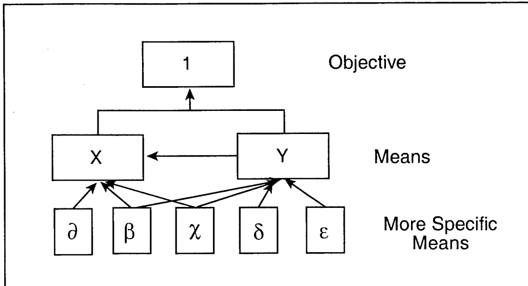
Figure 3. Means-Objective Network
