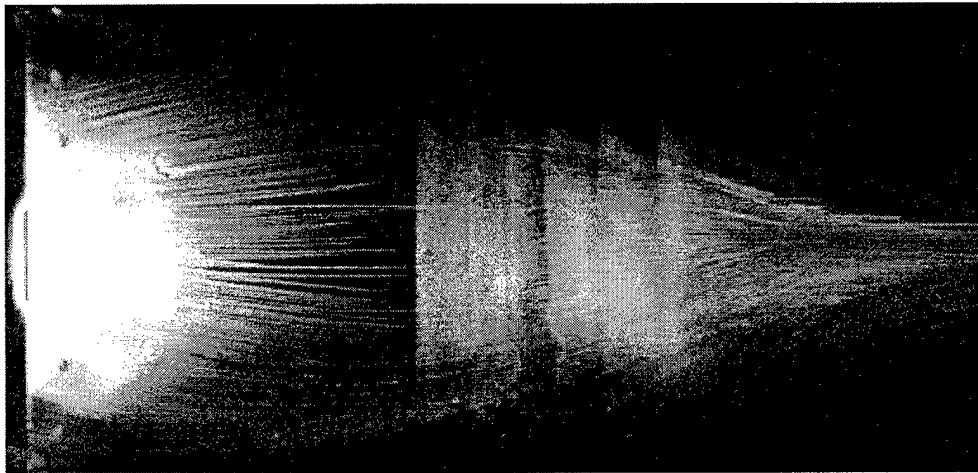
Figure 4: Surface flow visualization with helium injection, conditions similar to Condition 1, with J = 0.09 . The flow is from the left to the right. The slot is visible at the far left.
